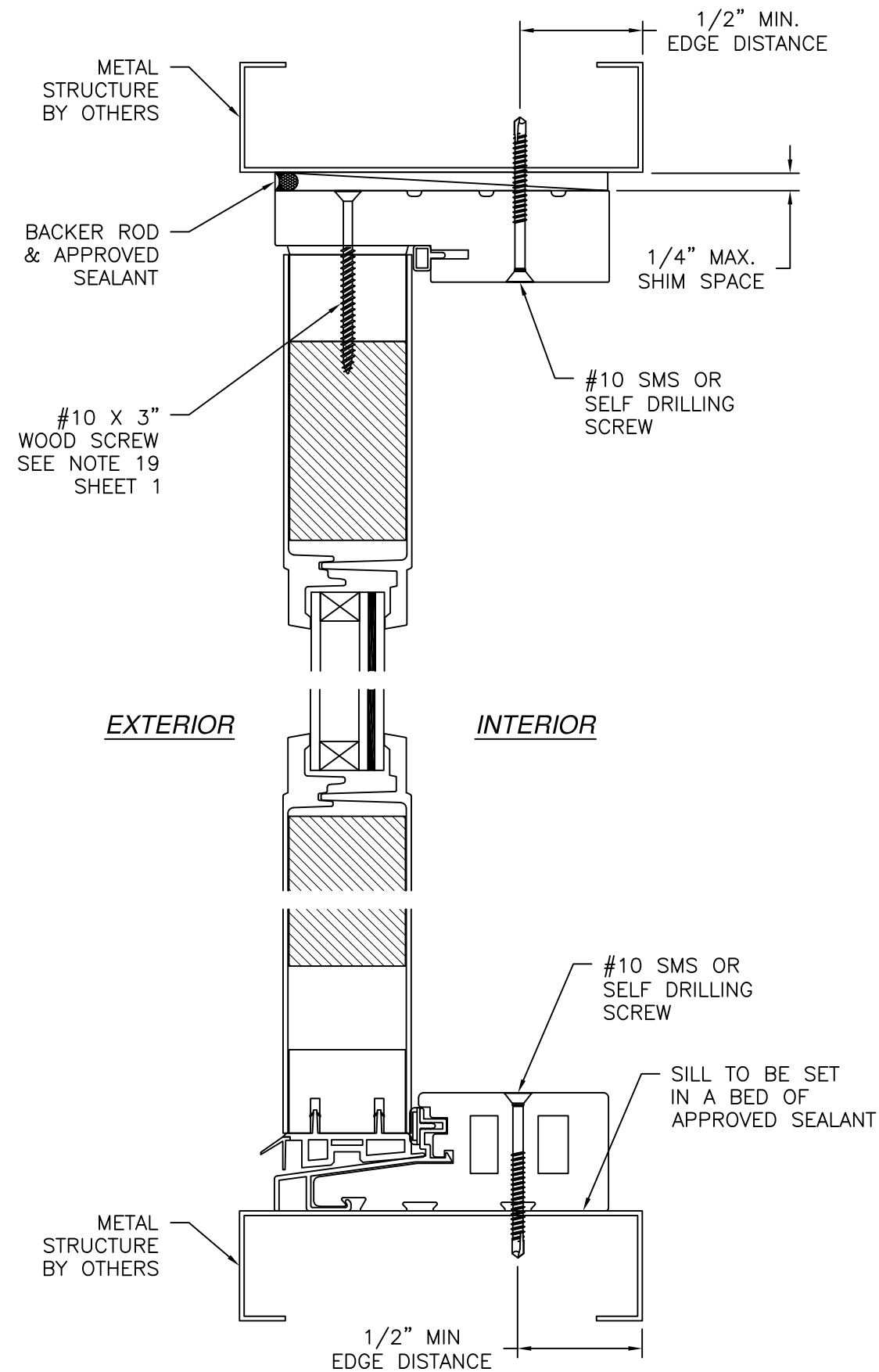
SIDELITE DOOR INSTALLATION DETAIL METAL STRUCTURE INSTALLATION STANDARD FRAME SHOWN, SOFT PVC FRAME SIMILAR FULL LITE SHOWN. 3/4 & 1/2 LITE SIMILAR
