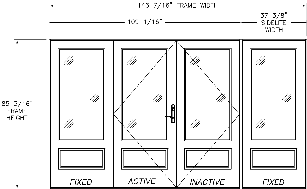
SLPS PATIO DOOR LITE OUTSWING (OXX/O) 7' UNIT EXTERIOR VIEW 3/4 LITE PANELS REFER TO SHEET 5 FOR HARDWARE AND NOTES
