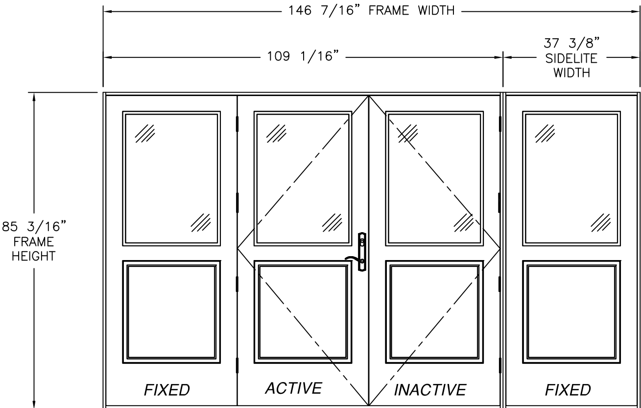
SLPS PATIO DOOR LITE OUTSWING (OXX/O) 7' UNIT EXTERIOR VIEW 1/2 LITE PANELS REFER TO SHEET 5 FOR HARDWARE AND NOTES
