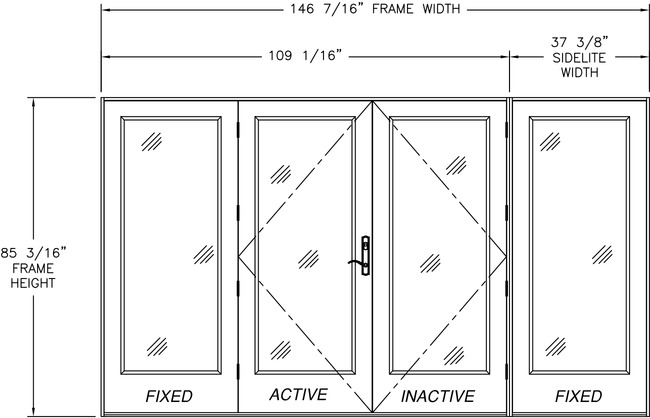
SLPS PATIO DOOR LITE OUTSWING (OXX/O) 7' UNIT EXTERIOR VIEW FULL LITE PANELS REFER TO SHEET 5 FOR HARDWARE AND NOTES
