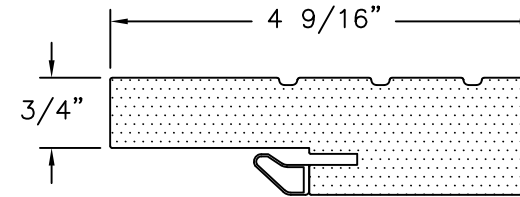
FRAME SOFT PVC FOAM PVC CO-EX
