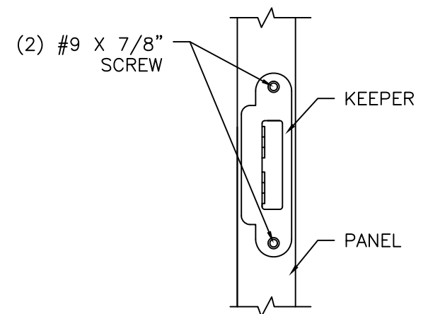
SLAB MULTI-POINT LOCK KEEPER DETAIL
