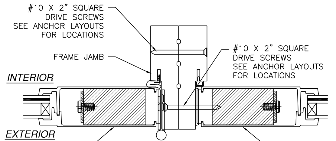
MULLION DETAIL
