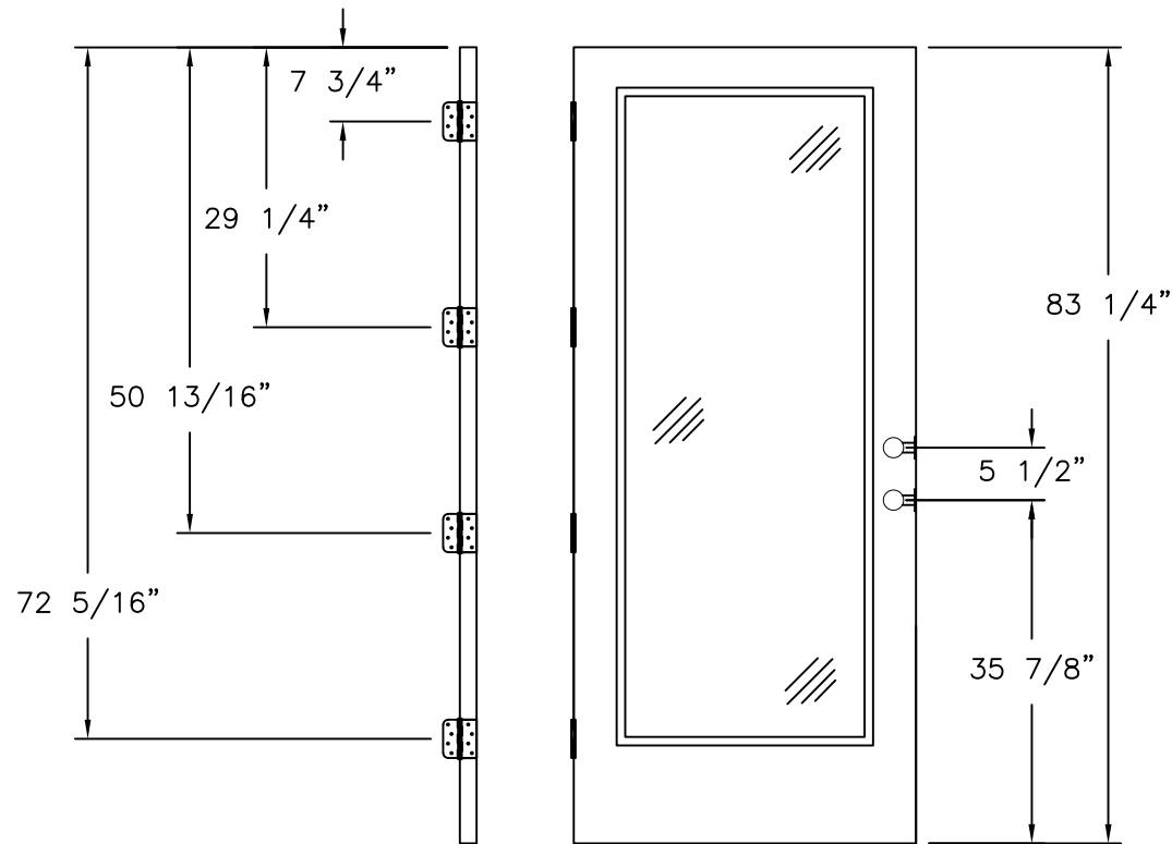
LOCK AND HINGES LOCATIONS 7' UNIT, WITH LATCH AND DEADBOLT, FULL LITE AND 3/4 LITE PANELS
