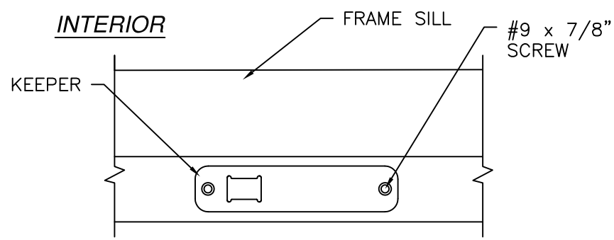
SILL KEEPER DETAIL
