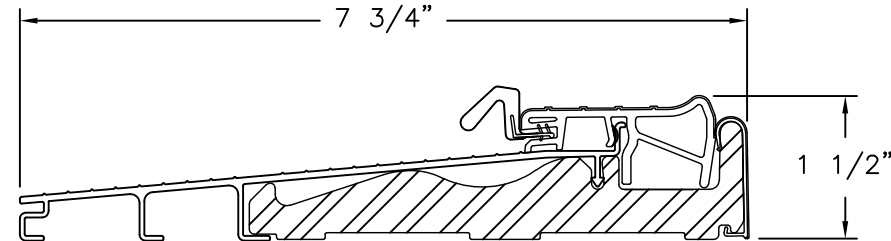
ENDURA THRESHOLD ZOB4565 ALTERNATE
