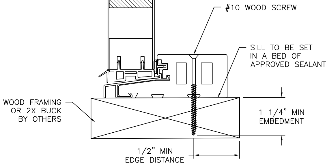
SIDELITE DOOR INSTALLATION DETAIL 2X BUCK/WOOD FRAMING STANDARD FRAME SHOWN, SOFT PVC FRAME SIMILAR FULL LITE SHOWN. 3/4 & 1/2 LITE SIMILAR
