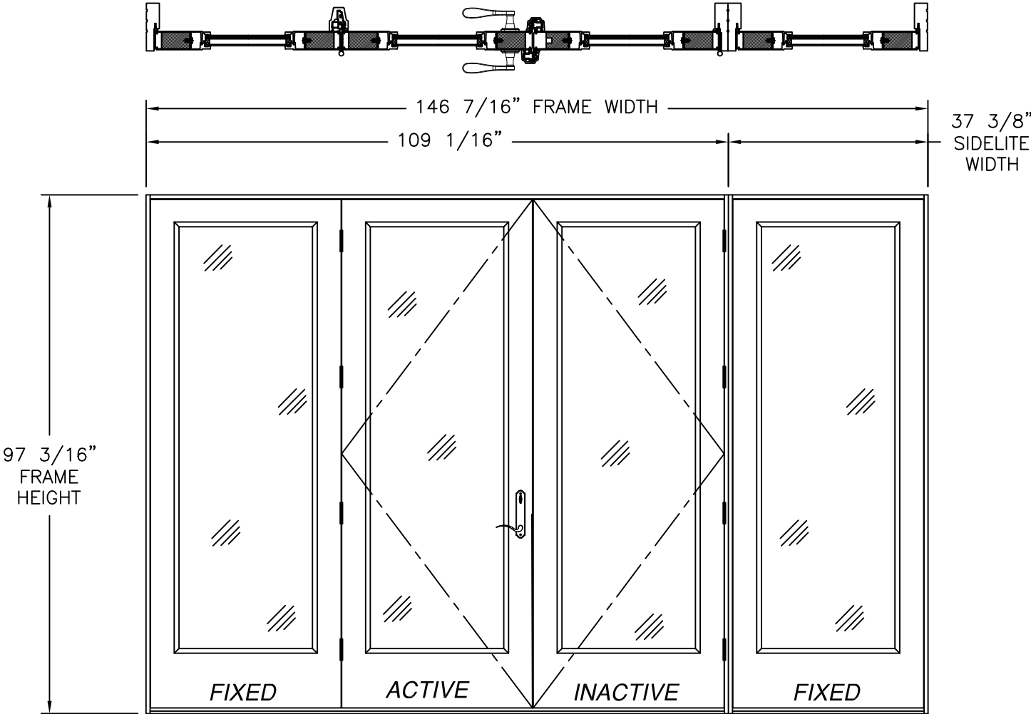
SLPS PATIO DOOR LITE OUTSWING (OXX/O) 8' UNIT EXTERIOR VIEW FULL LITE PANELS REFER TO SHEET 5 FOR HARDWARE AND NOTES
