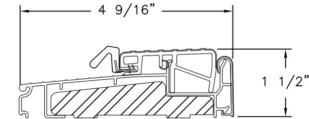
ENDURA THRESHOLD ZOB4565 ALTERNATE
