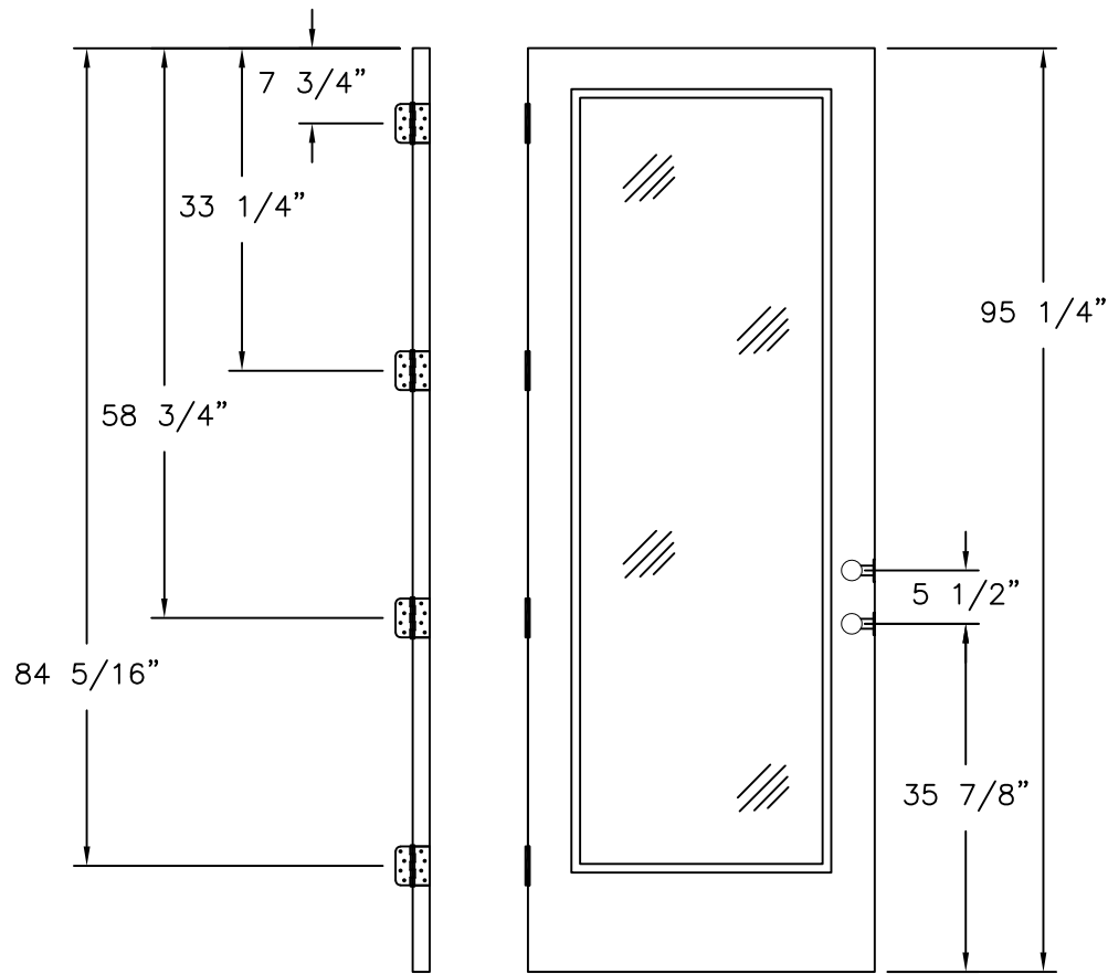
LOCK AND HINGES LOCATIONS 8' UNIT, WITH LATCH AND DEADBOLT, FULL LITE AND 3/4 LITE PANELS
