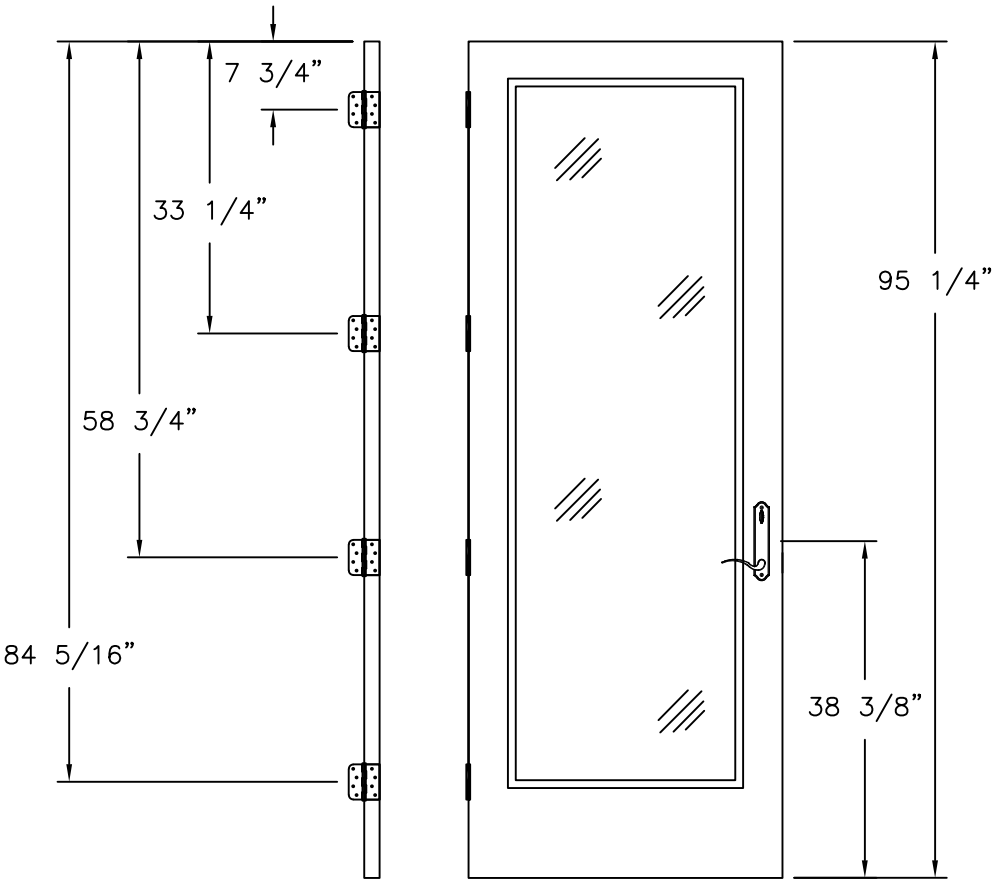
LOCK AND HINGES LOCATIONS 8' UNIT, WITH HANDLE, FULL LITE, 3/4 AND 1/2 LITE PANELS
