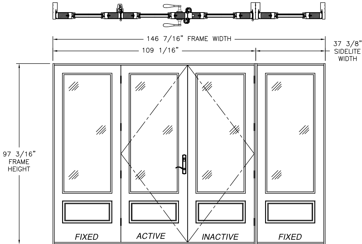
SLPS PATIO DOOR LITE OUTSWING (OXX/O) 8' UNIT EXTERIOR VIEW 3/4 LITE PANELS REFER TO SHEET 5 FOR HARDWARE AND NOTES
