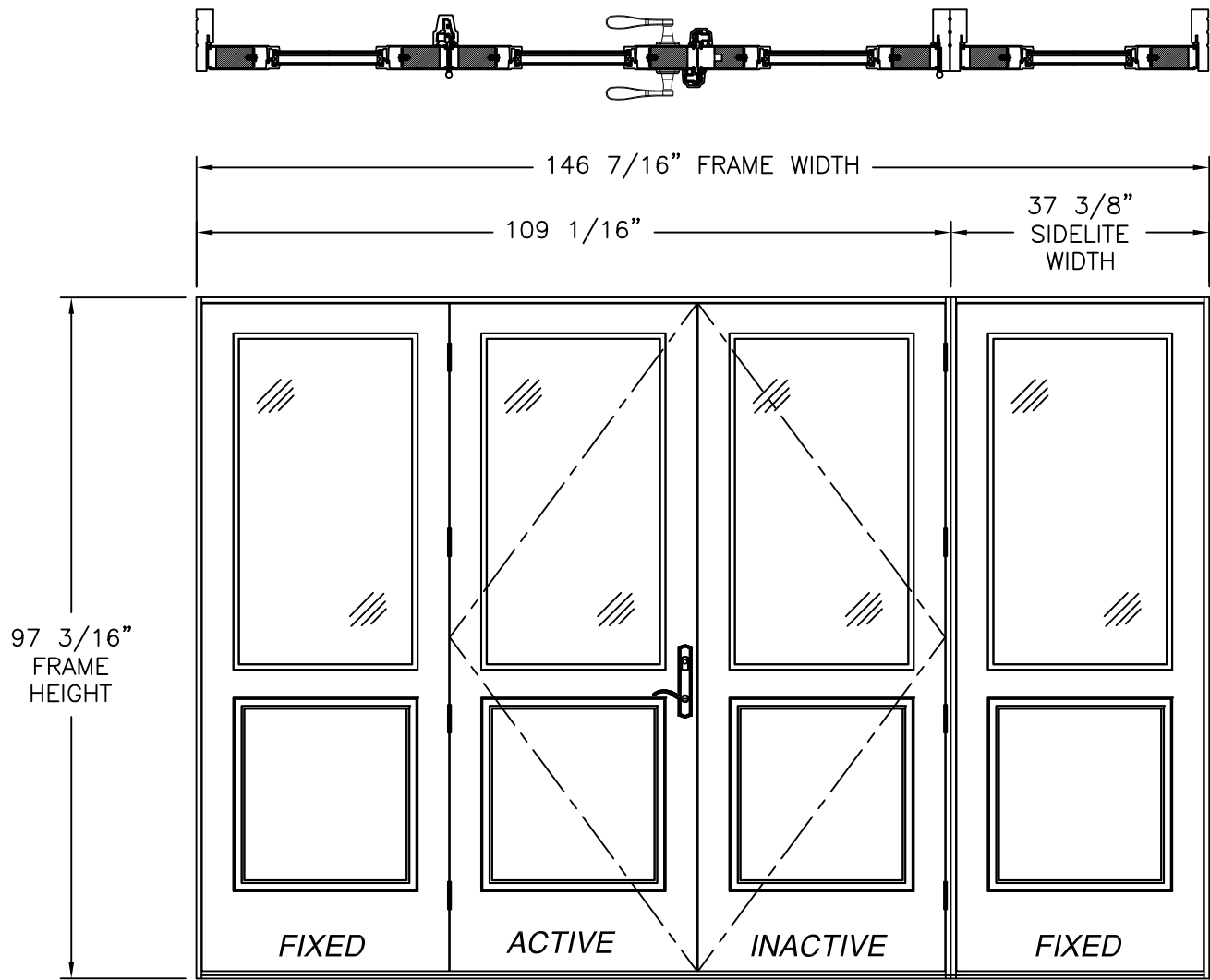
SLPS PATIO DOOR LITE OUTSWING (OXX/O) 8' UNIT EXTERIOR VIEW 1/2 LITE PANELS REFER TO SHEET 5 FOR HARDWARE AND NOTES
