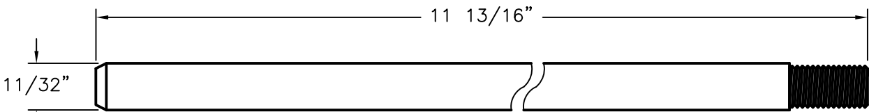
FLUSH BOLT BAR STAINLESS STEEL (SS93B)
