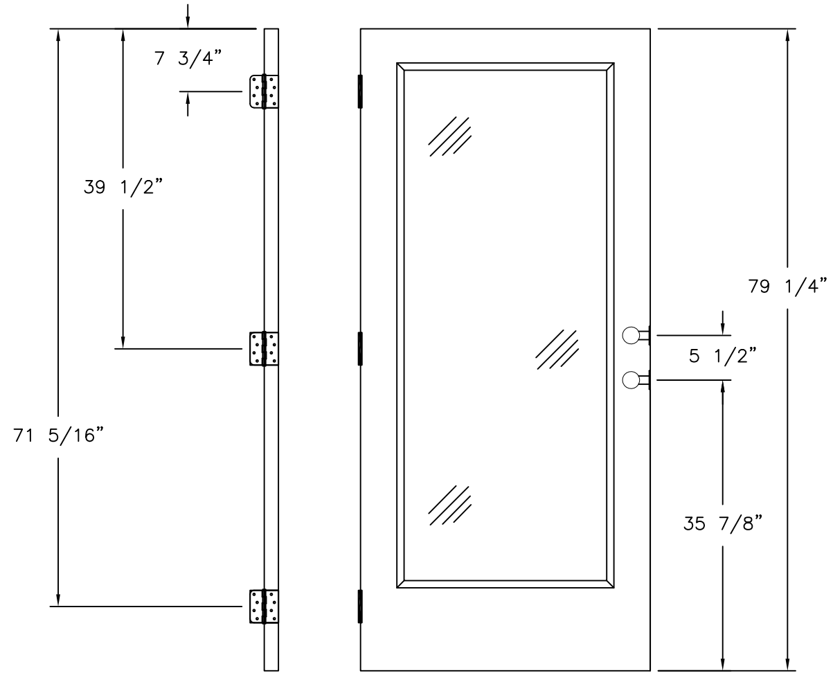
LOCK AND HINGES LOCATIONS WITH LATCH AND DEADBOLT FULL LITE PANEL, 3/4 AND 1/2 PANELS
