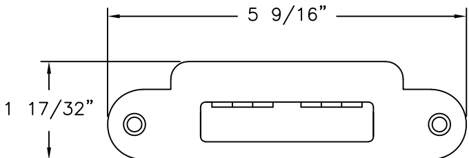
SLAB MULTI-POINT LOCK KEEPER STEEL
