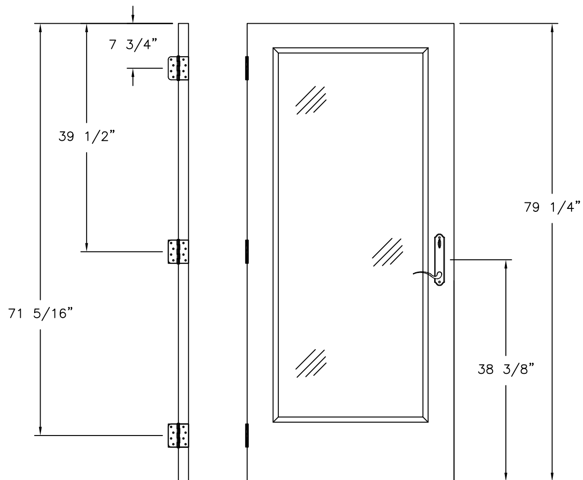
LOCK AND HINGES LOCATIONS WITH HANDLE FULL LITE PANEL, 3/4 AND 1/2 LITE PANELS
