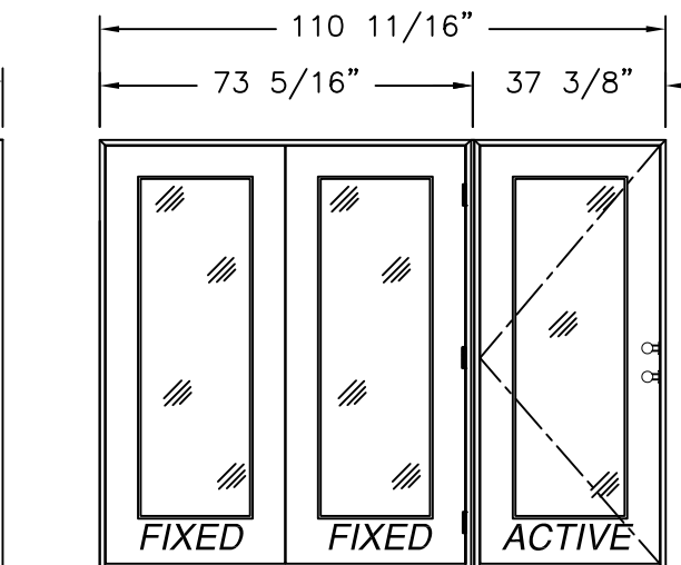
SINGLE W/SIDELITES MULL. (OO/X) EXTERIOR VIEW FULL LITE SHOWN, 3/4 & 1/2 LITE SIMILAR
