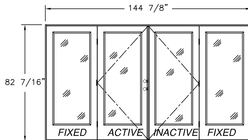
DOUBLE W/SIDELITE (OXXO) EXTERIOR VIEW FULL LITE SHOWN, 3/4 & 1/2 LITE SIMILAR
