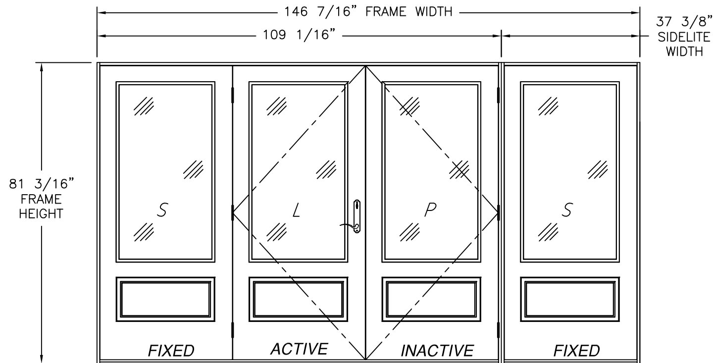
SLPS PATIO DOOR LITE 6'11" OUT-SWING (OXX/O) EXTERIOR VIEW, 3/4 LITE PANELS
