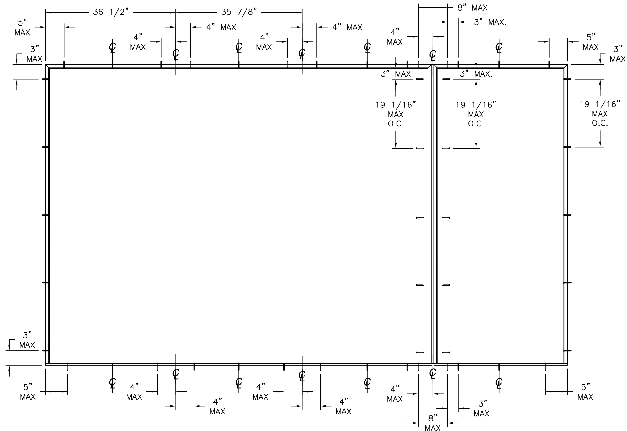
ANCHORING LAYOUT
