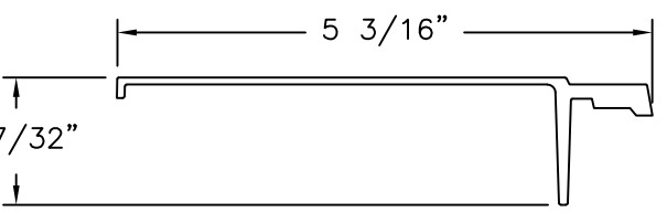
SHEET MOLDING COMPOUND SKIN-1 FIBERGLASS
