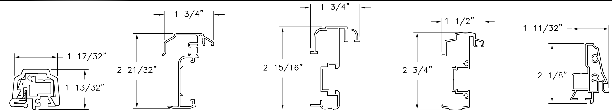
T-ASTRAGAL RIGID PVC ENDURA ULTIMATE PUSH BUTTON ASTRAGAL ALTERNATE DLP ASTRAGAL ALTERNATE COLUMBIA T-ASTRAGAL .060" THICKNESS, ALUMINUM 6063-T5 ALTERNATE REINFORCEMENT (B) ALUMINUM
