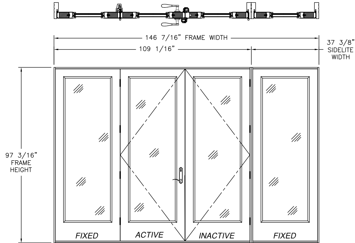
SLPS PATIO DOOR LITE OUTSWING (OXX/O) 8' UNIT EXTERIOR VIEW FULL LITE PANELS REFER TO SHEET 5 FOR HARDWARE AND NOTES
