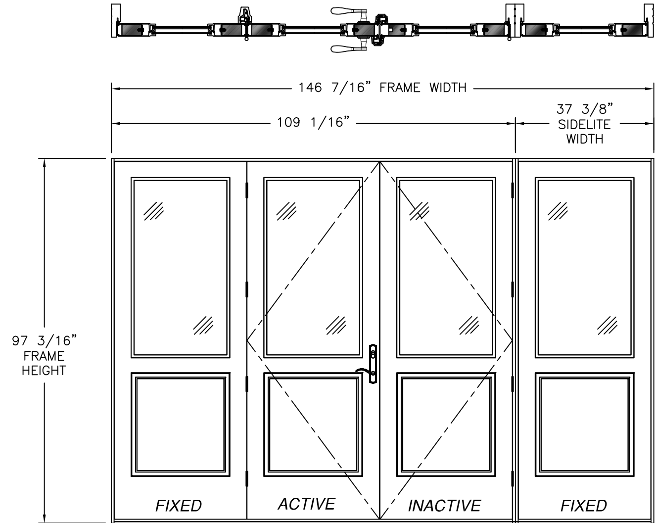
SLPS PATIO DOOR LITE OUTSWING (OXX/O) 8' UNIT EXTERIOR VIEW 1/2 LITE PANELS REFER TO SHEET 5 FOR HARDWARE AND NOTES
