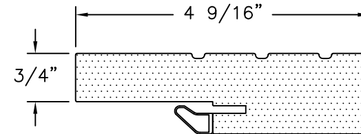
FRAME SOFT PVC FOAM PVC CO-EX
