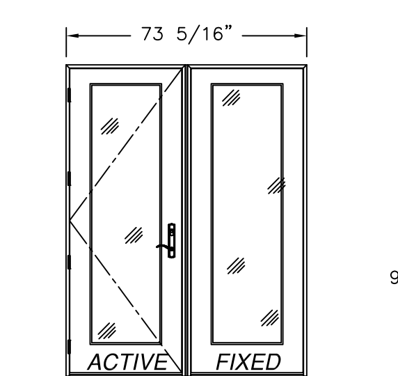
SINGLE W/SIDELITE MULL. (X/O, O/X) EXTERIOR VIEW FULL LITE SHOWN, 3/4 & 1/2 LITE SIMILAR
