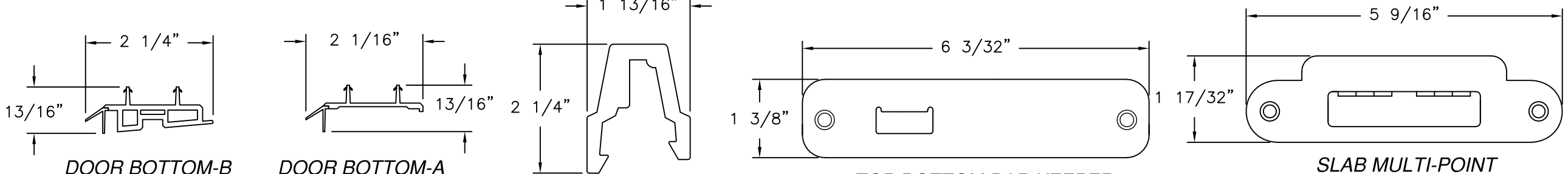
DOOR BOTTOM-B PVC CO-EX DOOR BOTTOM-A PVC CO-EX MULLION COVER (B) FOAM PVC TOP/BOTTOM BAR KEEPER STAINLESS STEEL (SS92H) SLAB MULTI-POINT LOCK KEEPER STEEL
