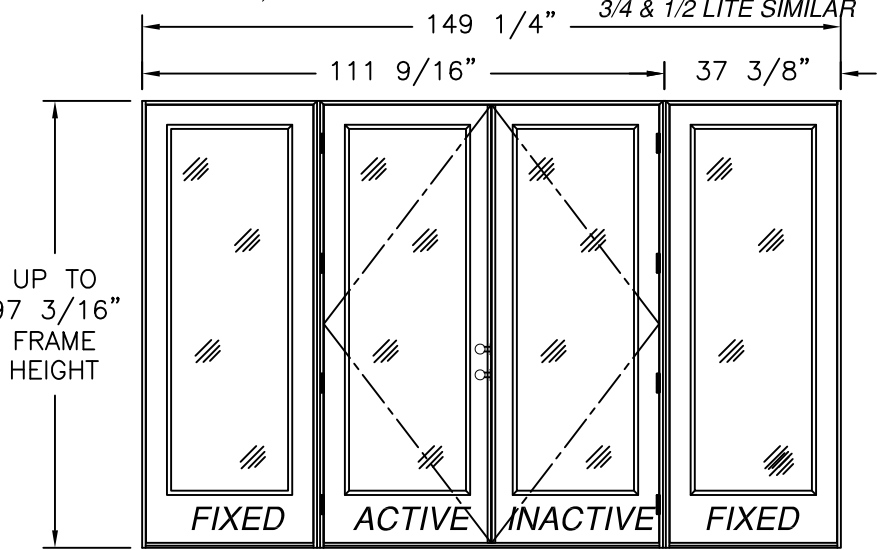
DOUBLE W/SIDELITES MULL. (O/XX/O) EXTERIOR VIEW FULL LITE SHOWN, 3/4 & 1/2 LITE SIMILAR
