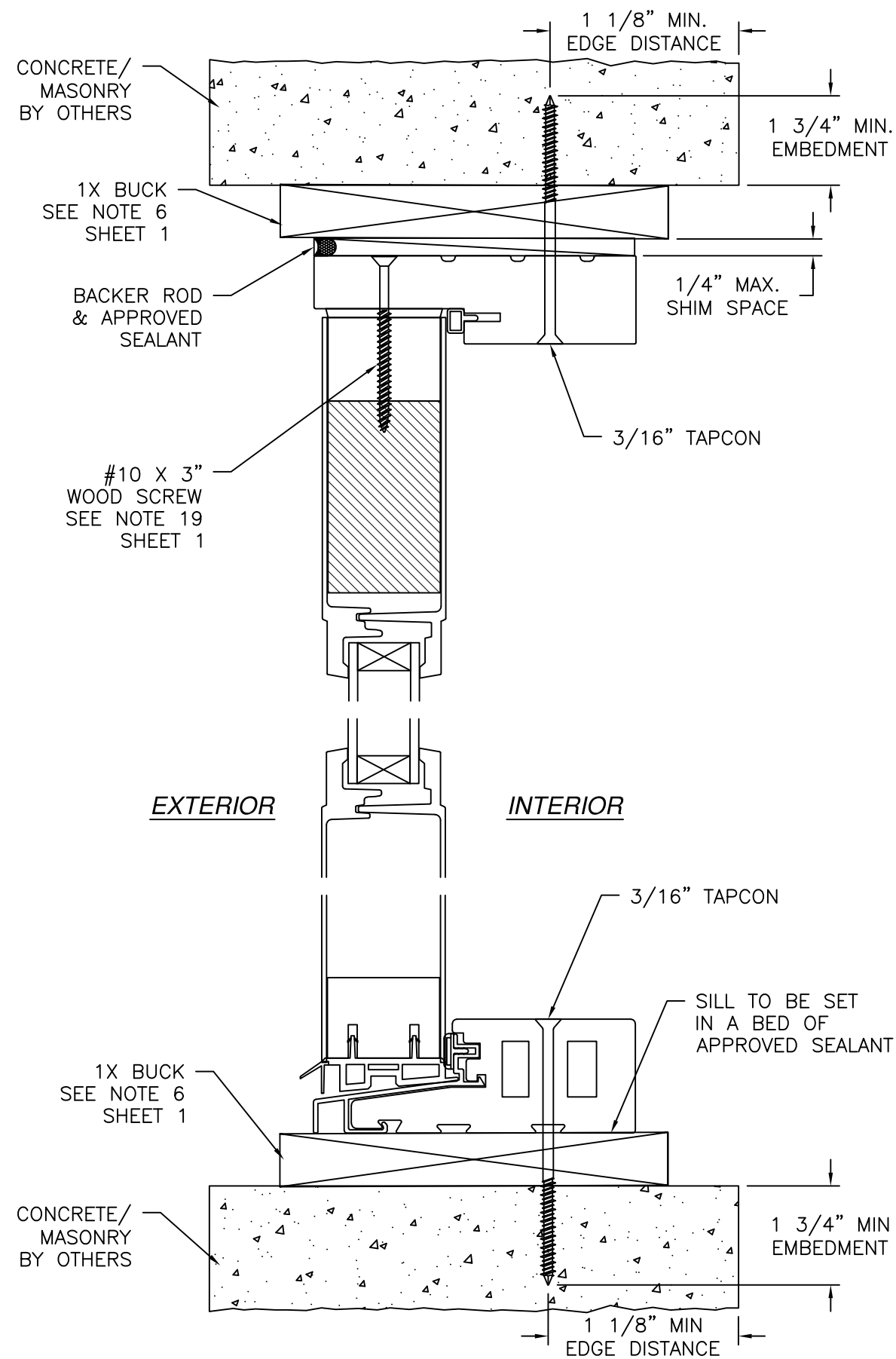
SIDELITE DOOR INSTALLATION DETAIL CONCRETE/MASONRY W/1X BUCK INSTALLATION FULL LITE SHOWN, 3/4 & 1/2 LITE SIMILAR
