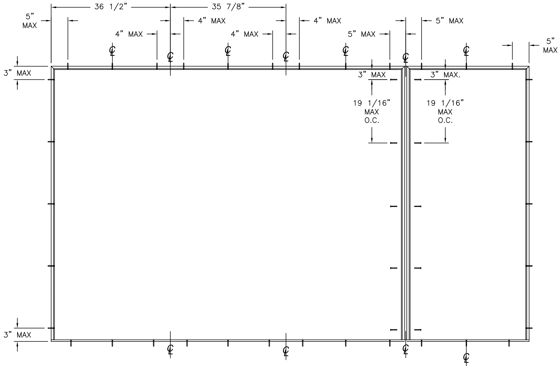
ANCHORING LAYOUT
