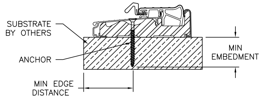
ENDURA THRESHOLD ZOBLH4565
