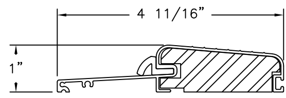
COLUMBIA THRESHOLD 575 ALTERNATE
