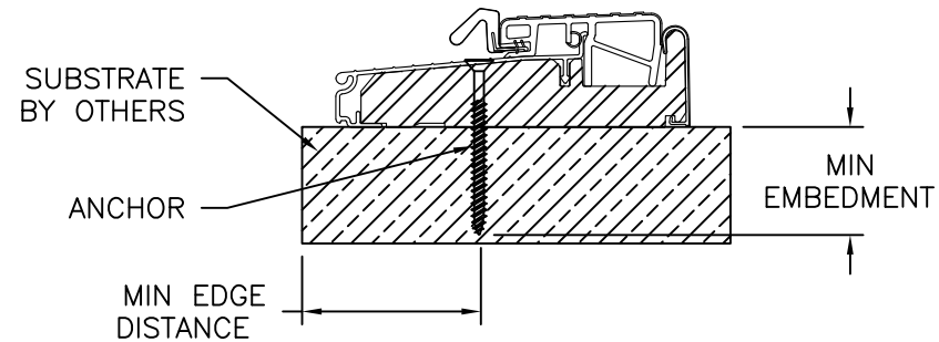
ENDURA THRESHOLD ZOB4565FN
