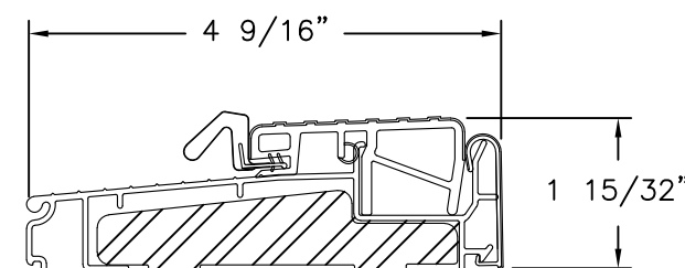
ENDURA THRESHOLD ZOBL4565 ALTERNATE
