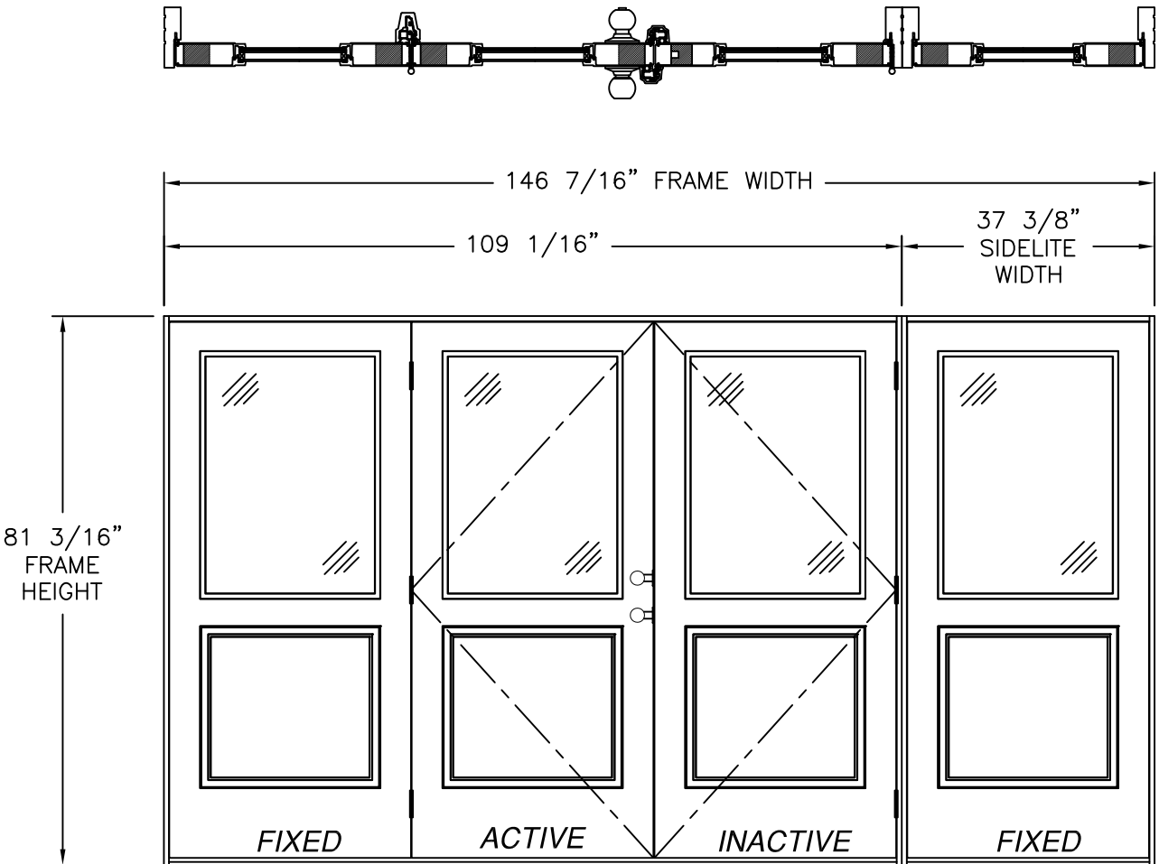
SERIES SLPS OUT-SWING SIDE-HINGED DOOR W/SIDELITES (OXX/O) EXTERIOR VIEW 1/2 LITE PANELS
