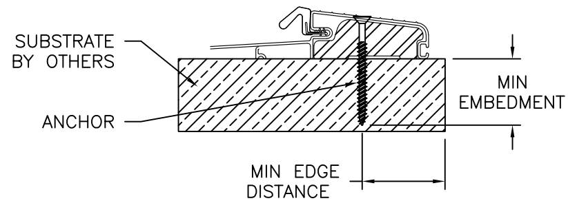
ENDURA THRESHOLD FOB4565
