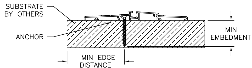
ENDURA ADA THRESHOLD ZHCO5622
