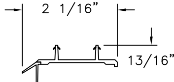
DOOR BOTTOM-A PVC CO-EX
