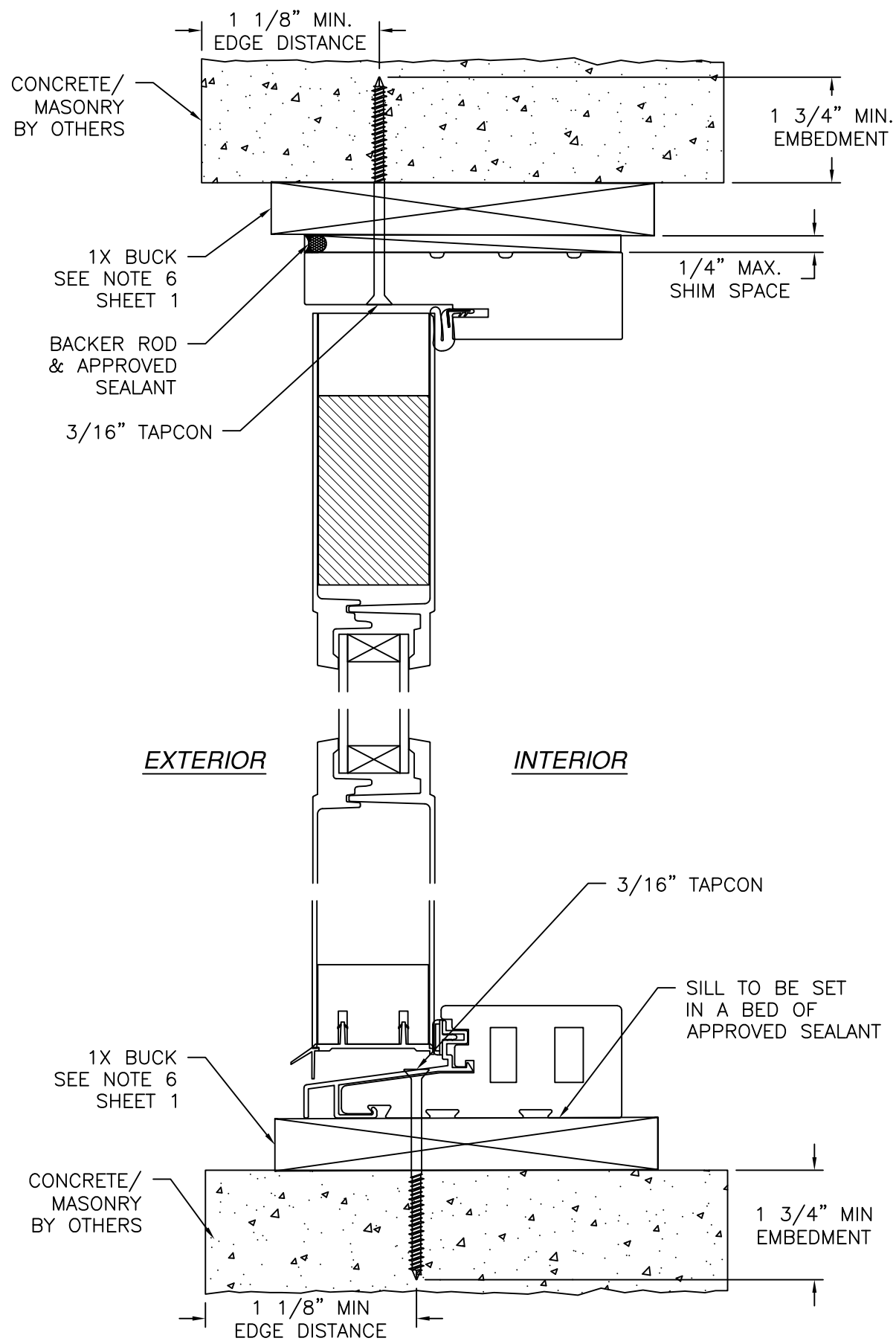
DOOR INSTALLATION DETAIL CONCRETE/MASONRY W/1X BUCK INSTALLATION FULL LITE SHOWN, 3/4 & 1/2 LITE SIMILAR
