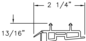
DOOR BOTTOM-B PVC CO-EX
