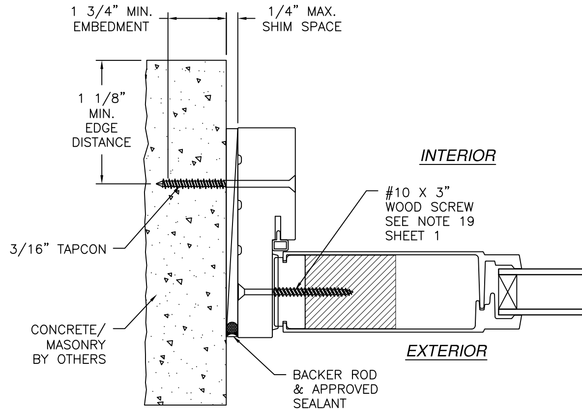
SIDELITE INSTALLATION DETAIL CONCRETE/MASONRY INSTALLATION
