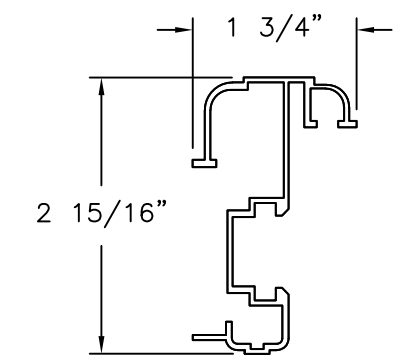
DLP ASTRAGAL ALTERNATE
