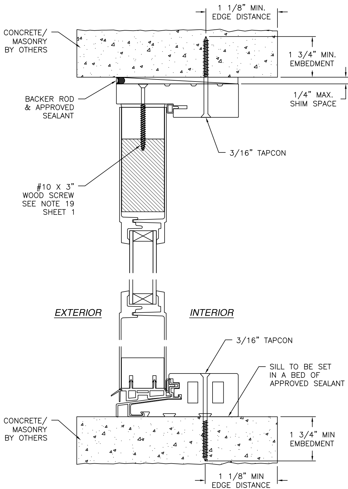
SIDELITE DOOR INSTALLATION DETAIL CONCRETE/MASONRY INSTALLATION FULL LITE SHOWN, 3/4 & 1/2 LITE SIMILAR
