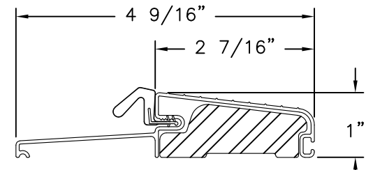
ENDURA THRESHOLD FOB4565 ALTERNATE
