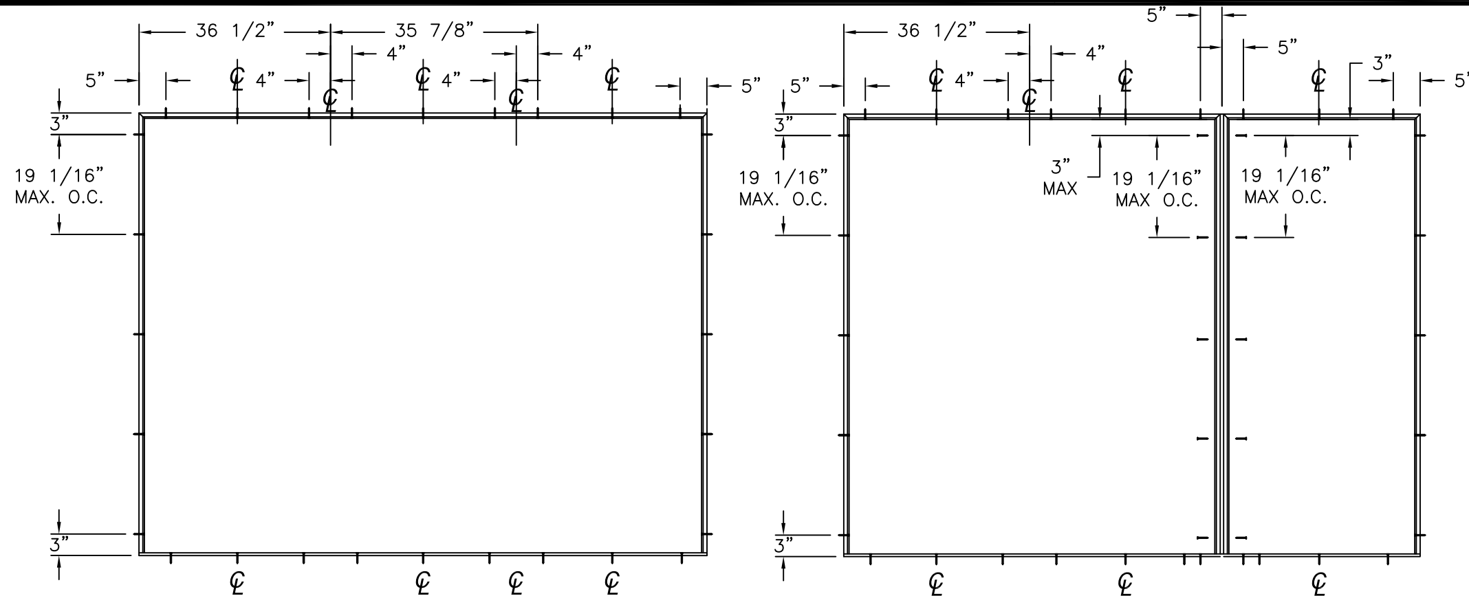
ANCHORING LAYOUT FOR OXO, XXO AND OXX
