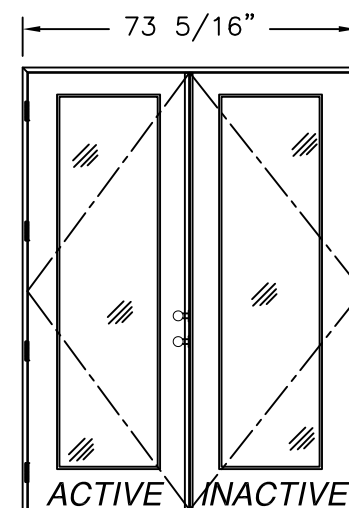
DOUBLE (XX) EXTERIOR VIEW
