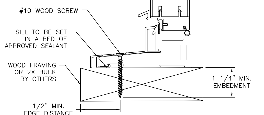
DOOR INSTALLATION DETAIL 2X BUCK/WOOD FRAMING INSTALLATION FULL LITE SHOWN, 3/4 & 1/2 LITE SIMILAR
