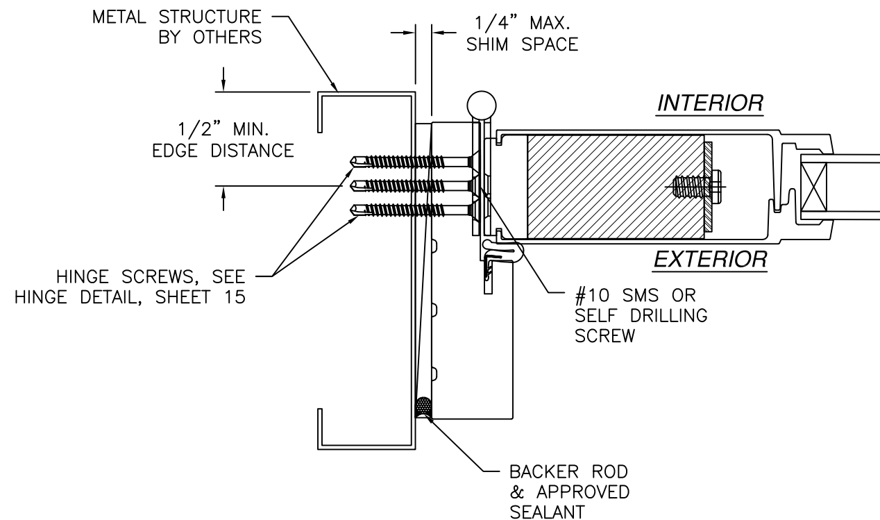
DOOR INSTALLATION DETAIL METAL STRUCTURE INSTALLATION
