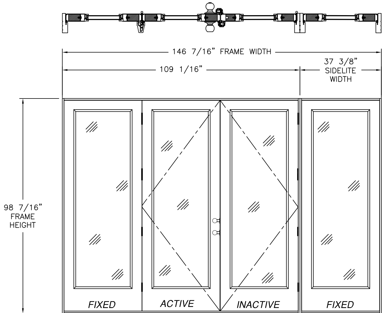
SERIES SLPS IN-SWING SIDE-HINGED DOOR W/SIDELITES (OXX/O)
