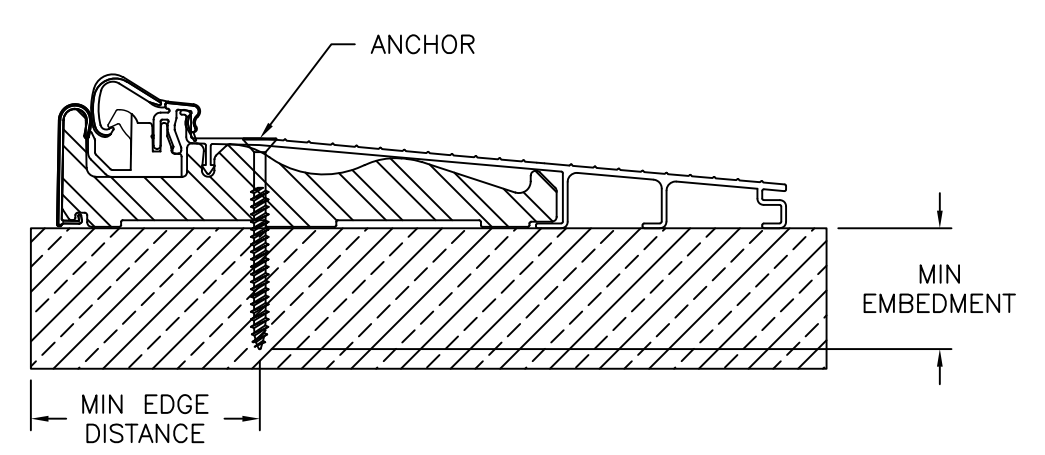
ENDURA THRESHOLD ZAC LH7815
