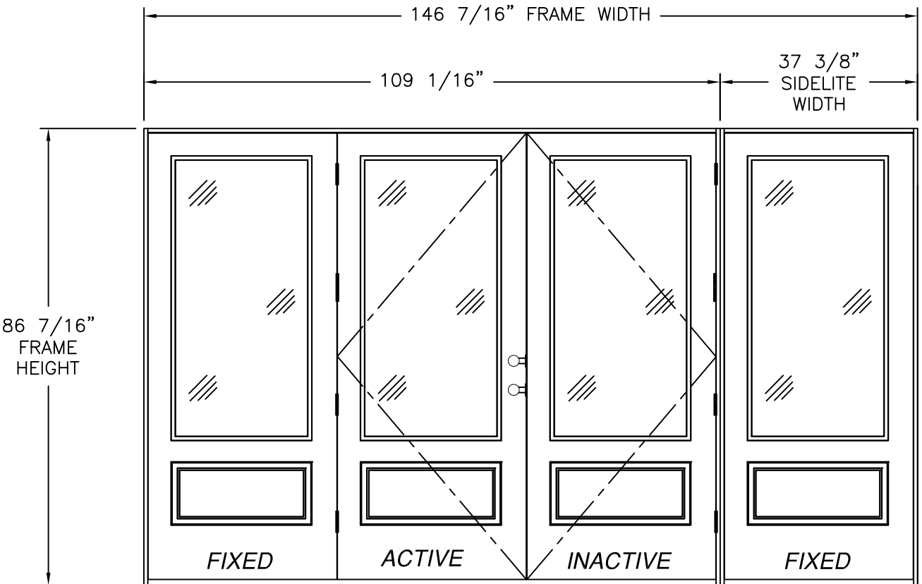
SERIES SLPS IN-SWING SIDE-HINGED DOOR W/SIDELITES (OXX/O)
