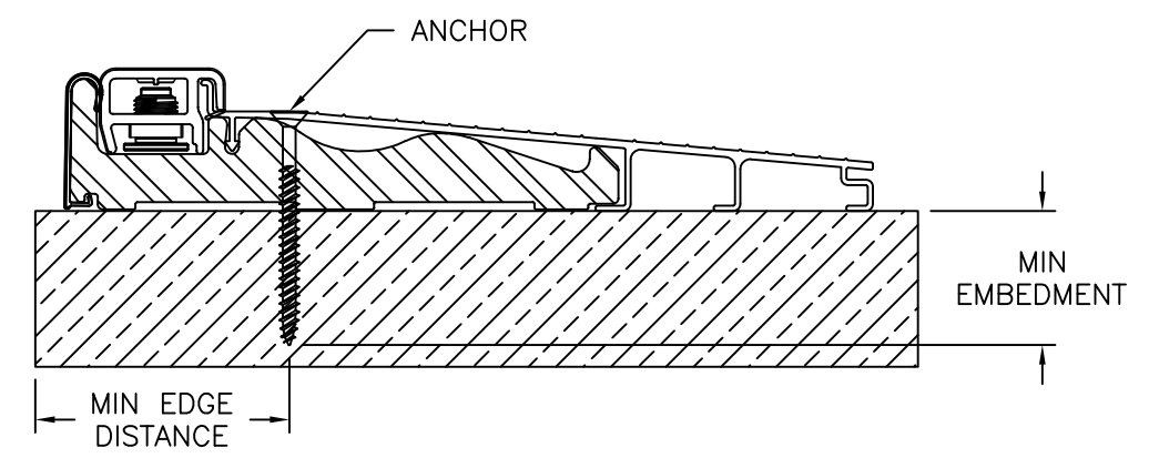
ENDURA THRESHOLD ZAIL H 7625
