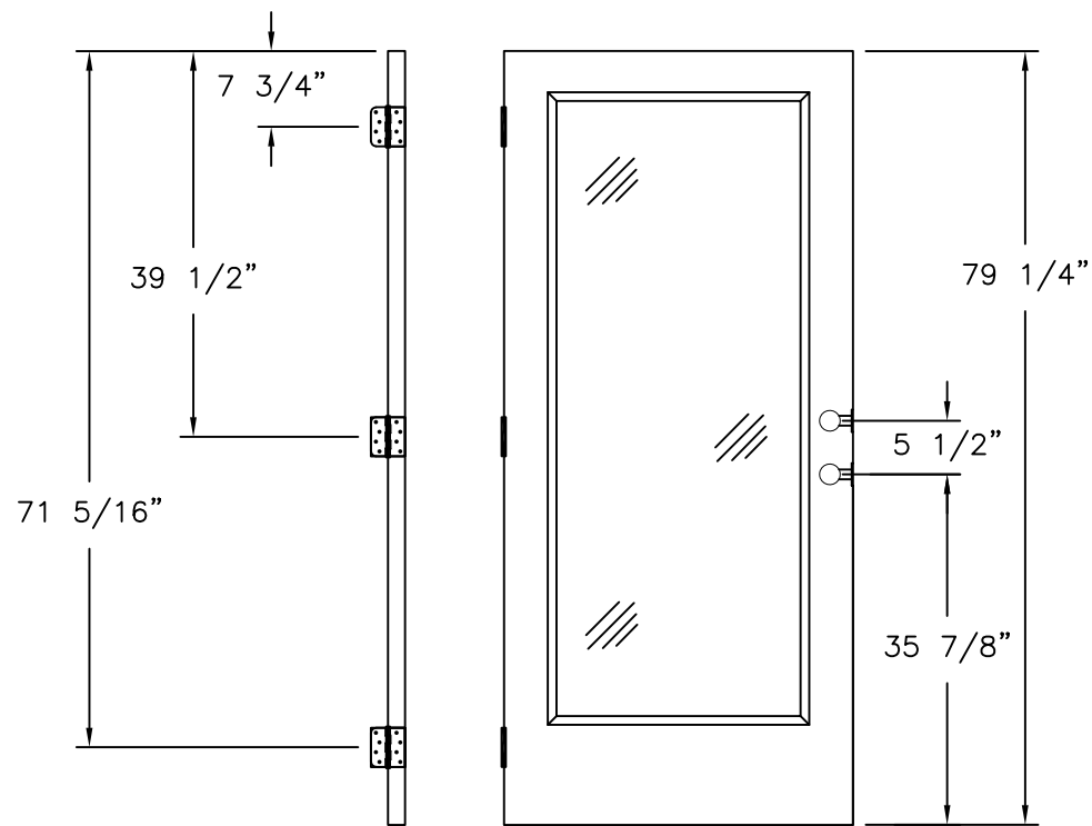
LOCK AND HINGES LOCATIONS 6'8\"/>
