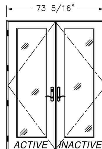
DOUBLE (XX) EXTERIOR VIEW FULL LITE SHOWN, 3/4 & 1/2 LITE SIMILAR
