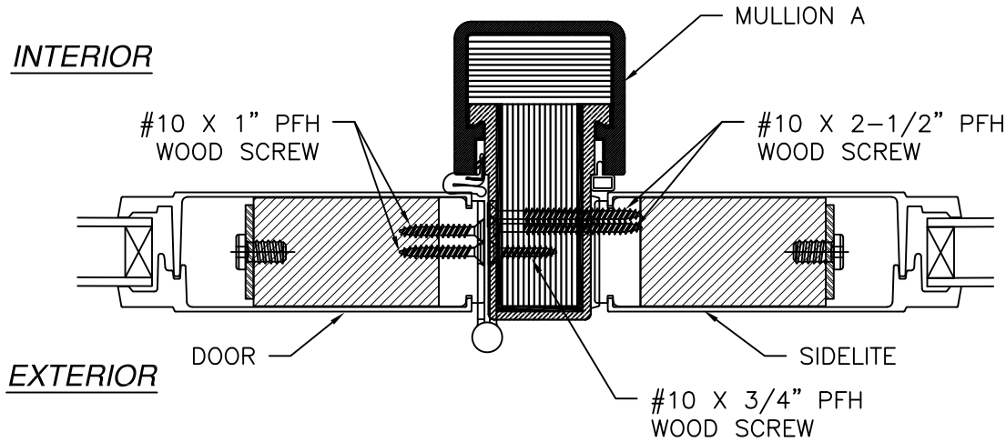
T-MULLION DETAIL
