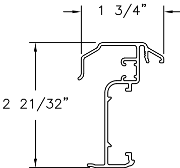
ENDURA ULTIMATE PUSH BUTTON ASTRAGAL ALTERNATE
