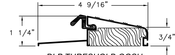
DLP THRESHOLD QOSH ALTERNATE
