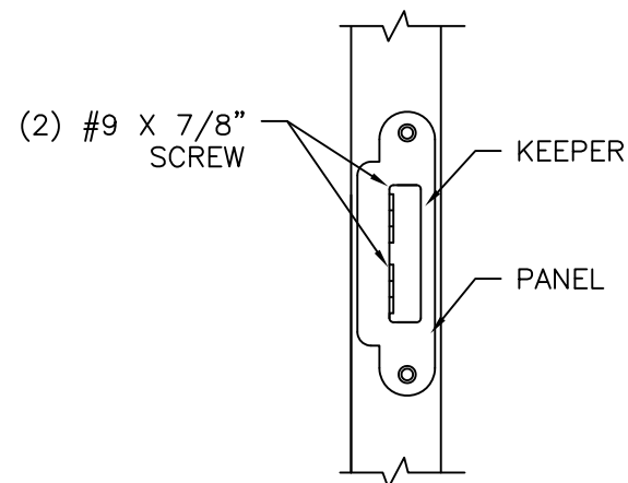
SLAB MULTI-POINT LOCK KEEPER DETAIL
