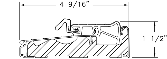
ENDURA THRESHOLD ZOBLH4565 ALTERNATE
