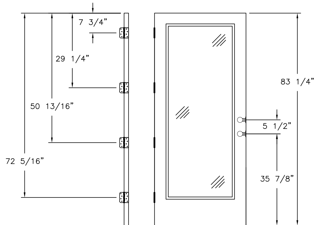
LOCK AND HINGES LOCATIONS 7' UNIT, WITH LATCH AND DEADBOLT, FULL LITE, 3/4 AND 1/2 LITE PANELS
