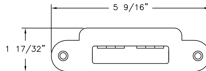
SLAB MULTI-POINT LOCK KEEPER STEEL
