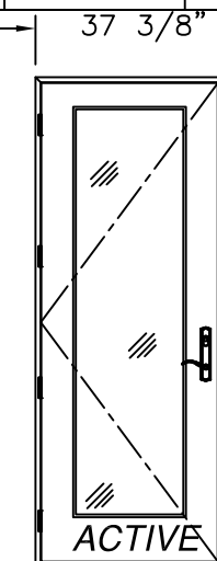
SINGLE (X) EXTERIOR VIEW FULL LITE SHOWN, 3/4 & 1/2 LITE SIMILAR
