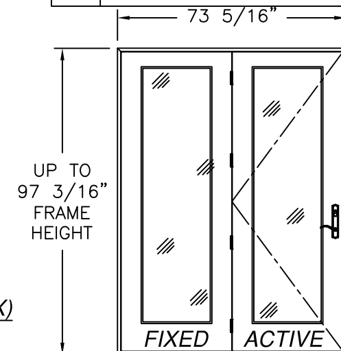
SINGLE W/SIDELITE (OX, XO) EXTERIOR VIEW FULL LITE SHOWN, 3/4 & 1/2 LITE SIMILAR
