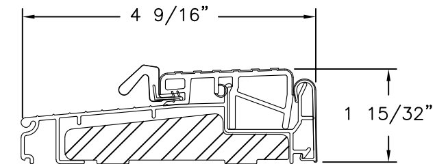
ENDURA THRESHOLD ZOBL4565 ALTERNATE
