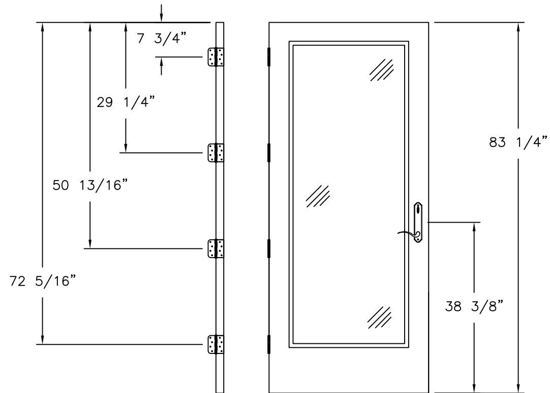
LOCK AND HINGES LOCATIONS 7' UNIT, WITH HANDLE, FULL LITE, 3/4 AND 1/2 LITE PANELS
