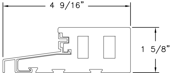
DOOR SILL FOAM PVC CO-EX & ALUMINUM
