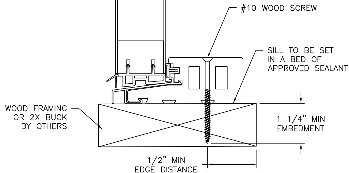
SIDELITE DOOR INSTALLATION DETAIL 2X BUCK/WOOD FRAMING INSTALLATION FULL LITE SHOWN, 3/4 & 1/2 LITE SIMILAR
