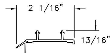
DOOR BOTTOM-A PVC CO-EX
