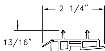
DOOR BOTTOM-B PVC CO-EX
