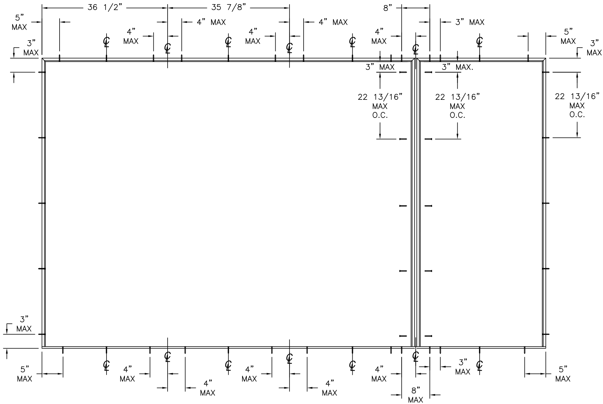
ANCHORING LAYOUT
