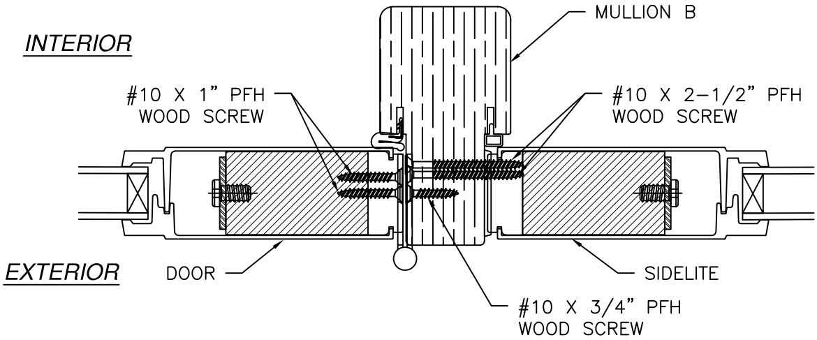
ENDURA T-MULLION DETAIL
