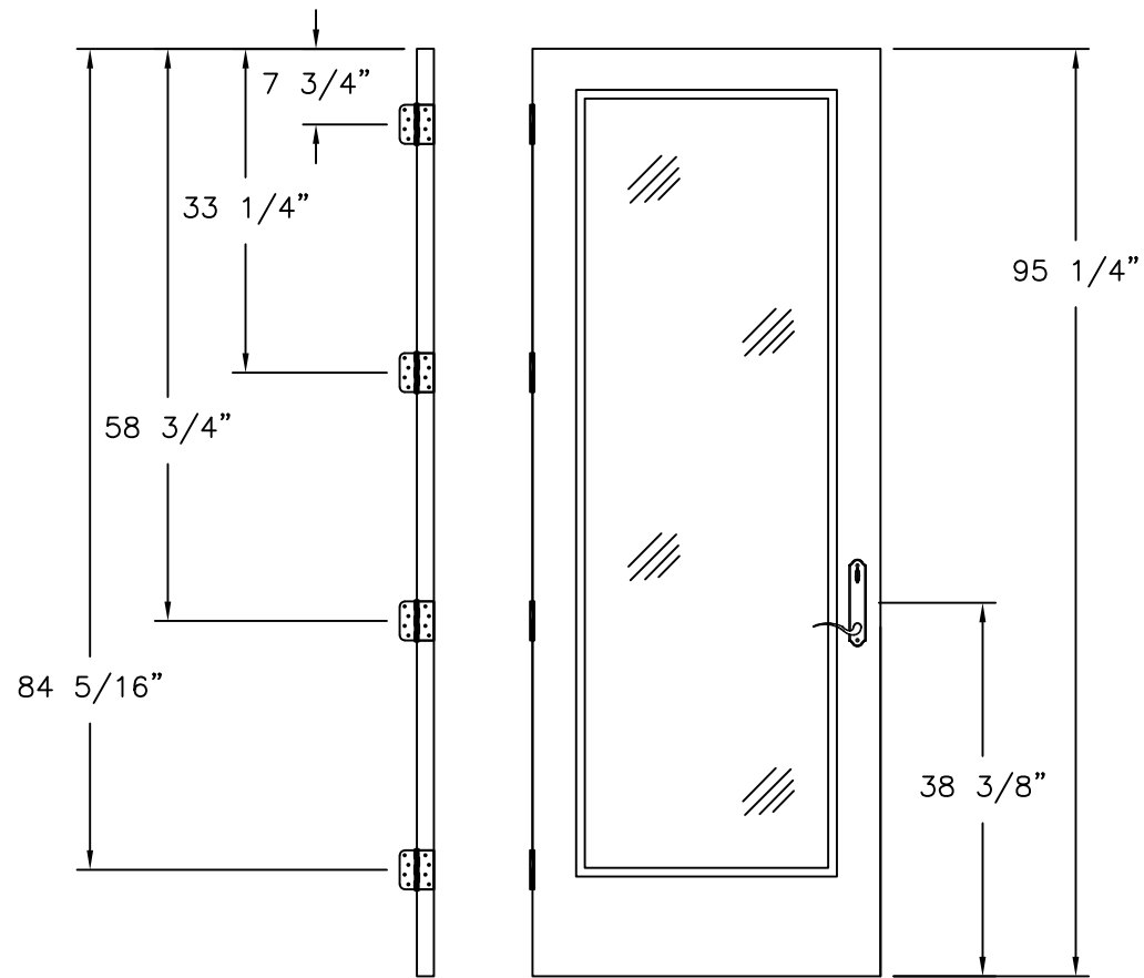
LOCK AND HINGES LOCATIONS 8' UNIT, WITH HANDLE, FULL LITE, 3/4 AND 1/2 LITE PANELS
