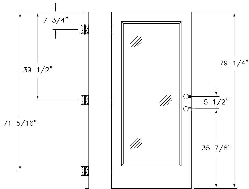
LOCK AND HINGES LOCATIONS 6' UNIT, WITH LATCH AND DEADBOLT, FULL LITE, 3/4 AND 1/2 LITE PANELS
