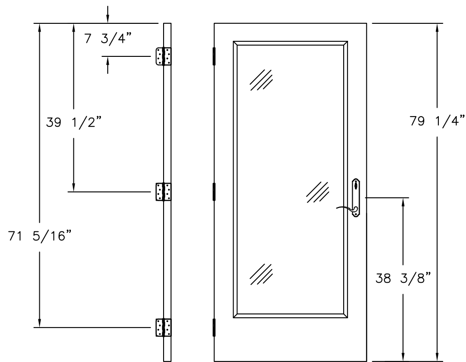
LOCK AND HINGES LOCATIONS 6'8" UNIT, WITH HANDLE, FULL LITE, 3/4 AND 1/2 LITE PANEL
