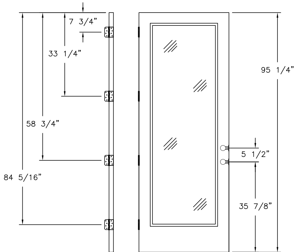
LOCK AND HINGES LOCATIONS 8' UNIT, WITH LATCH AND DEADBOLT, FULL LITE, 3/4 AND 1/2 LITE PANELS
