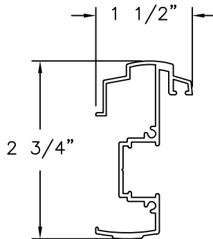
COLUMBIA T-ASTRAGAL .060" THICKNESS, ALUMINUM 6063-T5 ALTERNATE
