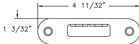
HOOK KEEPER STAINLESS STEEL (SS92G)
