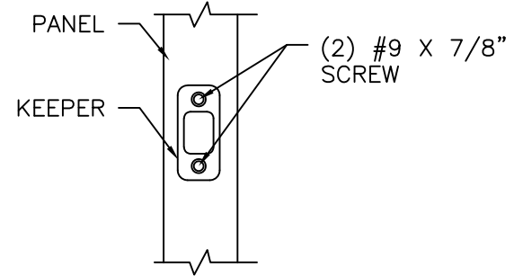
DEADBOLT KEEPER DETAIL
