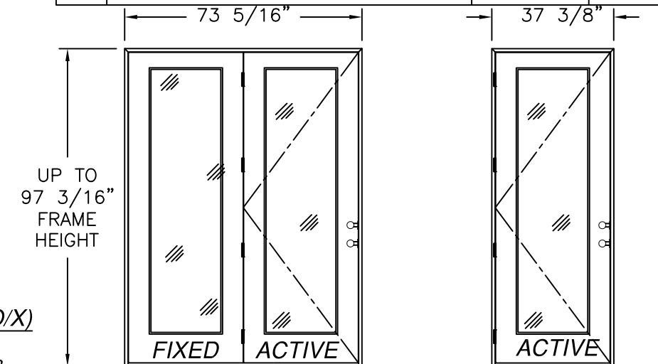
SINGLE (X) EXTERIOR VIEW FULL LITE SHOWN, 3/4 & 1/2 LITE SIMILAR
