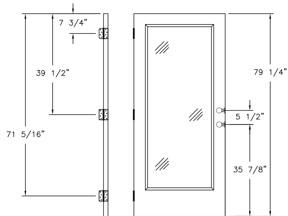
LOCK AND HINGES LOCATIONS 6'8" UNIT, FULL LITE, 3/4 & 1/2 LITE PANELS
