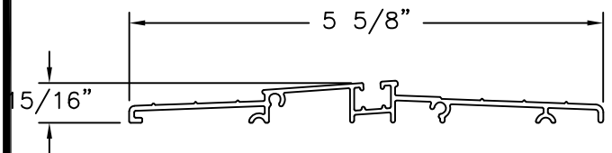
ENDURA ADA THRESHOLD ZHCO5622 ALTERNATE
