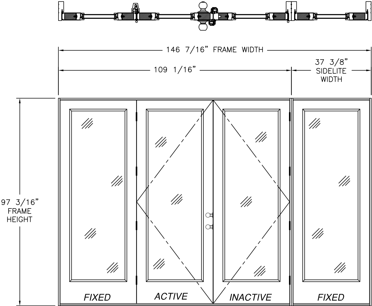
SERIES SLPS OUT-SWING SIDE-HINGED DOOR W/SIDELITES (OXX/O) 8' UNIT EXTERIOR VIEW FULL LITE PANELS REFER TO SHEET 5 FOR HARDWARE AND NOTES
