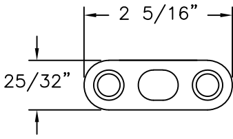
DRIVE BAR PLATE STAINLESS STEEL
