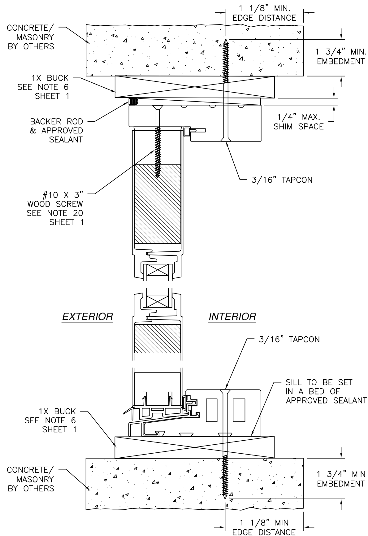
VERTICAL CROSS SECTION CONCRETE/MASONRY WITH 1X BUCK INSTALLATION FOR CONCRETE/MASONRY WITHOUT 1X BUCK REFER TO JAMB INSTALLATION DETAIL
