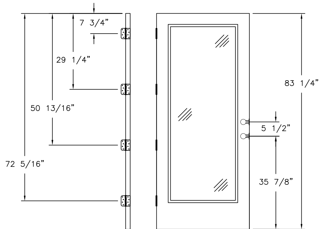
LOCK AND HINGES LOCATIONS 7' UNIT, FULL LITE, 3/4 & 1/2 LITE PANELS
