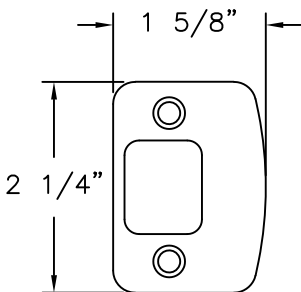
LATCH KEEPER STAINLESS STEEL
