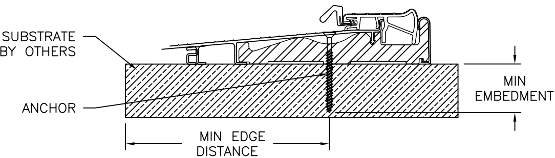
ENDURA THRESHOLD ZOBLH7815
