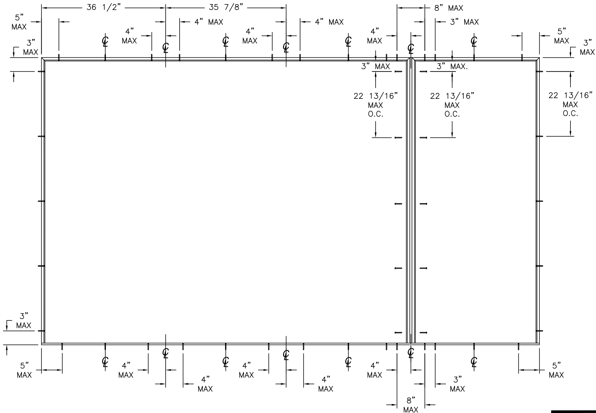
ANCHORING LAYOUT
