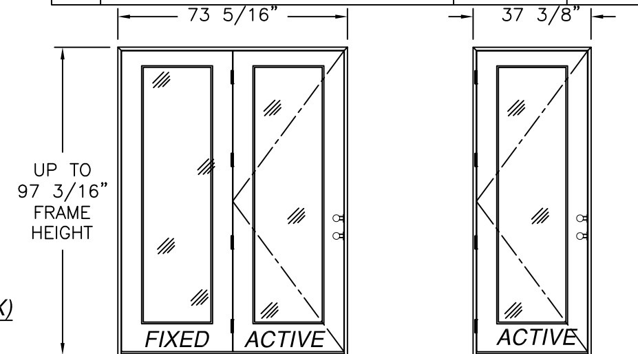
SINGLE W/SIDELITE (OX, XO) EXTERIOR VIEW FULL LITE SHOWN, 3/4 & 1/2 LITE SIMILAR SINGLE (X) EXTERIOR VIEW FULL LITE SHOWN, 3/4 & 1/2 LITE SIMILAR
