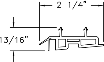
DOOR BOTTOM-B PVC CO-EX
