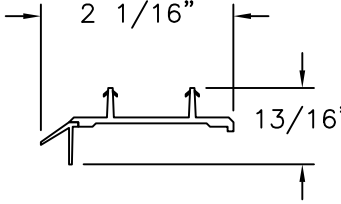
DOOR BOTTOM-A PVC CO-EX
