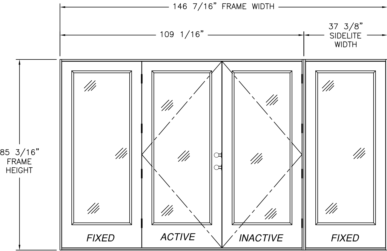
SERIES SLPS OUT-SWING SIDE-HINGED DOOR W/SIDELITES (OXX/O) 7' UNIT EXTERIOR VIEW FULL LITE PANELS REFER TO SHEET 5 FOR HARDWARE AND NOTES
