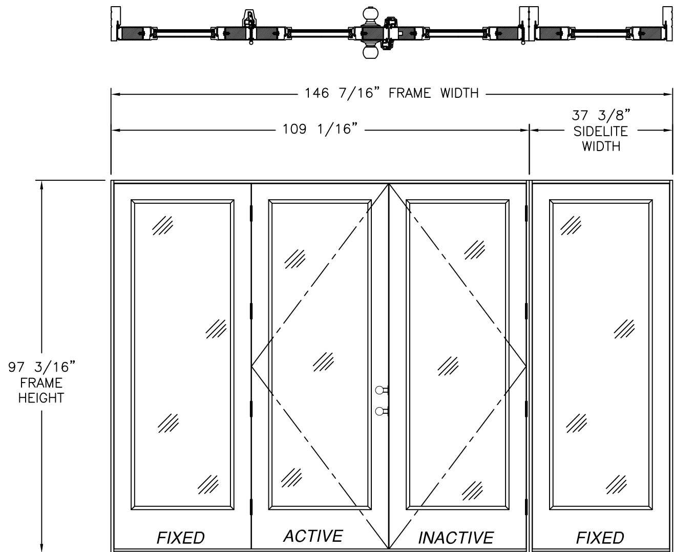
SERIES SLPS OUT-SWING SIDE-HINGED DOOR W/SIDELITES (OXX/O) 8' UNIT EXTERIOR VIEW FULL LITE PANELS REFER TO UNIT 5 FOR HARDWARE AND NOTES
