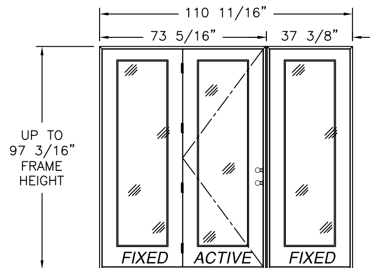
SINGLE W/SIDELITE MULL. (OX/O, O/XO) EXTERIOR VIEW FULL LITE SHOWN, 3/4 & 1/2 LITE SIMILAR
