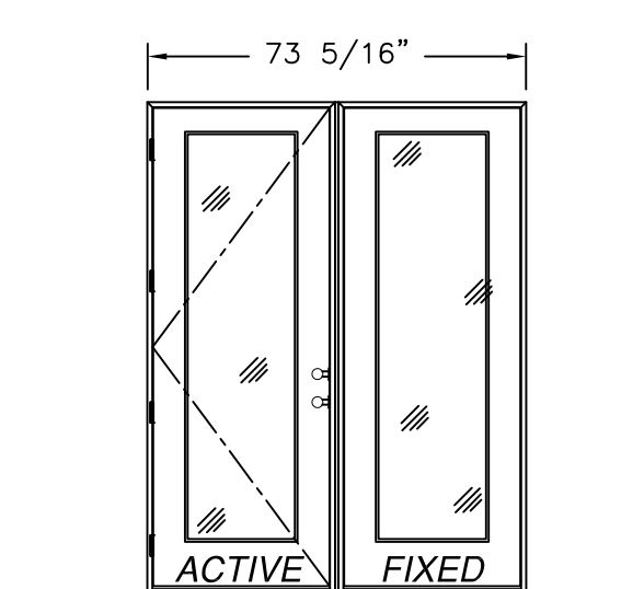
SINGLE W/SIDELITE MULL. (X/O, O/X) EXTERIOR VIEW FULL LITE SHOWN, 3/4 & 1/2 LITE SIMILAR
