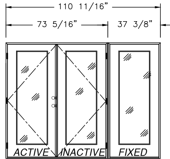
DOUBLE W/SIDELITE MULL. (XX/O, O/XX) EXTERIOR VIEW FULL LITE SHOWN, 3/4 & 1/2 LITE SIMILAR
