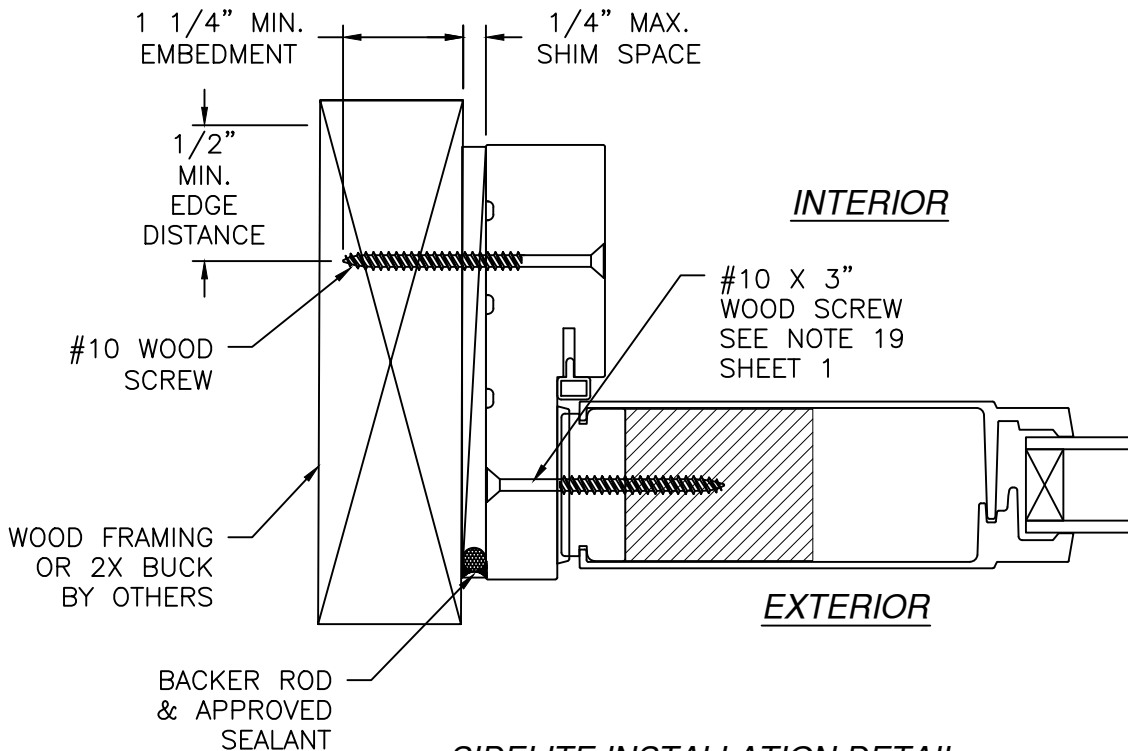
SIDELITE INSTALLATION DETAIL WOOD FRAMING OR 2X BUCK
