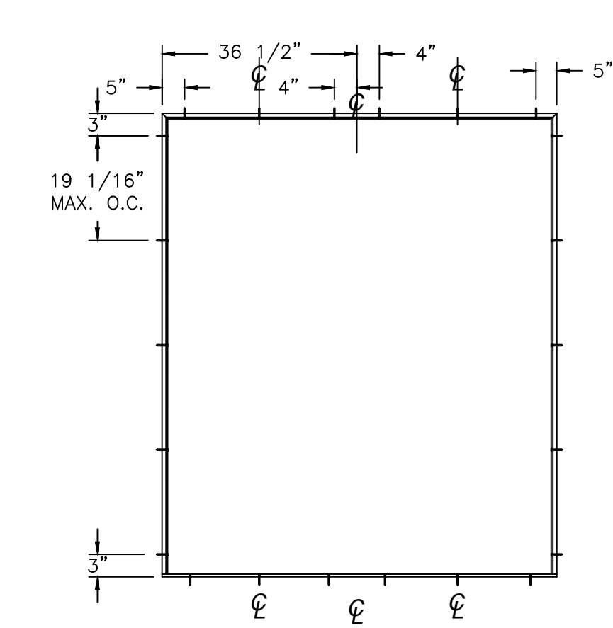
ANCHORING LAYOUT FOR XX, OX AND XO
