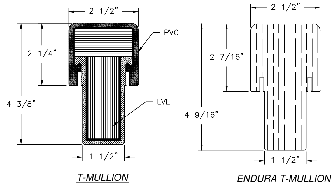
ENDURA T-MULLION DETAIL
