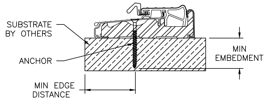
ENDURA THRESHOLD ZOBLH4565
