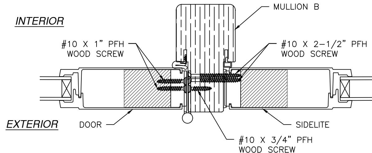
ENDURA T-MULLION DETAIL
