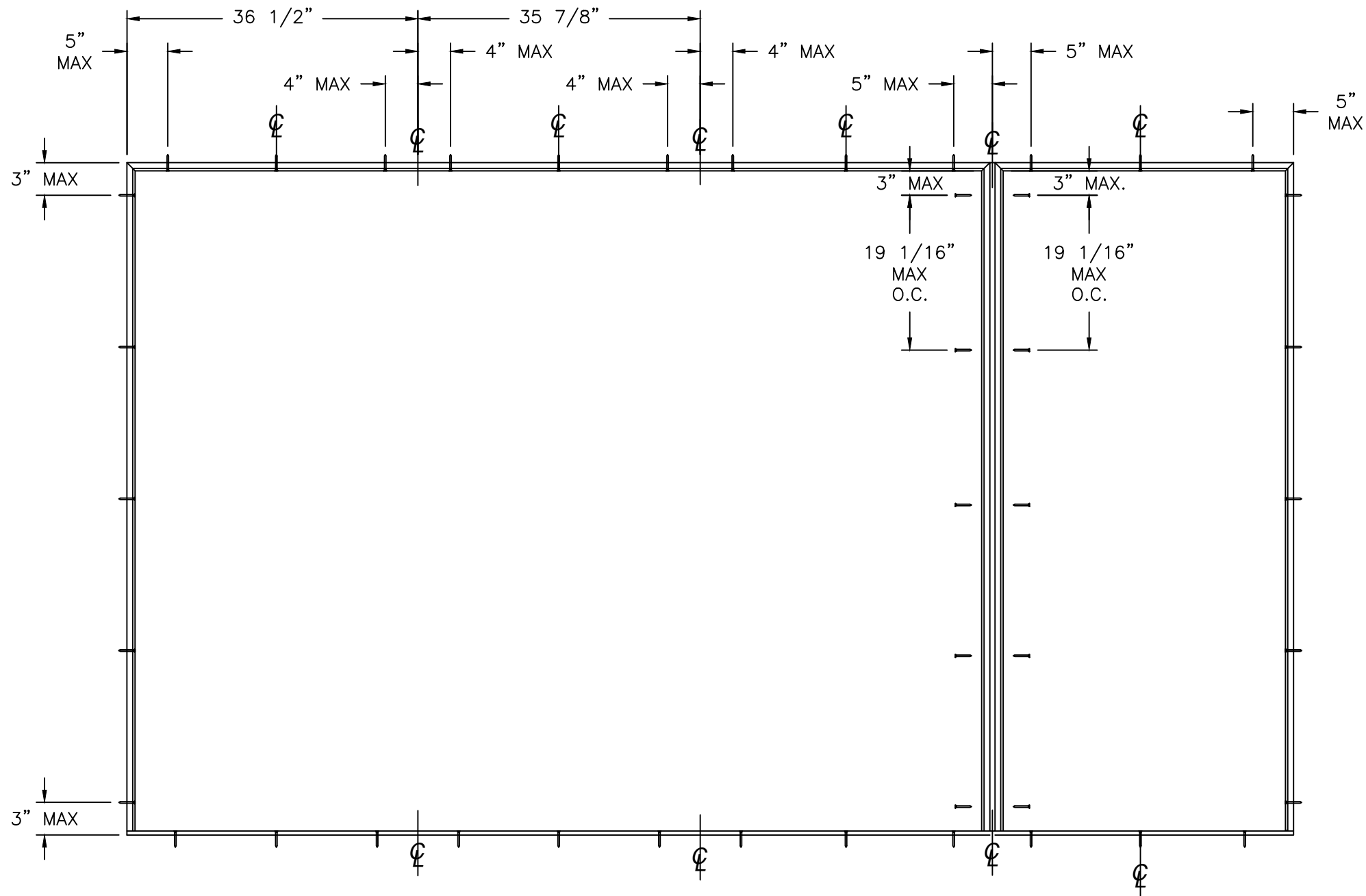
ANCHORING LAYOUT
