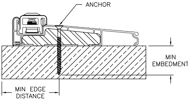
ENDURA THRESHOLD ZAI 5625
