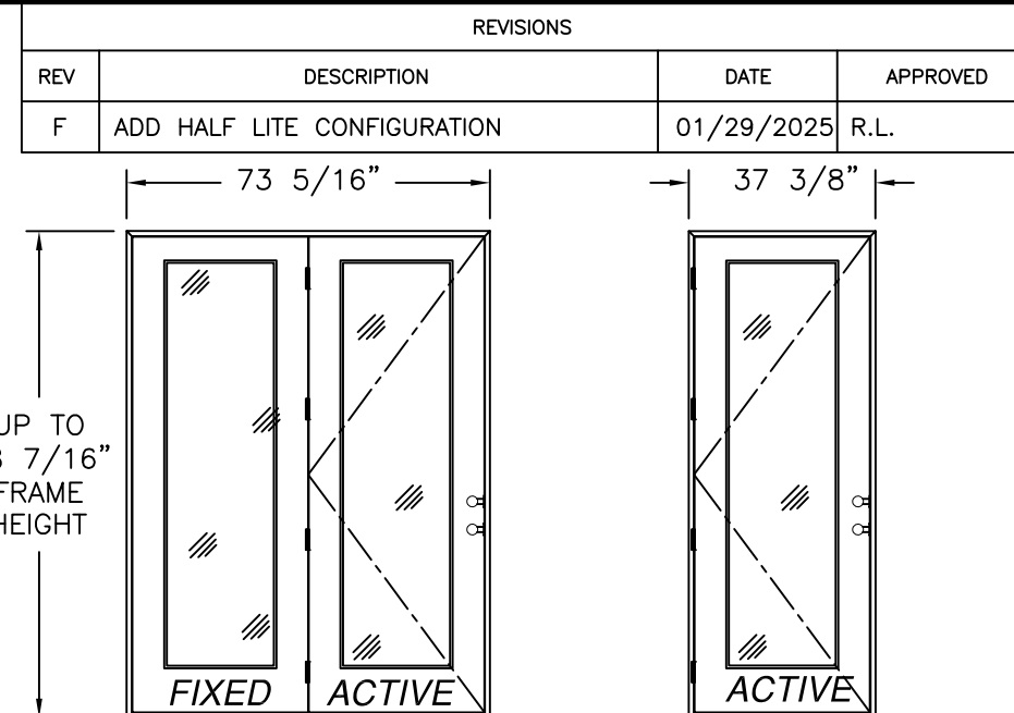
SINGLE W/SIDELITE (OX, XO) EXTERIOR VIEW FULL LITE SHOWN, 3/4 & 1/2 LITE SIMILAR
