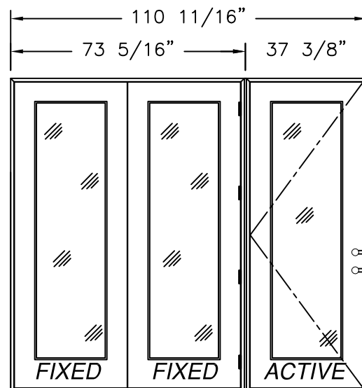
SINGLE W/SIDELITES MULL. (OO/X) EXTERIOR VIEW FULL LITE SHOWN, 3/4 & 1/2 LITE SIMILAR
