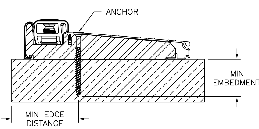
ENDURA THRESHOLD ZAI5815FN
