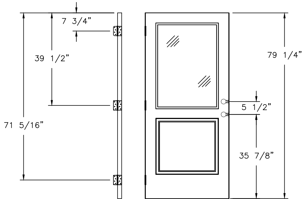
LOCK AND HINGES LOCATIONS 1/2 LITE PANEL
