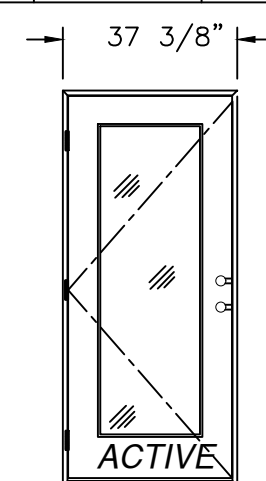
SINGLE (X) EXTERIOR VIEW FULL LITE SHOWN, 3/4 & 1/2 LITE SIMILAR
