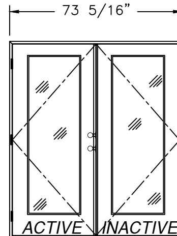
DOUBLE (XX) EXTERIOR VIEW FULL LITE SHOWN, 3/4 & 1/2 LITE SIMILAR
