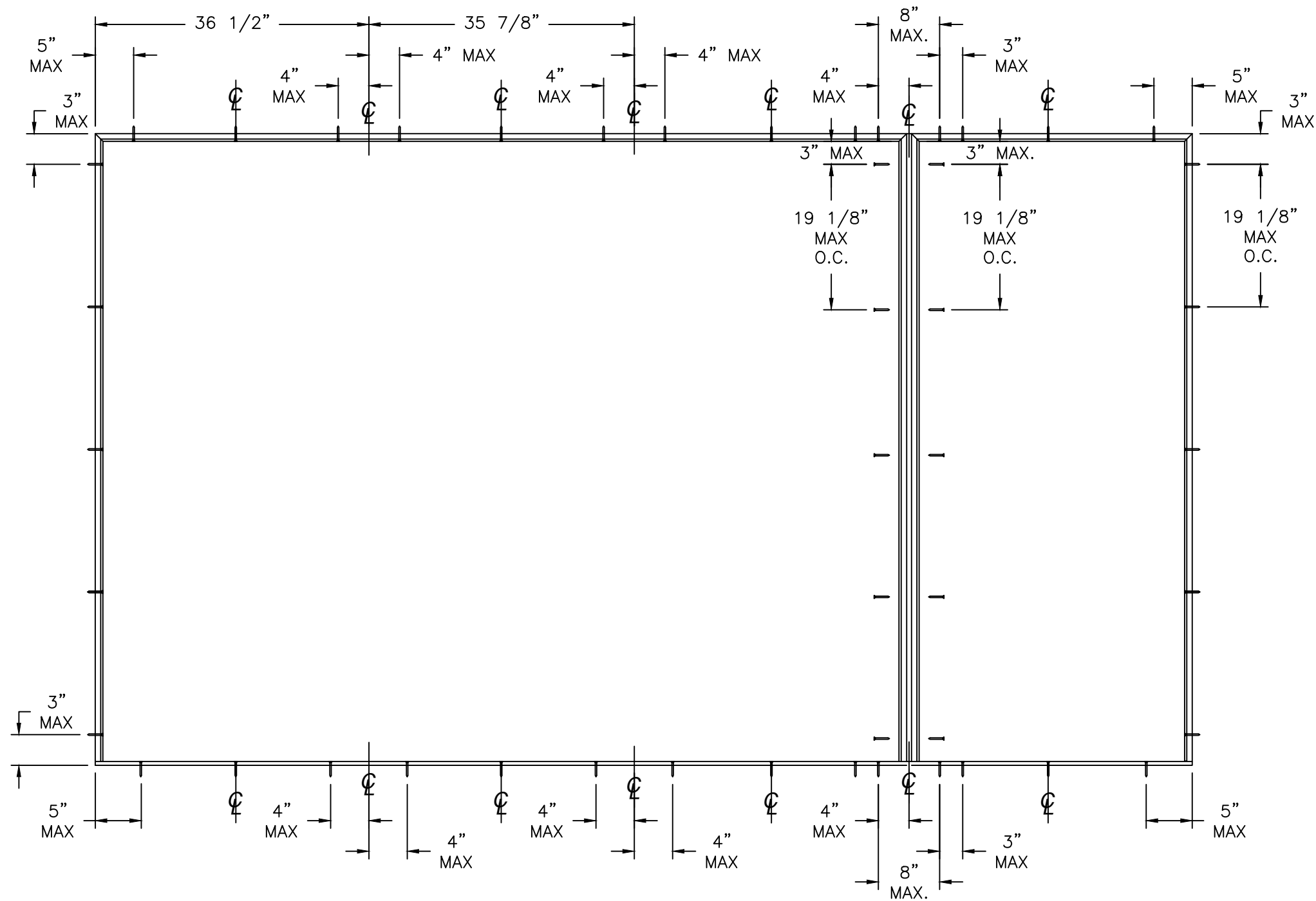
ANCHORING LAYOUT
