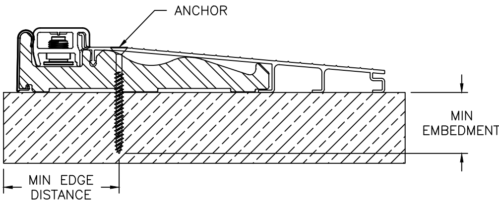
ENDURA THRESHOLD ZAILH7625
