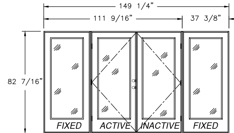
DOUBLE W/SIDELITES MULL. (O/XX/O) EXTERIOR VIEW FULL LITE SHOWN, 3/4 & 1/2 LITE SIMILAR
