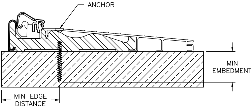
ENDURA THRESHOLD ZAC LH7815
