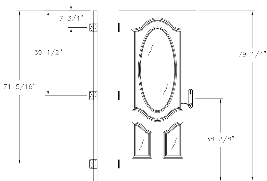
LOCK AND HINGES LOCATIONS WITH HANDLE
