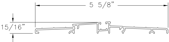
ENDURA ADA THRESHOLD ZHCO5622 ALTERNATE
