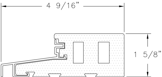
DOOR SILL FOAM PVC CO-EX & ALUMINUM
