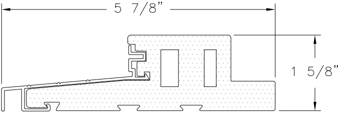
NEUMA SILL ALTERNATE
