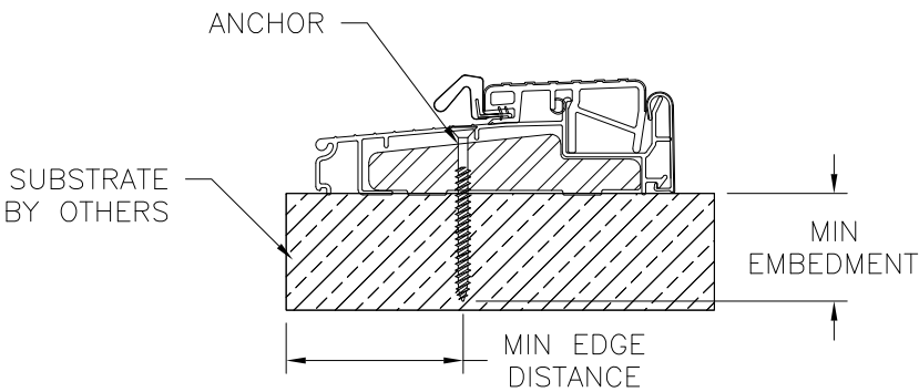
ENDURA THRESHOLD ZOBL4565
