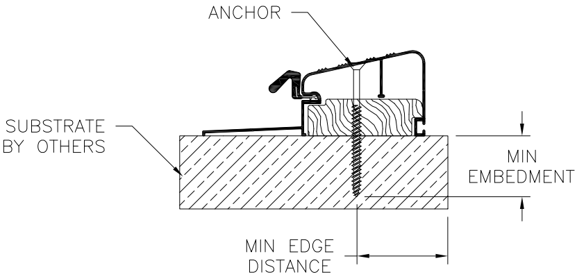
DLP THRESHOLD QOSR
