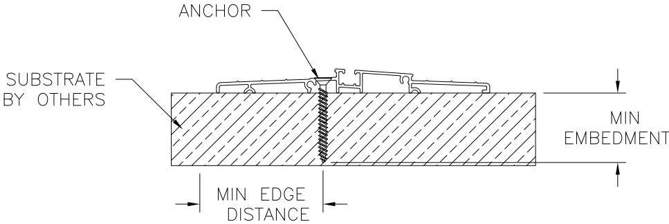
ENDURA ADA THRESHOLD ZHCO5622 TO BE USED ONLY WHERE WATER PENETRATION RESISTANCE IS NOT REQUIRED
