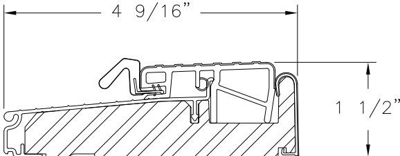
ENDURA THRESHOLD ZOB4565FN ALTERNATE
