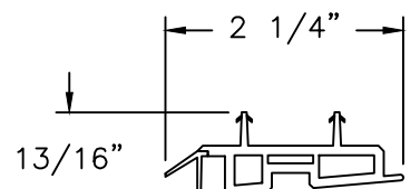
DOOR BOTTOM-B PVC CO-EX
