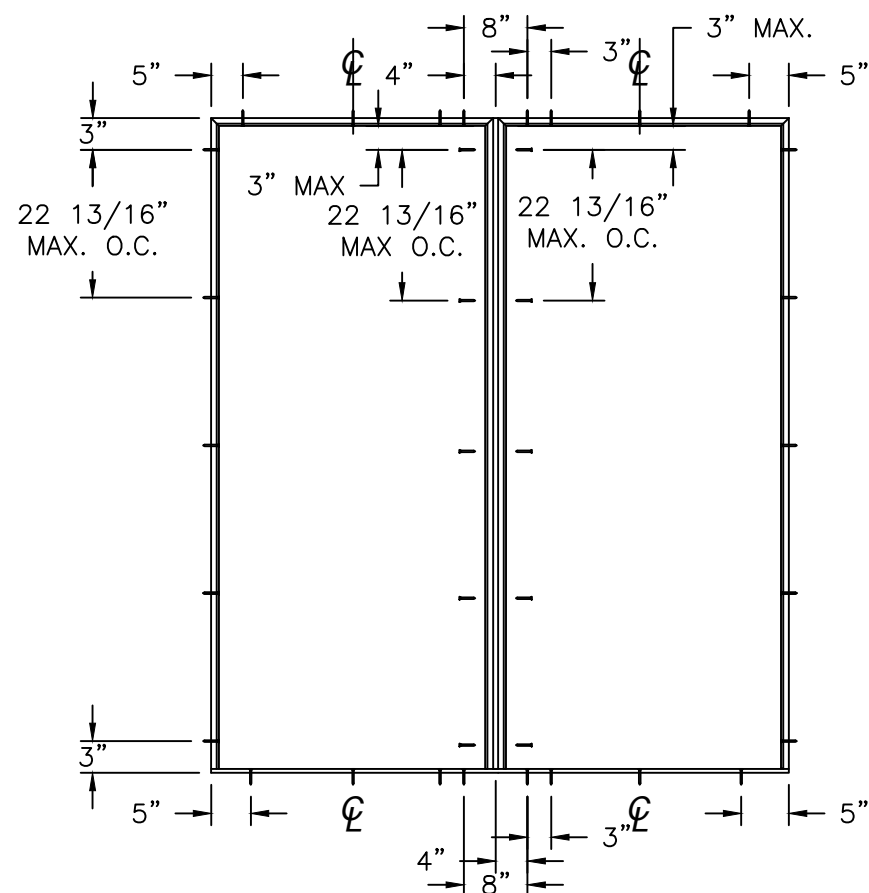
ANCHORING LAYOUT FOR OX AND XO (MULL)
