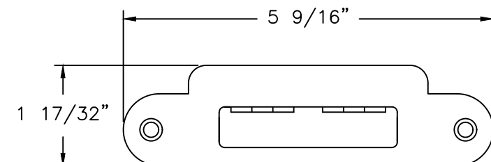
SLAB MULTI-POINT LOCK KEEPER STEEL
