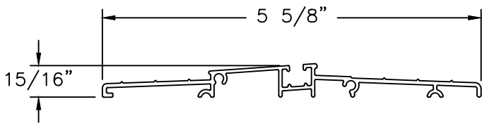
ENDURA ADA THRESHOLD ZHCO5622 ALTERNATE
