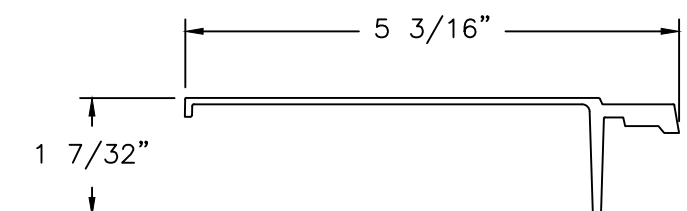
SHEET MOLDING COMPOUND SKIN-1 FIBERGLASS
