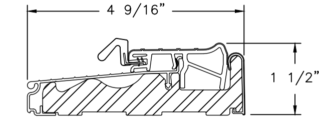
ENDURA THRESHOLD ZOBLH4565 ALTERNATE
