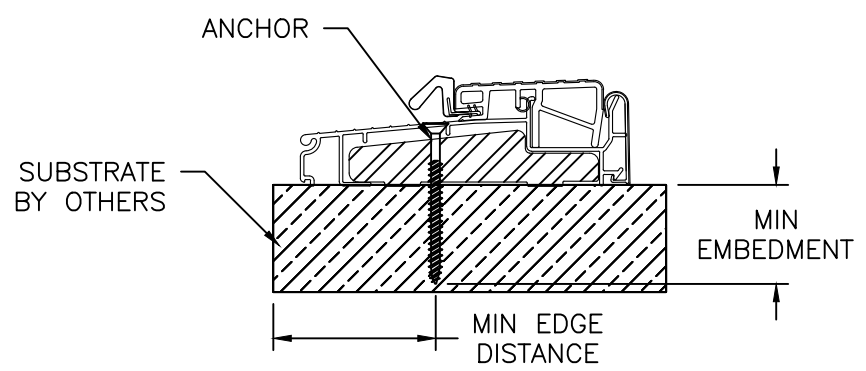
ENDURA THRESHOLD ZOBL4565
