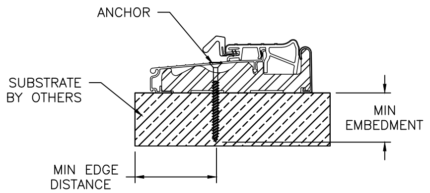
ENDURA THRESHOLD ZOBLH4565
