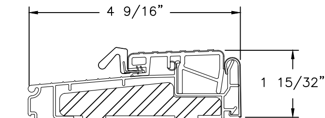
ENDURA THRESHOLD ZOBL4565 ALTERNATE
