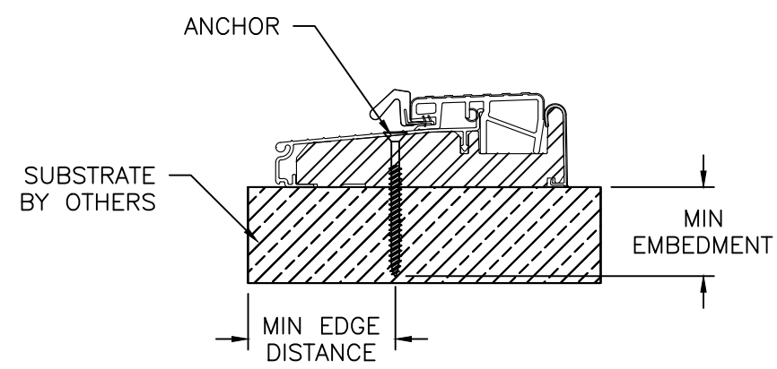
ENDURA THRESHOLD ZOB4565FN
