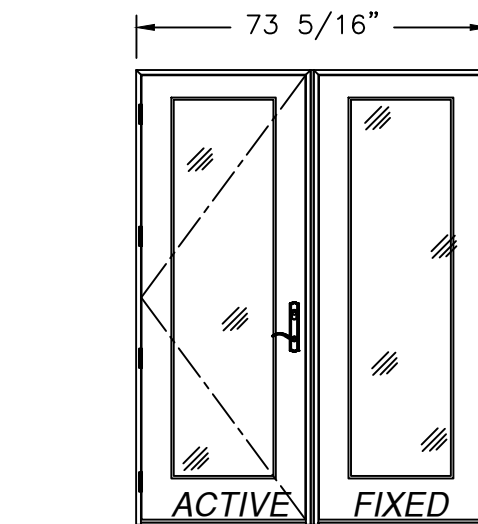
SINGLE W/SIDELITE MULL. (X/O, O/X) EXTERIOR VIEW FULL LITE SHOWN, 3/4 & 1/2 LITE SIMILAR
