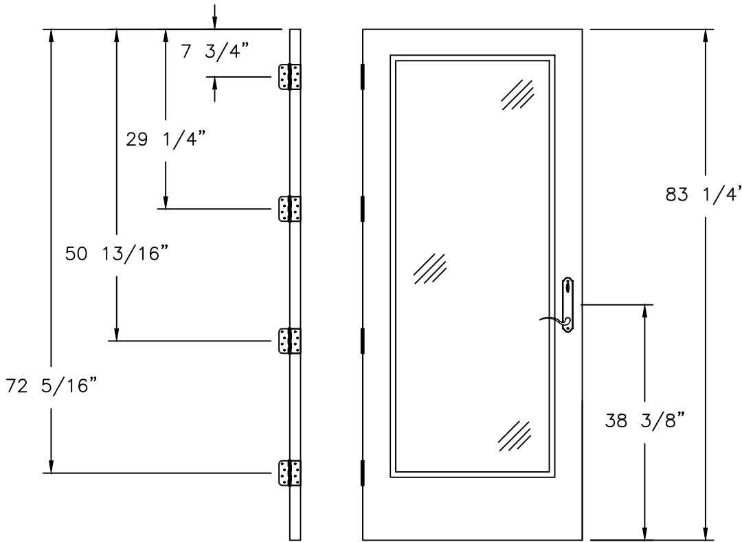
LOCK AND HINGES LOCATIONS 7' UNIT, WITH HANDLE, FULL LITE, 3/4 AND 1/2 LITE PANELS
