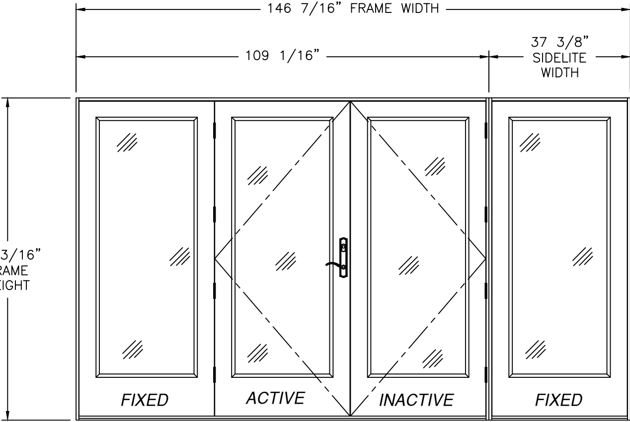
SERIES SLPS OUT-SWING SIDE-HINGED DOOR W/SIDELITES (OXX/O) 7' UNIT EXTERIOR VIEW FULL LITE PANELS REFER TO SHEET 5 FOR HARDWARE AND NOTES
