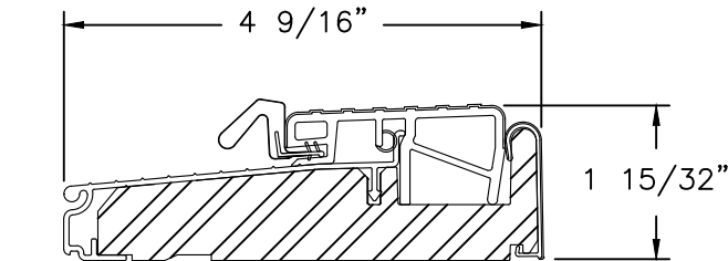
ENDURA THRESHOLD ZOB4565FN ALTERNATE
