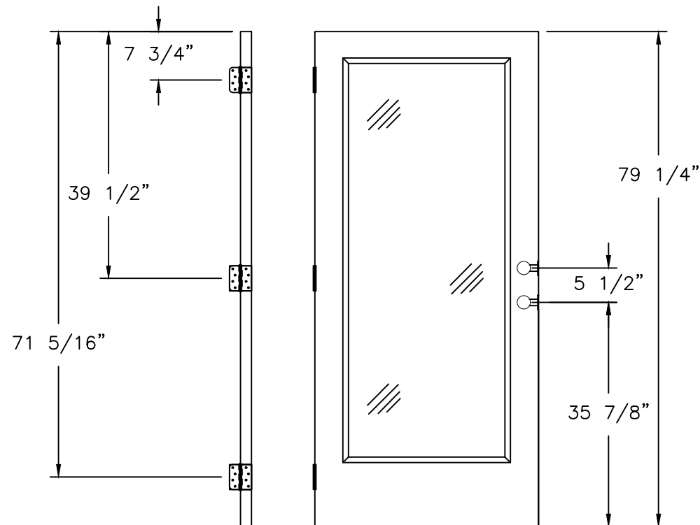
LOCK AND HINGES LOCATIONS 6'8" UNIT, WITH LATCH AND DEADBOLT, FULL LITE, 3/4 AND 1/2 LITE PANELS
