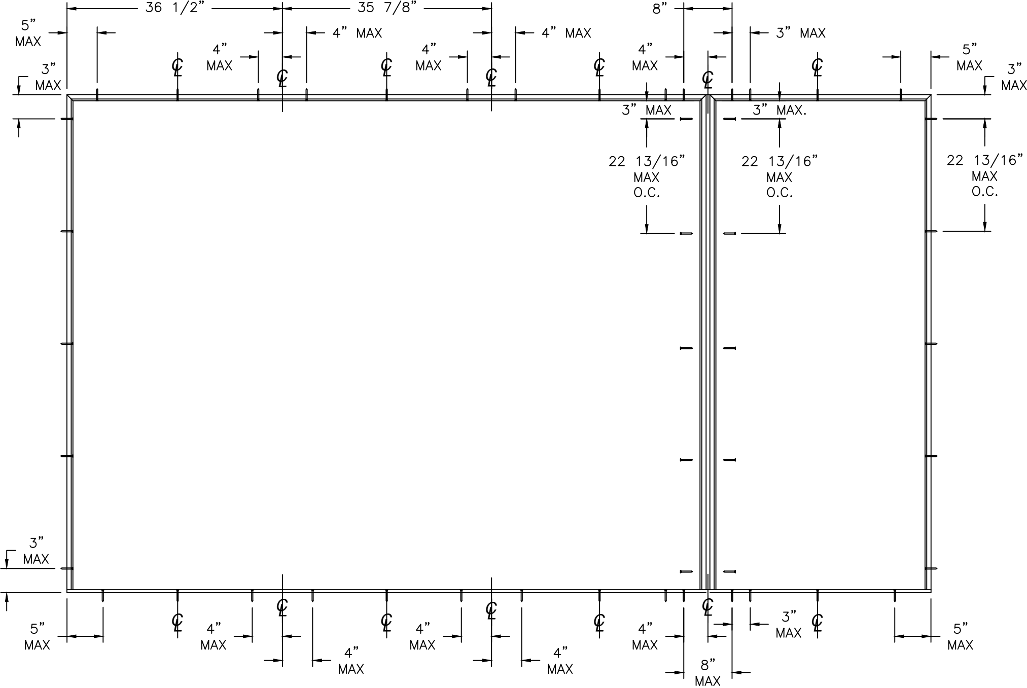
ANCHORING LAYOUT
