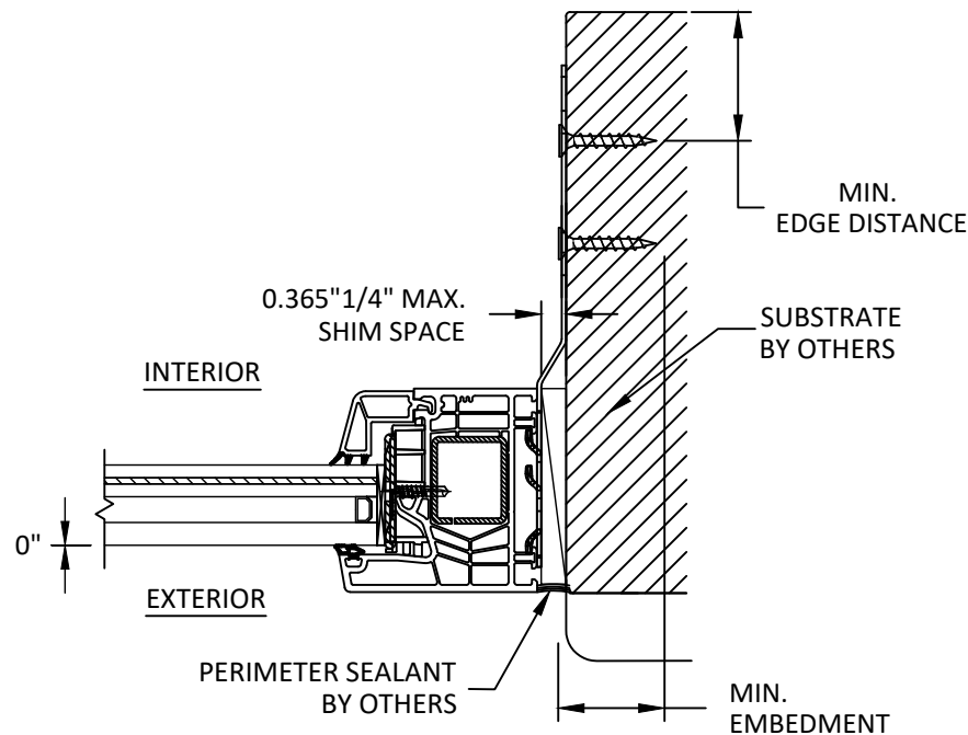
B 4 HORIZONTAL SECTION STRAP (JAMB)
