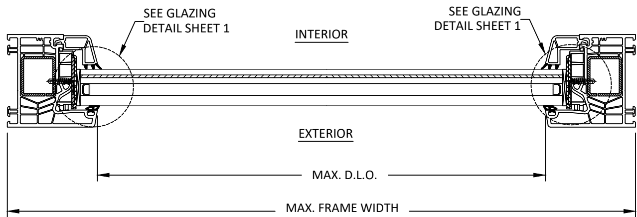
B 3 HORIZONTAL SECTION FIXED WINDOW
