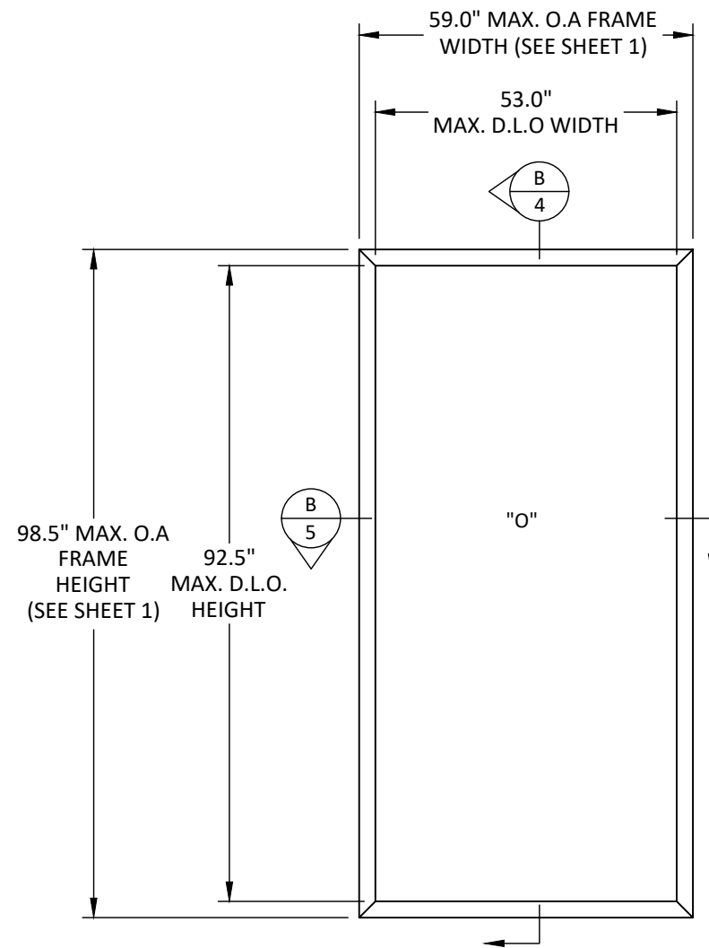
ELEVATION FIXED WINDOW - SINGLE
