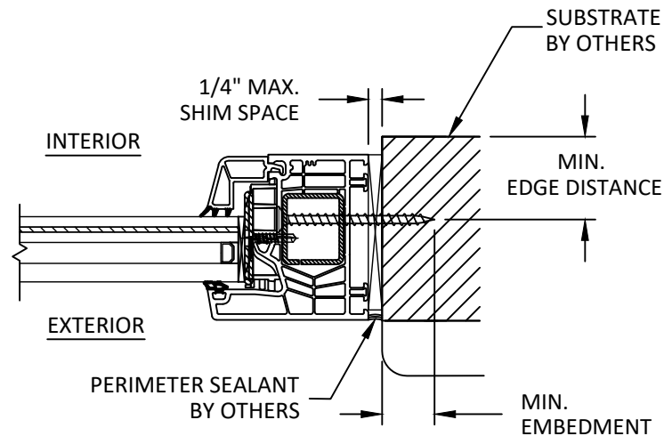
A 4 HORIZONTAL SECTION THROUGH FRAME (JAMB)
