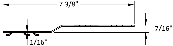
6 ANCHOR STRAP
