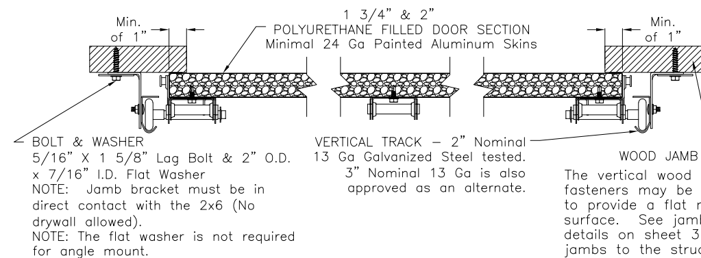
DETAIL H
