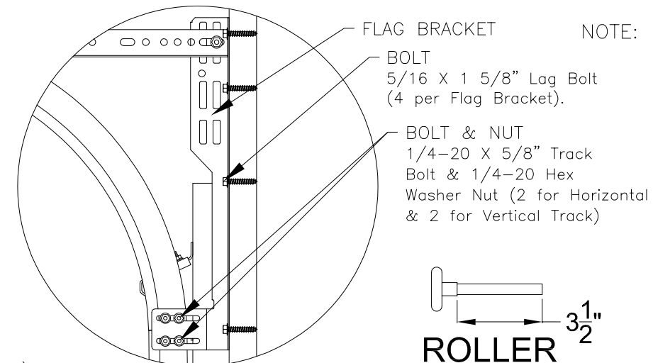
DETAIL H
