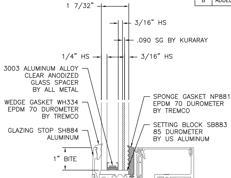
GLAZING DETAIL
