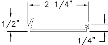
PICTURE WINDOW COVER PW803 ALUMINUM 6063-T5
