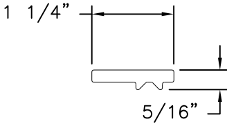
SETTING BLOCK SB883
