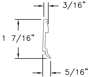
GLAZING STOP SH884
