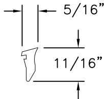
WEDGE GASKET WH334
