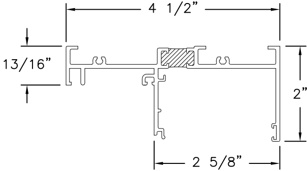
HEAD/JAMB EXTRUSION PW954 ALUMINUM 6063-T5
