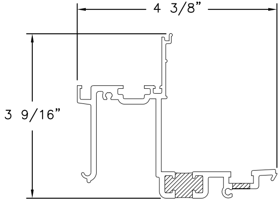
SILL INSERT HS804 ALUMINUM 6063-T5
