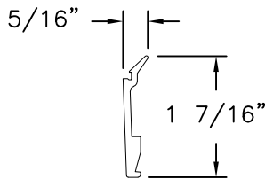
GLAZING STOP SH884 ALUMINUM 6063-T5
