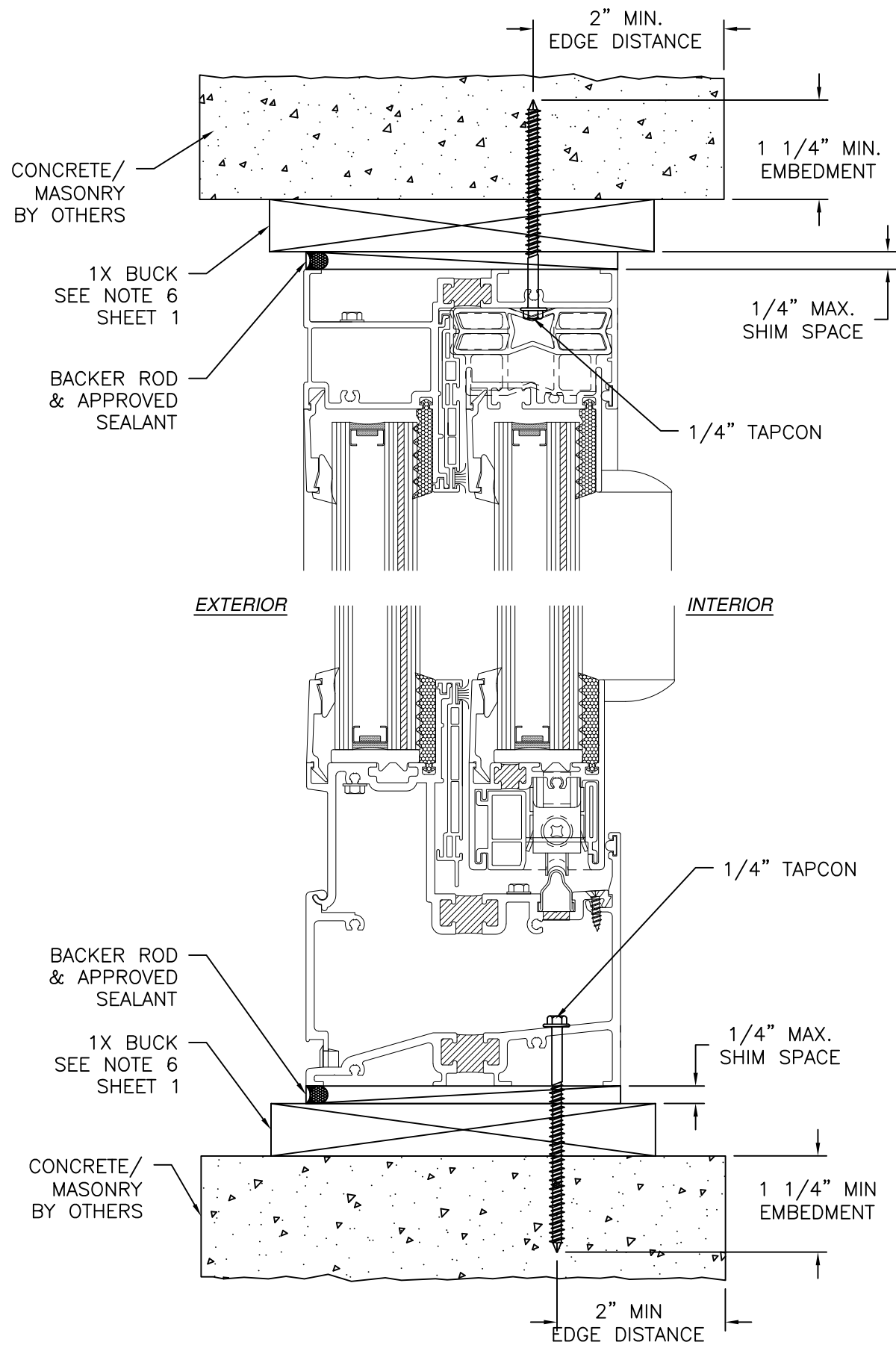
VERTICAL CROSS SECTION CONCRETE/MASONRY INSTALLATION WITH 1X BUCK INSTALLATION FOR CONCRETE/MASONRY WITHOUT 1X BUCK REFER TO JAMB INSTALLATION DETAILS
