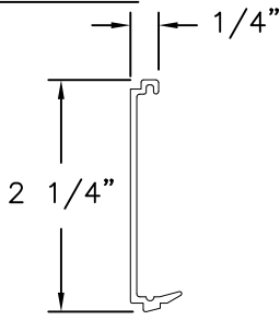
PICTURE WINDOW COVER PW803 ALUMINUM 6063-T5
