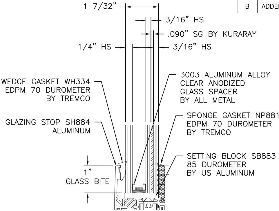
GLAZING DETAIL
