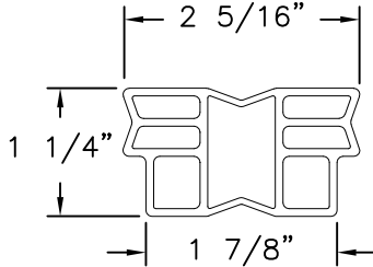
VENT STOP WH853 RIGID PVC
