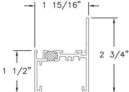
BOTTOM RAIL EXTRUSION HS813 ALUMINUM 6063-T5
