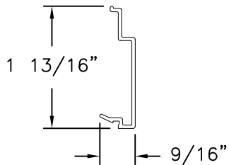
EXTERIOR FRAME COVER HS836 ALUMINUM 6063-T5
