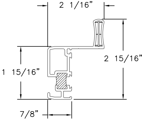
JAMB STILE EXTRUSION HS815 ALUMINUM 6063-T5
