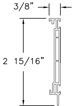
SILL ISOLATOR STRUT WH841 RIGID PVC
