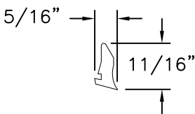
WEDGE GASKET WH344 RIGID PVC
