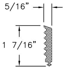
SPONGE GASKET NP881
