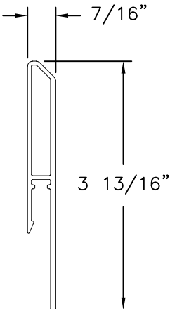
SILL RISER (10300241) ALUMINUM 6063-T5 (.078" THICK)
