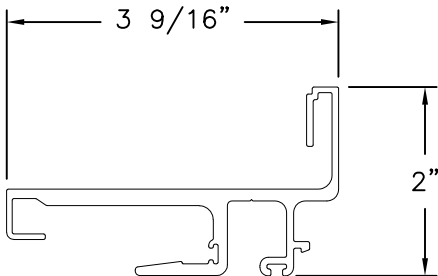
P-HOOK (10300236) ALUMINUM 6063-T5 (.1755" THICK)
