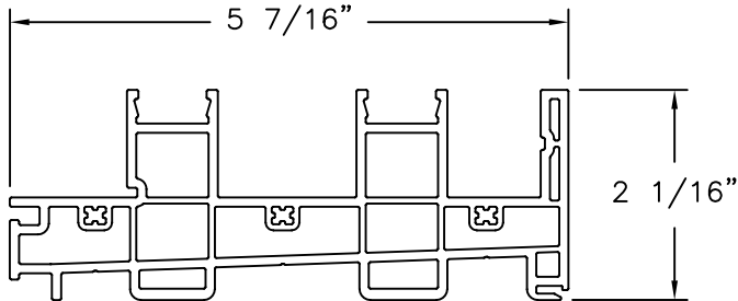
MAIN FRAME (10001160) PVC (.110" THICK)
