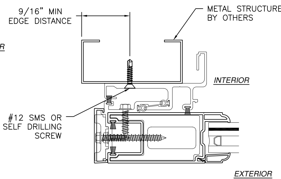
P-HOOK CROSS SECTION METAL STRUCTURE INSTALLATION
