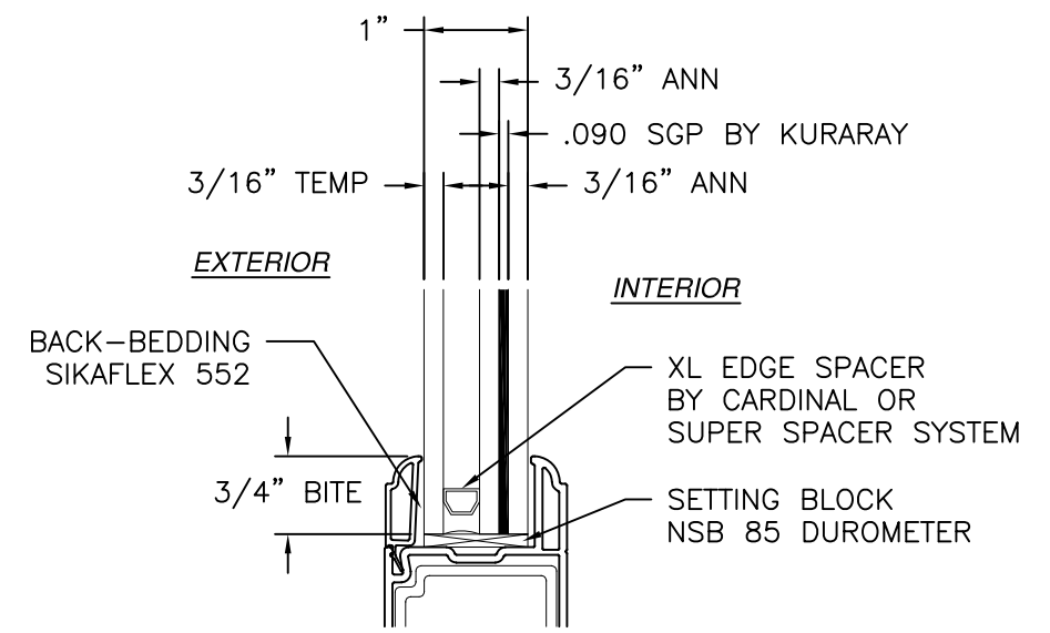
GLAZING DETAIL 1
