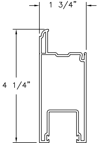
SASH FRAME (10001170) PVC (.075" THICK)
