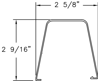
ASTRAGAL COVER (10001101) PVC (.060" THICK)
