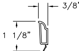
GLAZING BEAD (10001175) PVC (.075" THICK)
