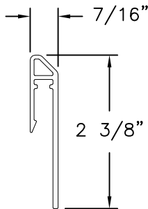
SILL RISER (10300323) ALUMINUM 6063-T5 (.078" THICK)
