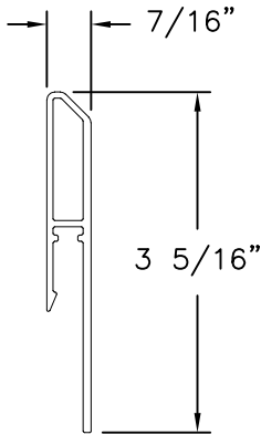
SILL RISER (10300240) ALUMINUM 6063-T5 (.078" THICK)
