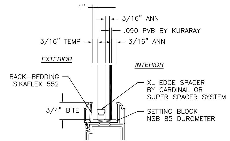
GLAZING DETAIL 2
