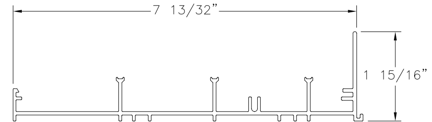
FRAME SILL 3TRACK ALUMINUM 6063-T6 BY SAPA (3291)
