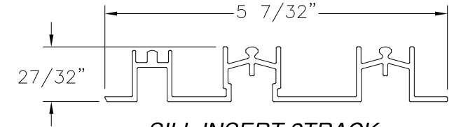
SILL INSERT 2TRACK ALUMINUM 6063-T6 BY SAPA (3288)
