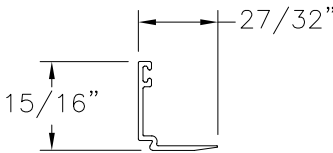
GLAZING BEAD ALUMINUM 6063-T6 BY SAPA (57278)
