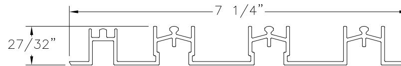
SILL INSERT 3TRACK ALUMINUM 6063-T6 BY SAPA (3288)
