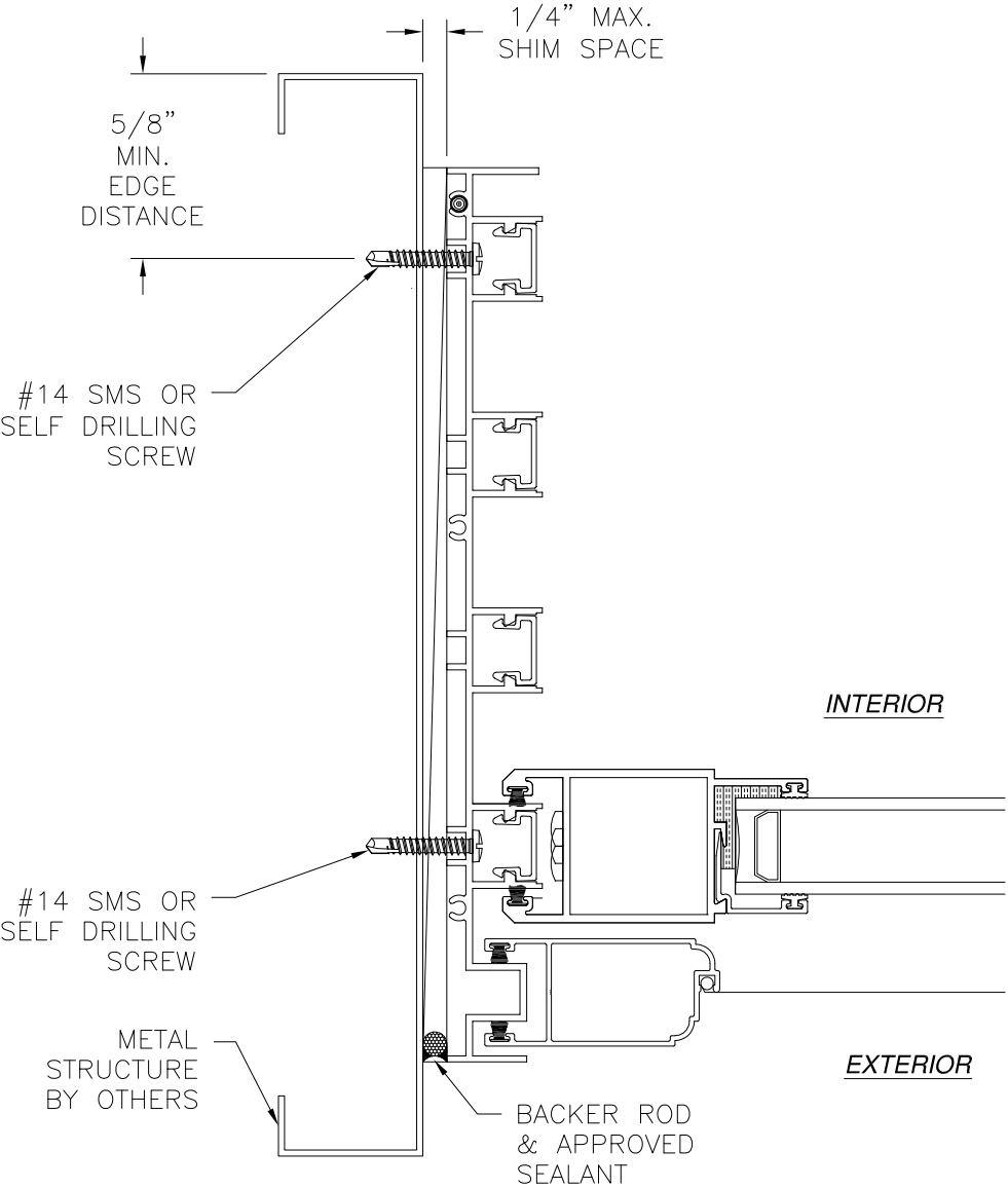
JAMB INSTALLATION DETAIL METAL STRUCTURE INSTALLATION SIGNED: 01/05/2026
