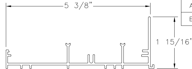
FRAME SILL 2TRACK ALUMINUM 6063-T6 BY SAPA (3291)
