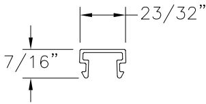
ANCHOR COVER ALUMINUM 6063-T6 BY SAPA (57398)
