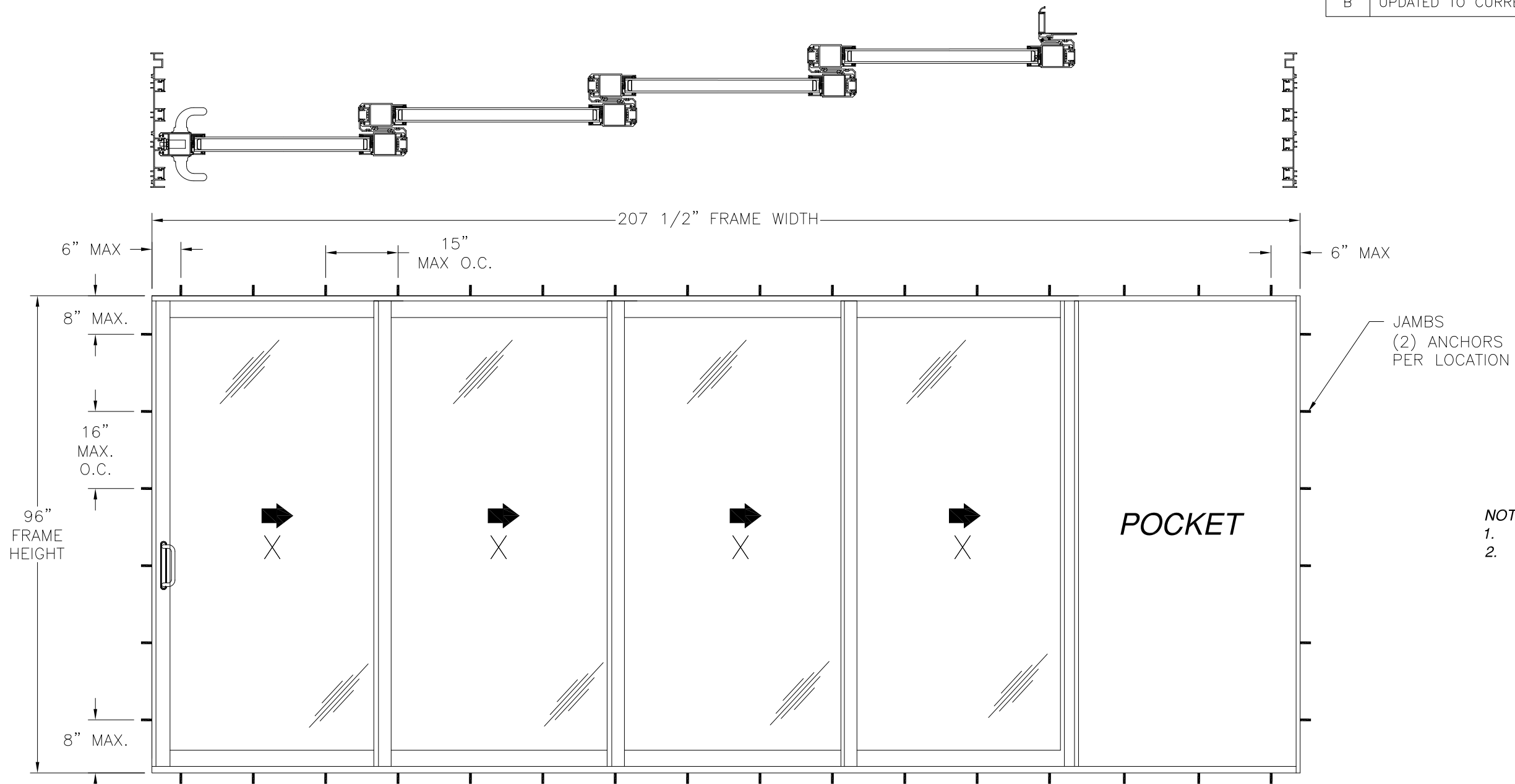
SERIES 7000 ALUMINUM SLIDING GLASS DOOR EXTERIOR VIEW
