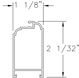
INTERLOCK SCREEN STILE ALUMINUM 6063-T6 BY SAPA (GAH-49197)
