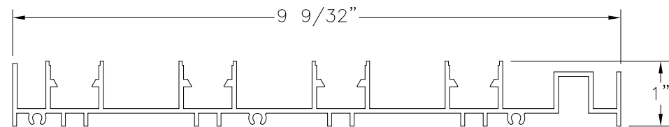
FRAME JAMB 4TRACK ALUMINUM 6063-T6 BY SAPA (57336)
