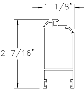
SCREEN LOCK STILE ALUMINUM 6063-T6 BY SAPA (GAH-49298)
