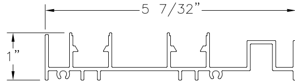
FRAME JAMB 2TRACK ALUMINUM 6063-T6 BY SAPA (57336)
