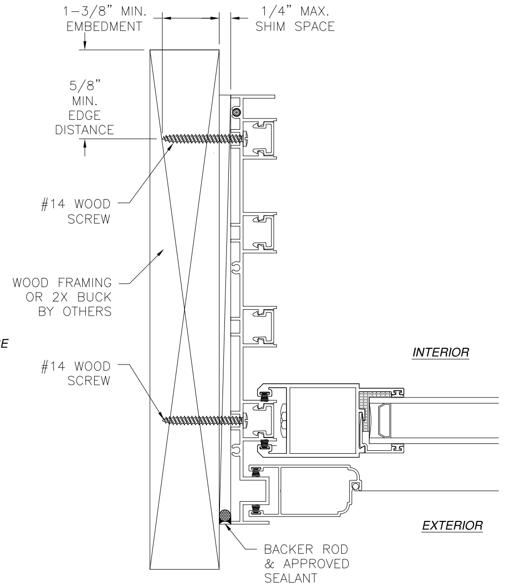
JAMB INSTALLATION DETAIL WOOD FRAMING OR 2X BUCK INSTALLATION SIGNED: 01/05/2026
