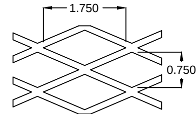
7 STD. BIRD SCREEN
