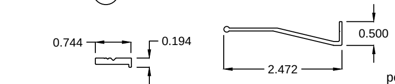
4 BIRD SCREEN FRAME
