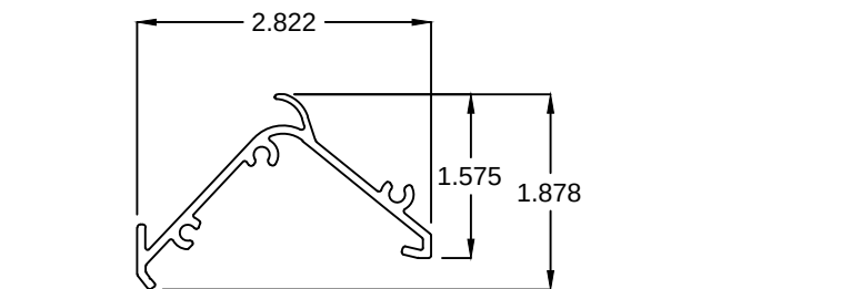
5 BLADE (Horizontal & Vertical)
