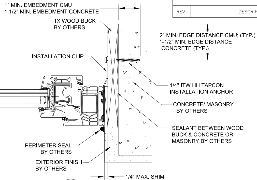
D 5 HORIZONTAL SECTION CONCRETE/MASONRY SUBSTRATE INSTALLATION CLIP
