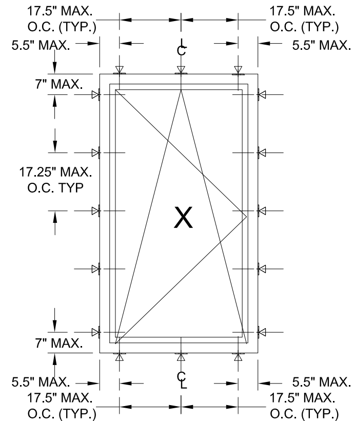
ANCHOR LAYOUT THROUGH FRAME & STRAP ANCHOR INSTALLATION
