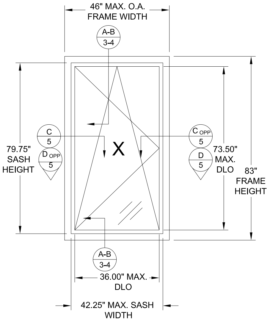
SERIES 76 MD VINYL BALCONY DOOR ELEVATION VIEW INTERIOR VIEW
