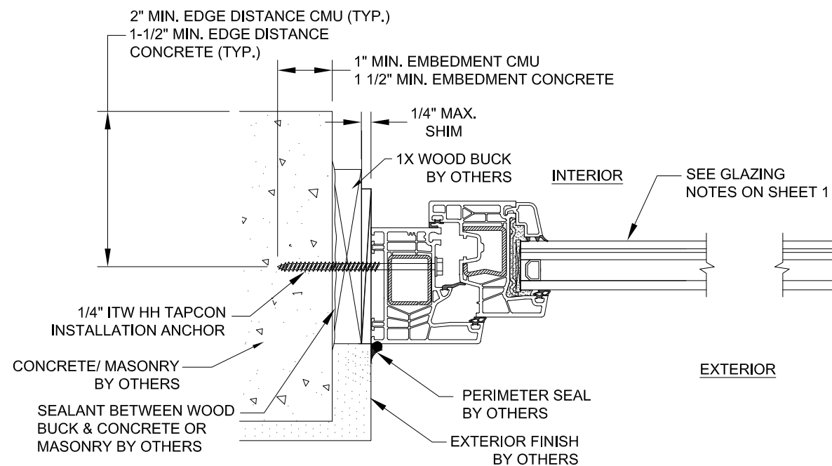
C 5 HORIZONTAL SECTION CONCRETE/MASONRY SUBSTRATE FRAME INSTALLATION
