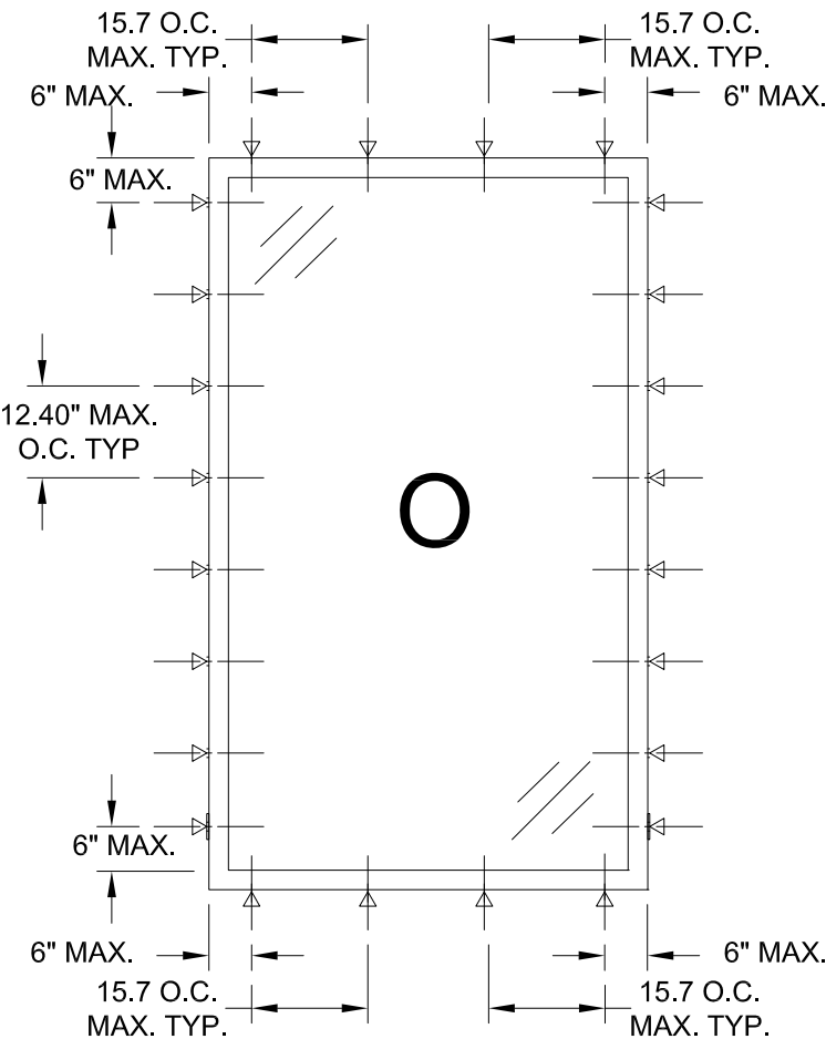
ANCHOR LAYOUT INTERIOR VIEW INSTALLATION THROUGH FRAME
