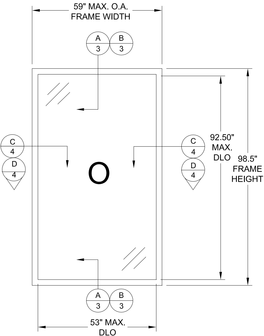
SERIES 76 MD VINYL P.W. ELEVATION VIEW INTERIOR VIEW
