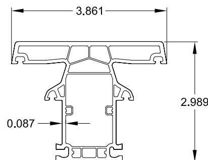
12 INTEGRAL ASTRAGAL STILE RIGID VINYL -76372-1
