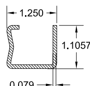
8 SASH REINFORCEMENT GALV. STL. 0.079" THICK V308
