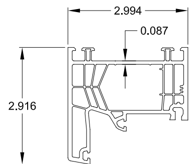
1 76171 MAIN FRAME EQUAL LEG RIGID VINYL
