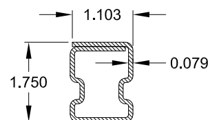
13 ASTRAGAL REINFORCEMENT GALV. STL. 0.079" THICK V319
