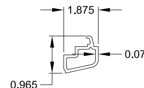
3 2435 2 32MM GLAZING BEAD RIGID VINYL
