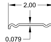
9 SASH GLAZING REINFORCEMENT GALV. STL. 0.079" THICK - V280
