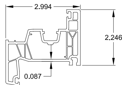
2 76271 MAIN SASH EQUAL LEG RIGID VINYL
