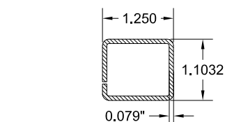
7 FRAME REINFORCEMENT GALV. STL. 0.079" THICK V310
