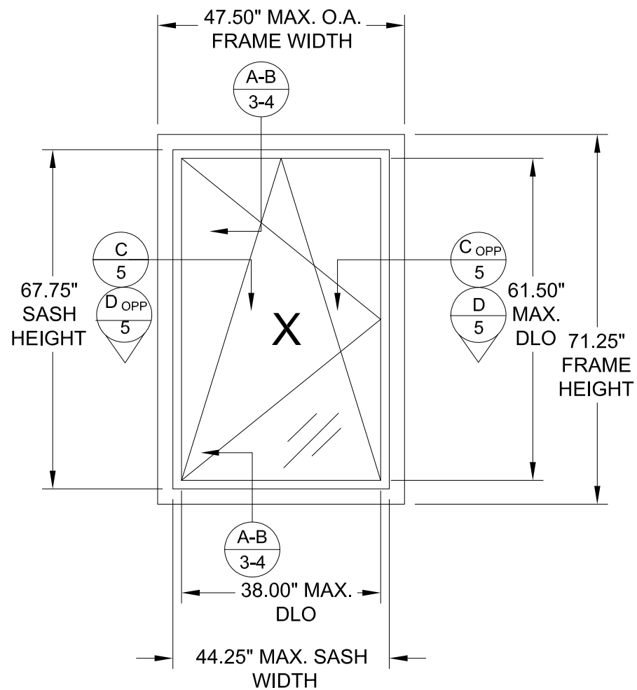
SERIES 76 MD VINYL TILT-TURN ELEVATION VIEW INTERIOR VIEW
