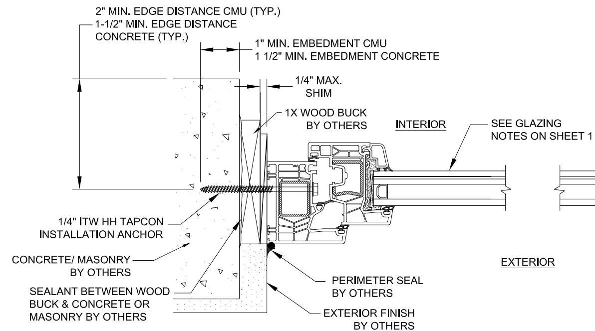
C 5 HORIZONTAL SECTION CONCRETE/MASONRY SUBSTRATE FRAME INSTALLATION
