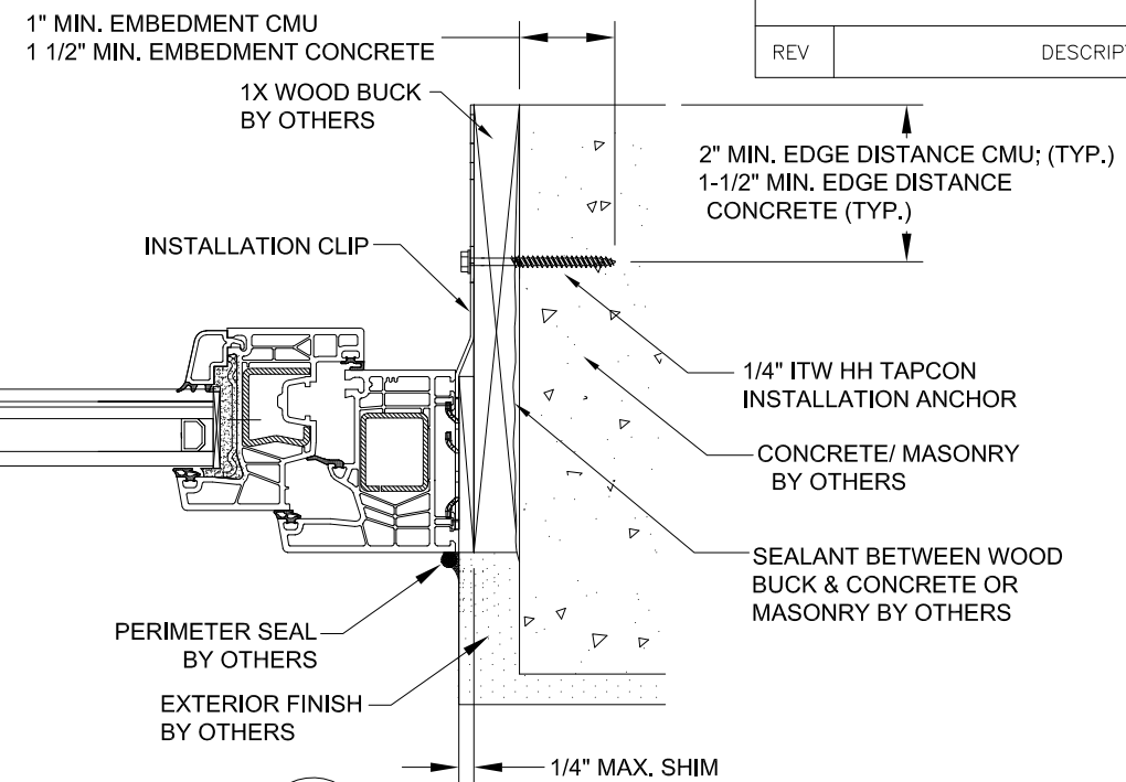
D 5 HORIZONTAL SECTION CONCRETE/MASONRY SUBSTRATE INSTALLATION CLIP
