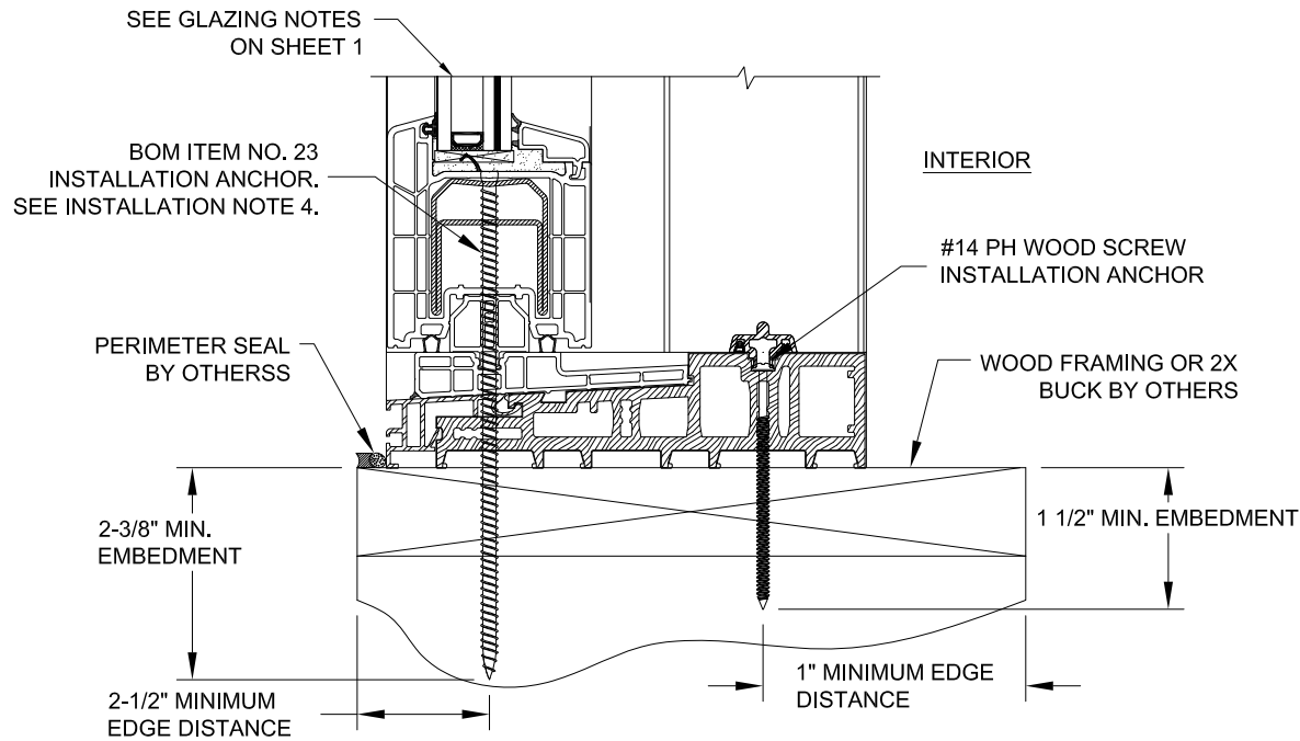
F 5 VERTICAL SECTION WOOD FRAMING OR 2 X BUCK INSTALLATION STATIONARY PANEL
