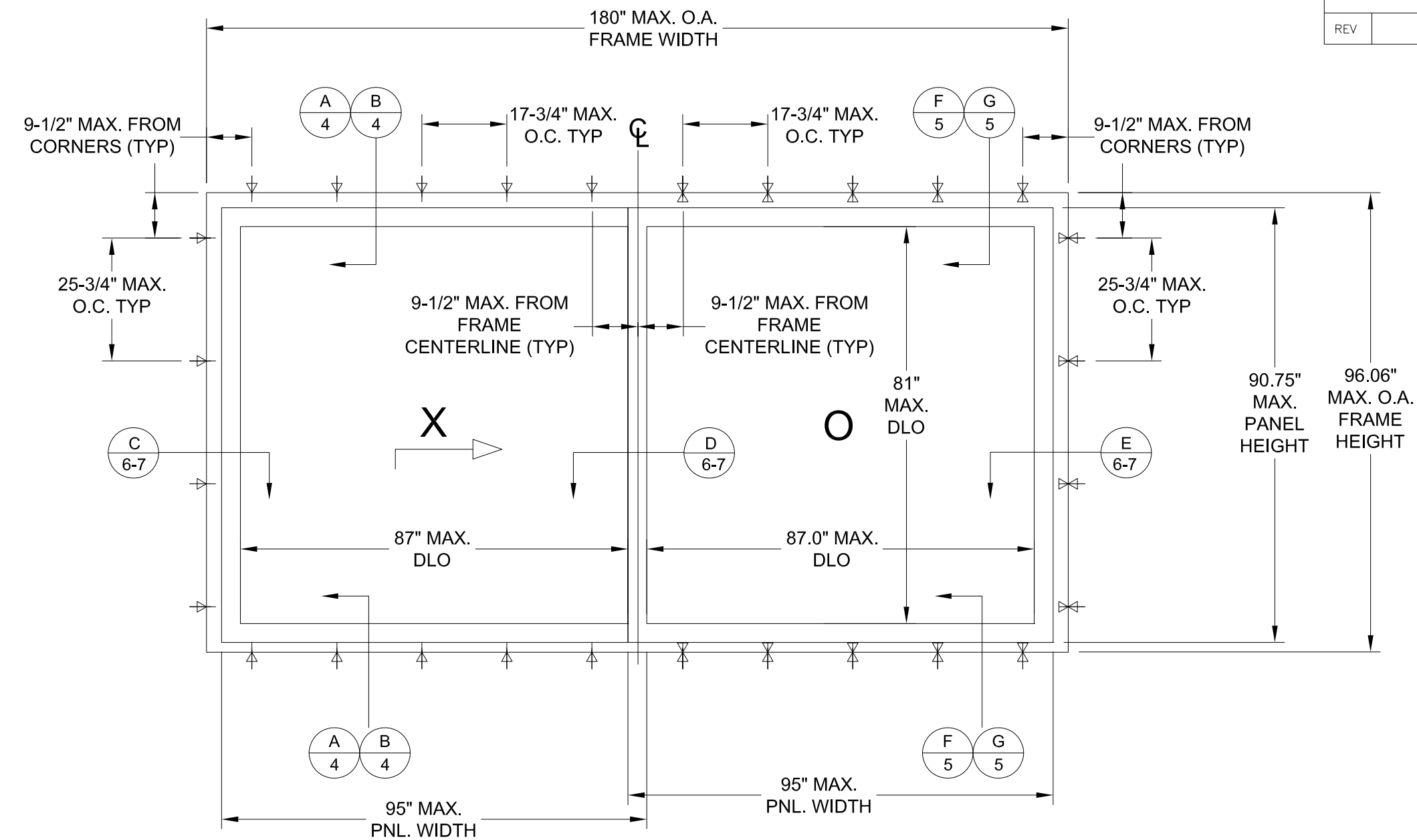
ELEVATION & ANCHOR DETAIL EXTERIOR VIEW
