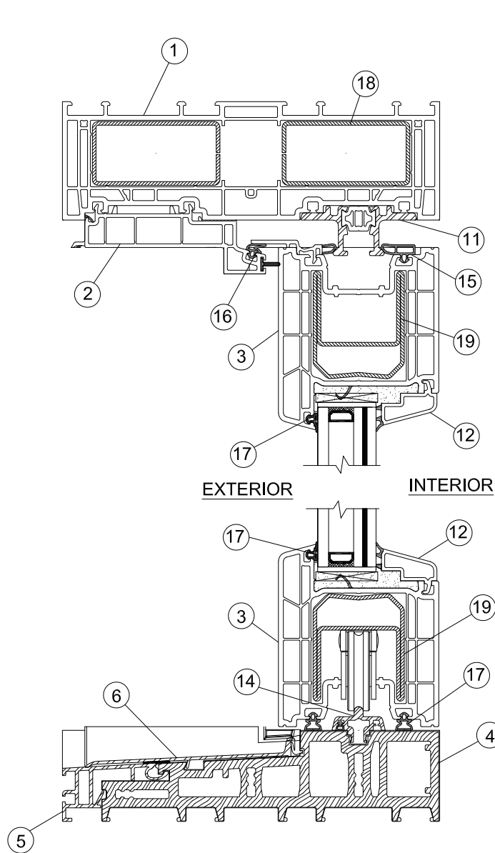
VERTICAL CROSS SECTION FOR PARTS IDENTIFICATION
