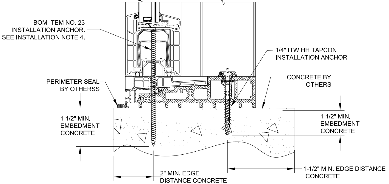
G 5 VERTICAL SECTION CONCRETE INSTALLATION STATIONARY PANEL
