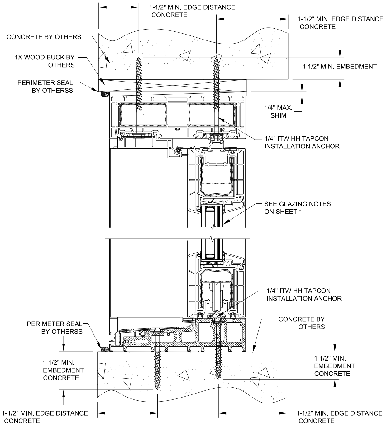
B 4 VERTICAL SECTION CONCRETE INSTALLATION OPERABLE PANEL
