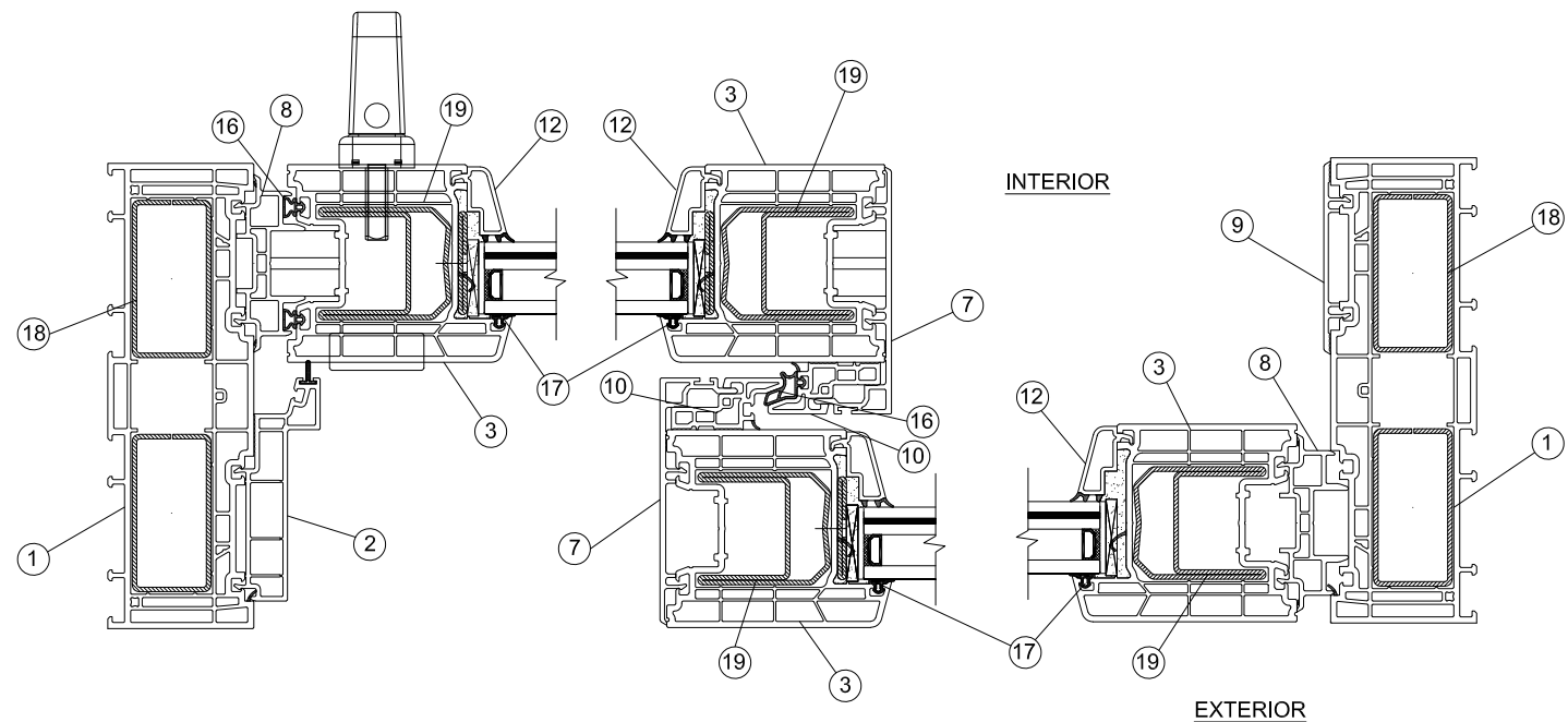
HORIZONTAL CROSS SECTION FOR PARTS IDENTIFICATION
