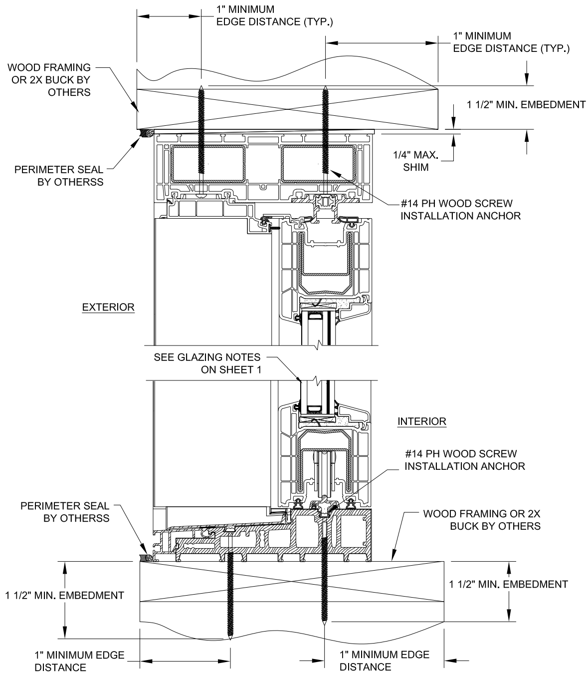
A 4 VERTICAL SECTION WOOD FRAMING OR 2 X BUCK INSTALLATION OPERABLE PANEL
