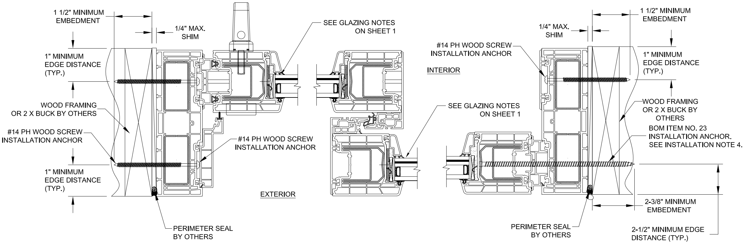
D 6 INTERLOCK SECTION
