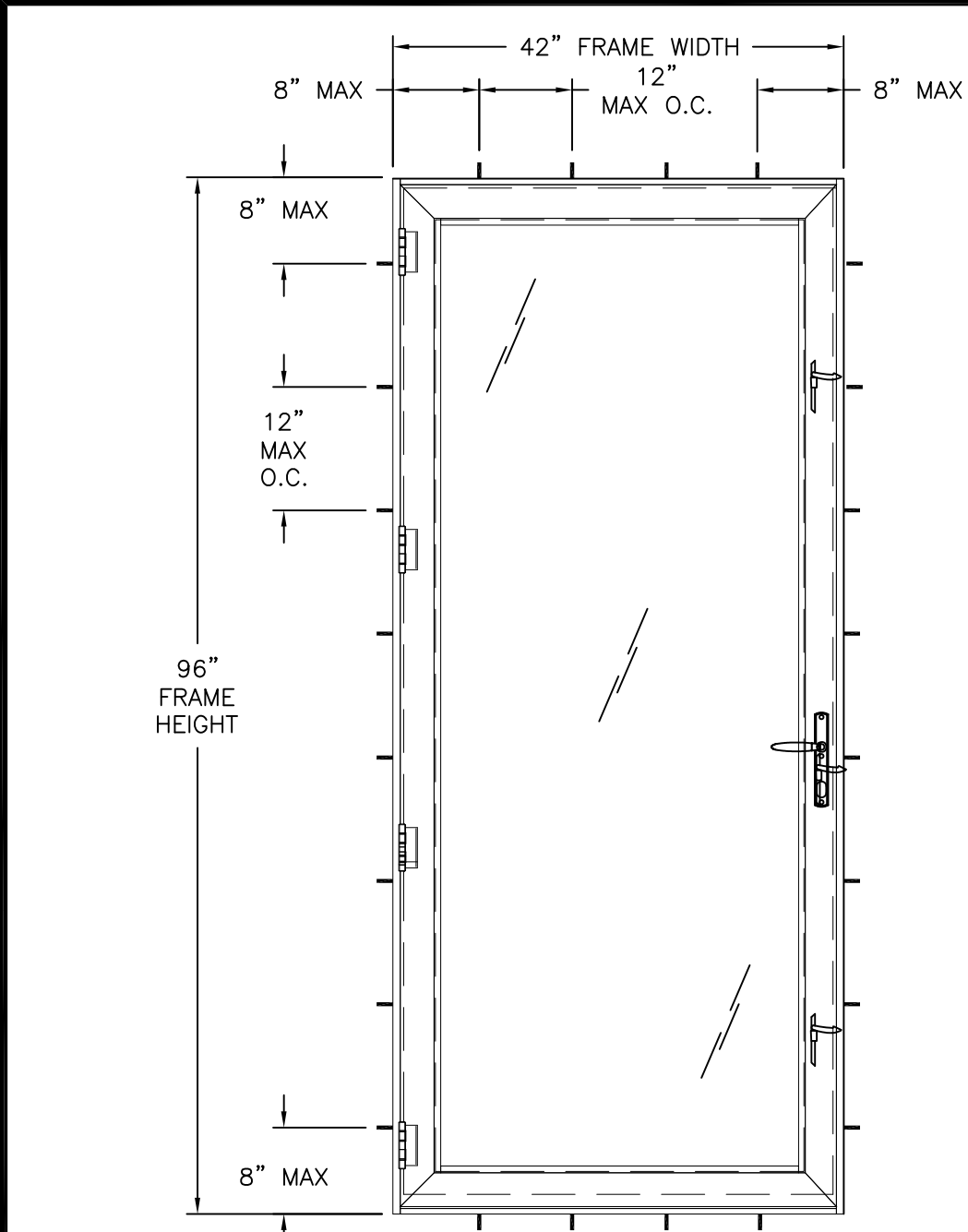
D900 ALUMINUM TERRACE DOOR EXTERIOR VIEW
