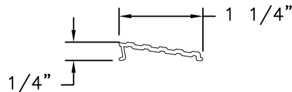
THRESHOLD SNAP COVER TH426 ALUMINUM 6063-T5
