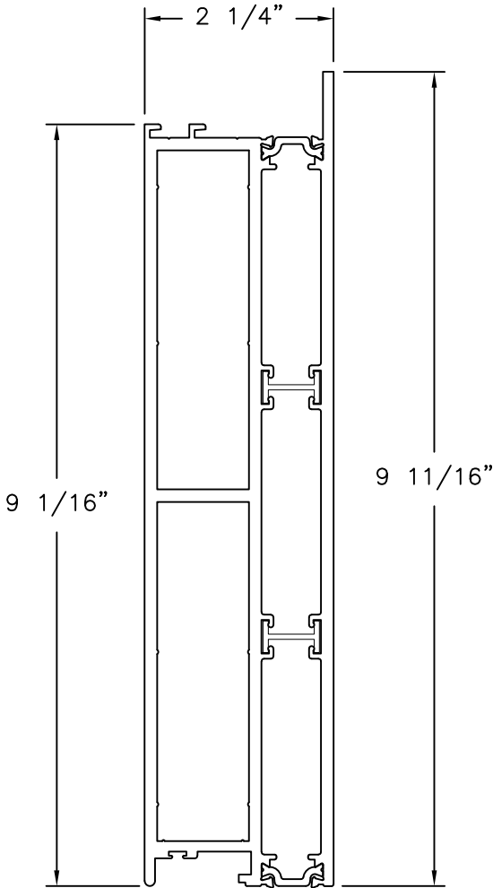
10" BOTTOM RAIL WT900 ALUMINUM 6063-T5
