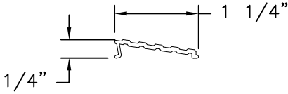
THRESHOLD SNAP COVER TH426 ALUMINUM 6063-T5
