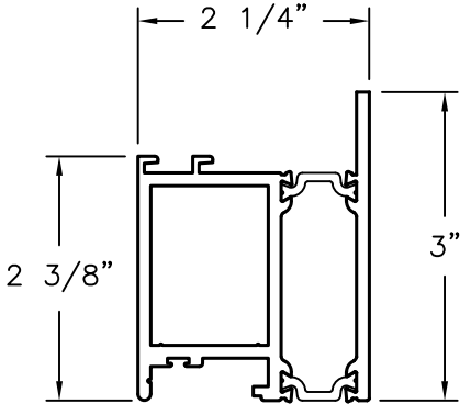
STANDARD BOTTOM RAIL HT301 ALUMINUM 6063-T5
