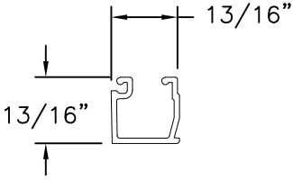
GLASS STOP WN429 ALUMINUM 6063-T5
