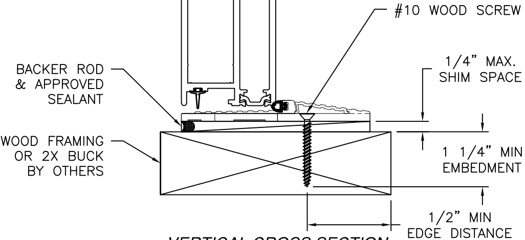
VERTICAL CROSS SECTION WOOD FRAMING OR 2X BUCK INSTALLATION 10" BOTTOM RAIL SHOWN, STANDARD RAIL SIMILAR
