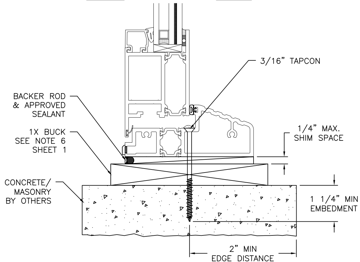
VERTICAL CROSS SECTION CONCRETE/MASONRY INSTALLATION WITH 1X BUCK INSTALLATION FOR CONCRETE/MASONRY WITHOUT 1X BUCK REFER TO JAMB INSTALLATION DETAILS
