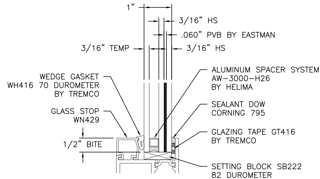
GLAZING DETAIL
