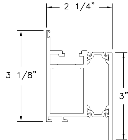
SASH MEMBER HT300 ALUMINUM 6063-T5
