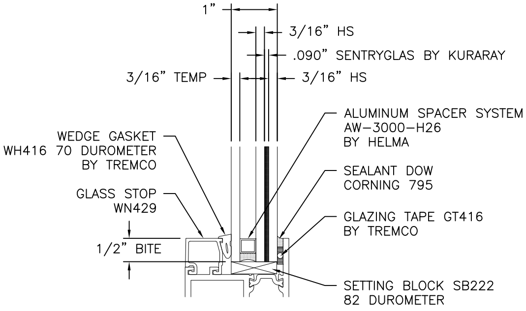
GLAZING DETAIL
