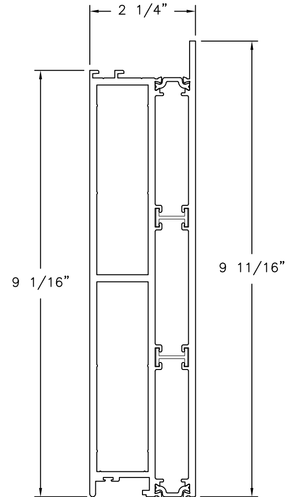
10" BOTTOM RAIL WT900 ALUMINUM 6063-T5
