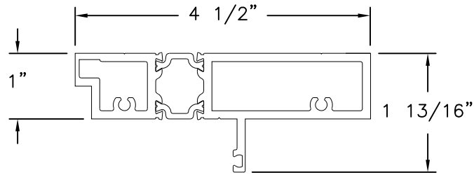
FRAME HEAD HT450 ALUMINUM 6063-T5
