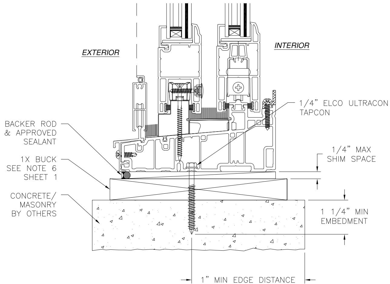
VERTICAL CROSS SECTION CONCRETE/MASONRY WITH 1X BUCK INSTALLATION FOR CONCRETE/MASONRY WITHOUT 1X BUCK REFER TO JAMB INSTALLATION DETAIL
