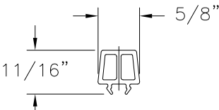
OUT. BEAD WELDED SASH TANDEM WHEEL SHIM (7541) RIGID PVC
