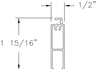
SCREEN ALUMINUM
