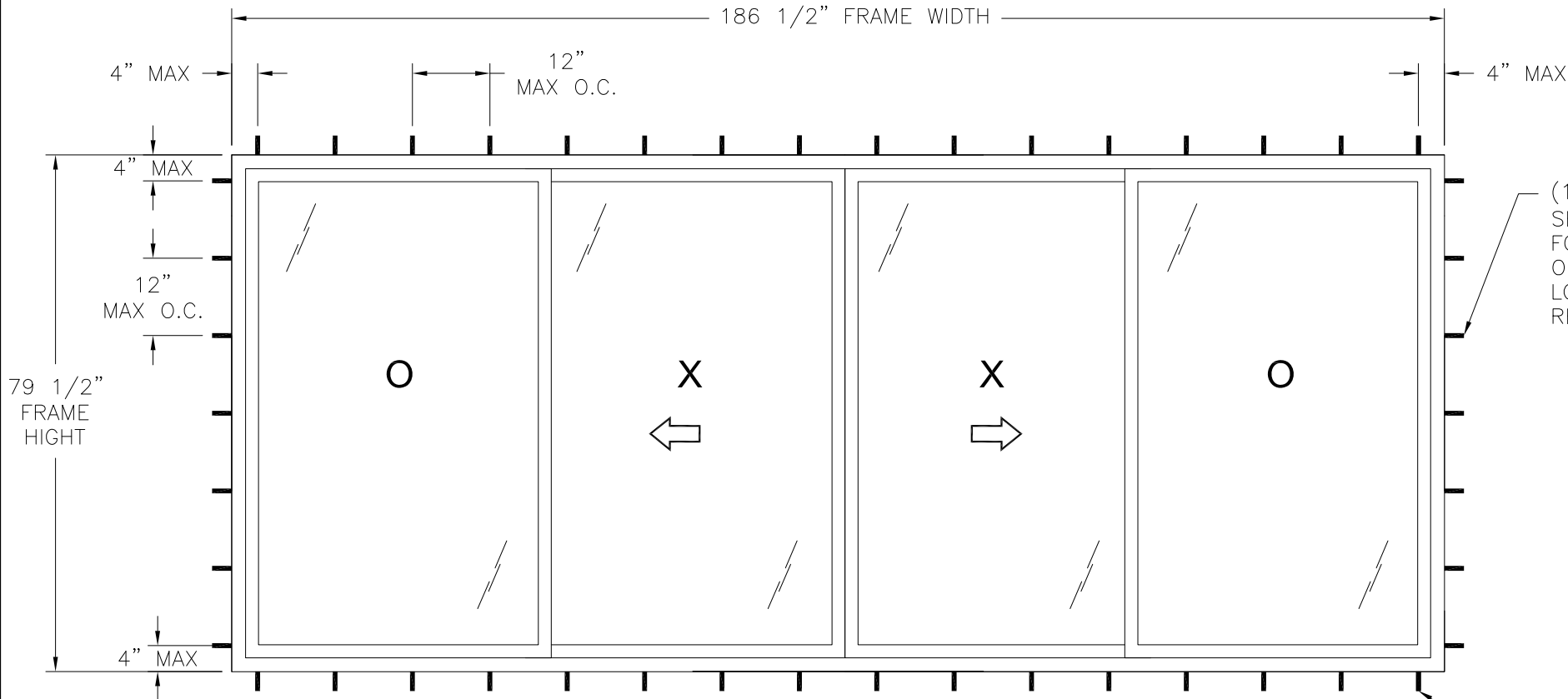
SERIES 1615/1617 PVC SLIDING GLASS DOOR NON - IMPACT EXTERIOR VIEW
