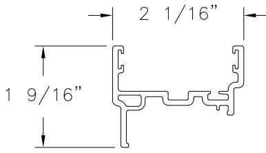
MULLION (7005) RIGID PVC
