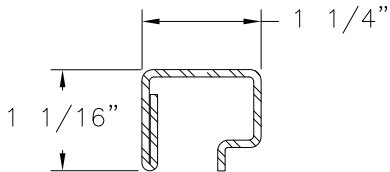
CENTER STILE REINFORCEMENT (9599) STEEL
