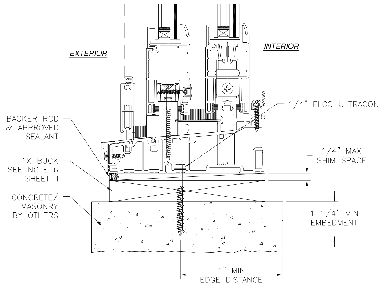
VERTICAL CROSS SECTION CONCRETE MASONRY 1X INSTALLATION
