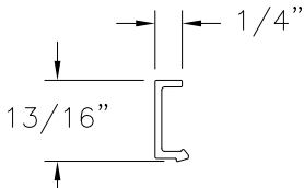
GLAZING BEAD EXTRUDED RIGID PVC
