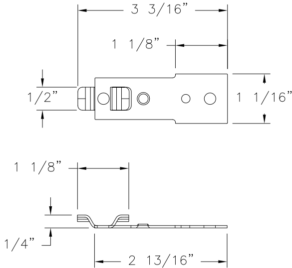
CLIP GALVANIZED STEEL (.051" THICK)
