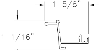
SILL CLADDING (9991) ALUMINUM
