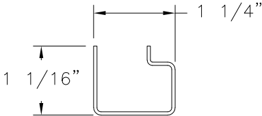
STILE REINFORCEMENT (9598) STEEL
