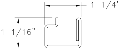
STILE REINFORCEMENT (9599) STEEL
