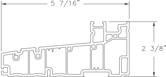
SILL (7000) RIGID PVC
