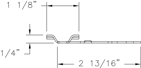
CLIP GALVANIZED STEEL (.051" THICK)
