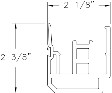
INTERLOCK (7026) RIGID PVC
