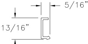
GLAZING BEAD (5775, -70, -71, 72) RIGID PVC
