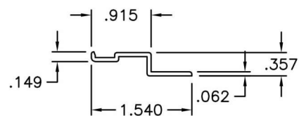
FIX. PANEL CLIP
