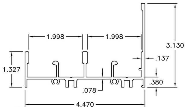
FRAME SILL
