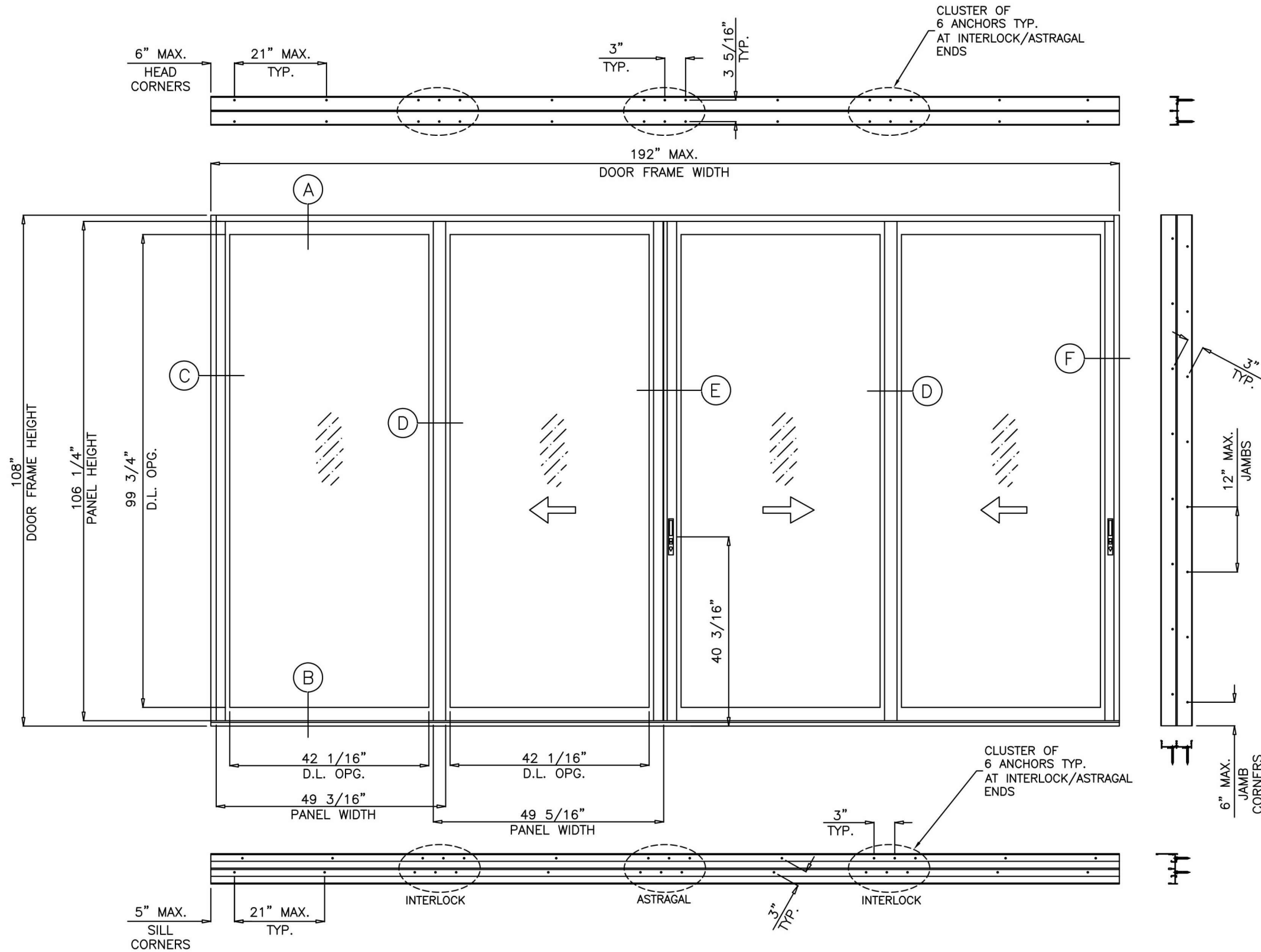
TYPICAL ELEVATION OXXX
