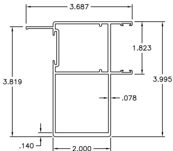
PANEL FEMALE ASTRAGAL
