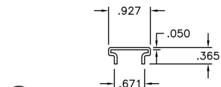
FRAME SILL COVER
