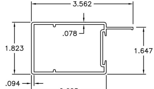
PANEL LOCK STILE
