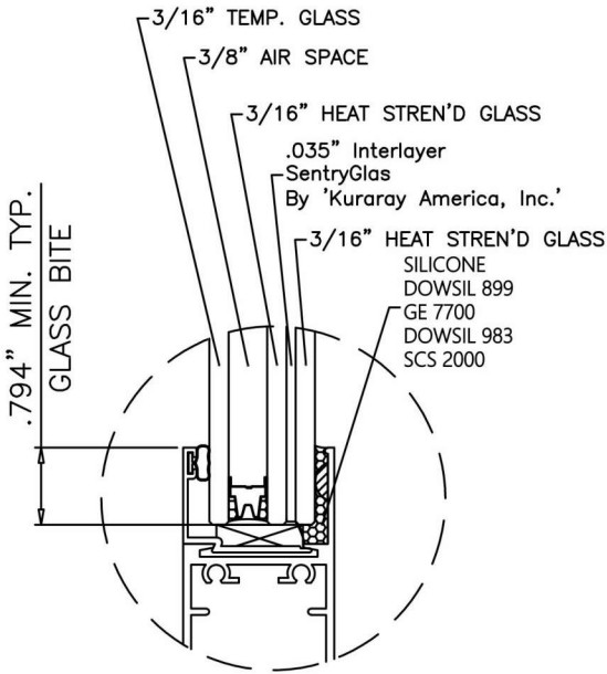
GLASS TYPE 'A1' 1" NOM. INSUL. LAM. GLASS
