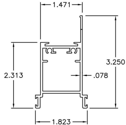
PANEL TOP & BOTTOM RAIL
