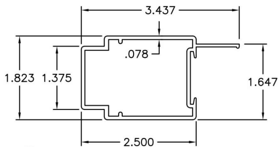
PANEL MALE ASTRAGAL
