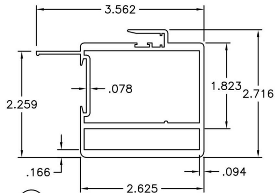
PANEL OUTER INTERLOCK
