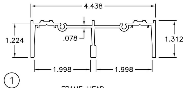
FRAME HEAD
