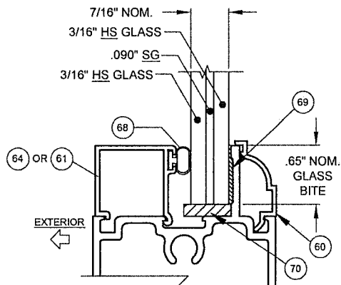
GLASS TYPE 7
