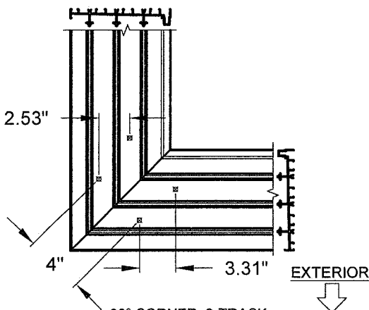
90° CORNER, 3-TRACK (USE WHERE 4 CLUSTER ANCHORS ARE REQUIRED, "C4")
