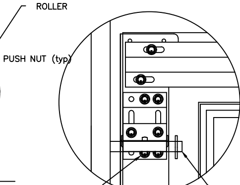
DETAIL F
