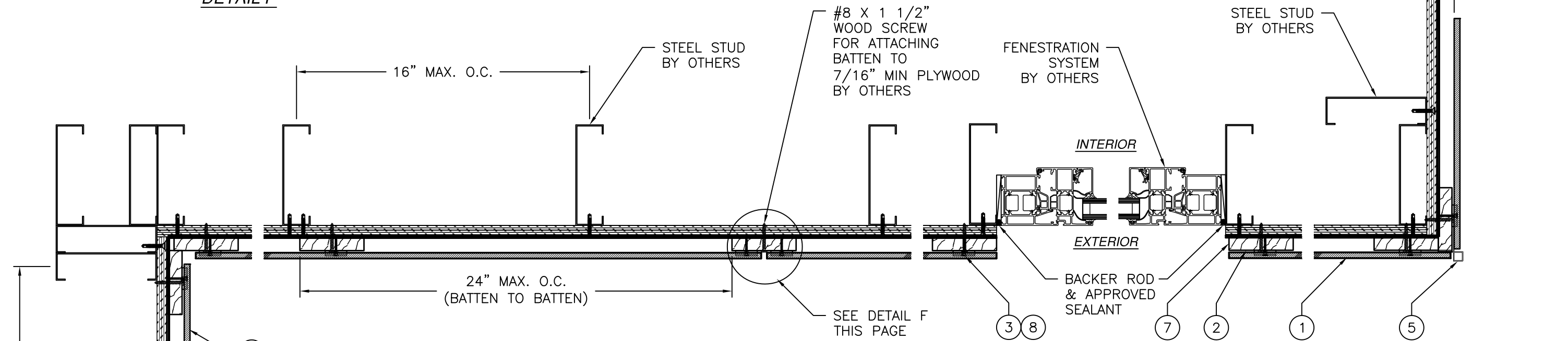
B 7 HORIZONTAL CROSS SECTION FLUSH SIDING INSTALLATION 7/16" MIN. PLYWOOD SHEATHING (METAL FRAME)
