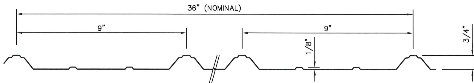
PANEL PROFILE
