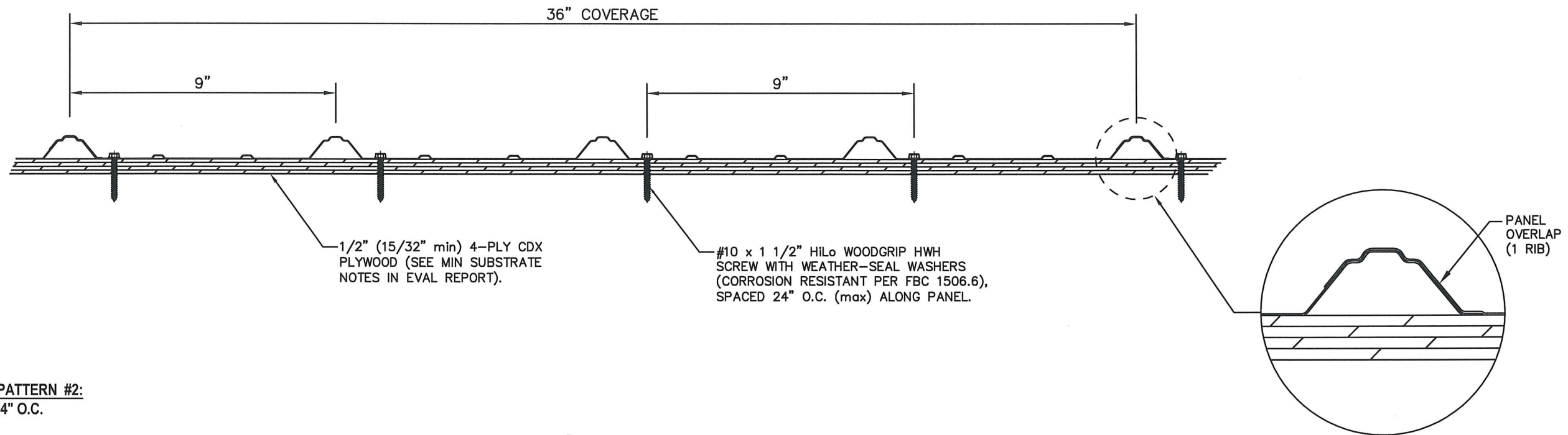
ANCHOR PATTERN #1: SPACED 24" O.C.
