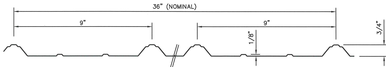
PANEL PROFILE
