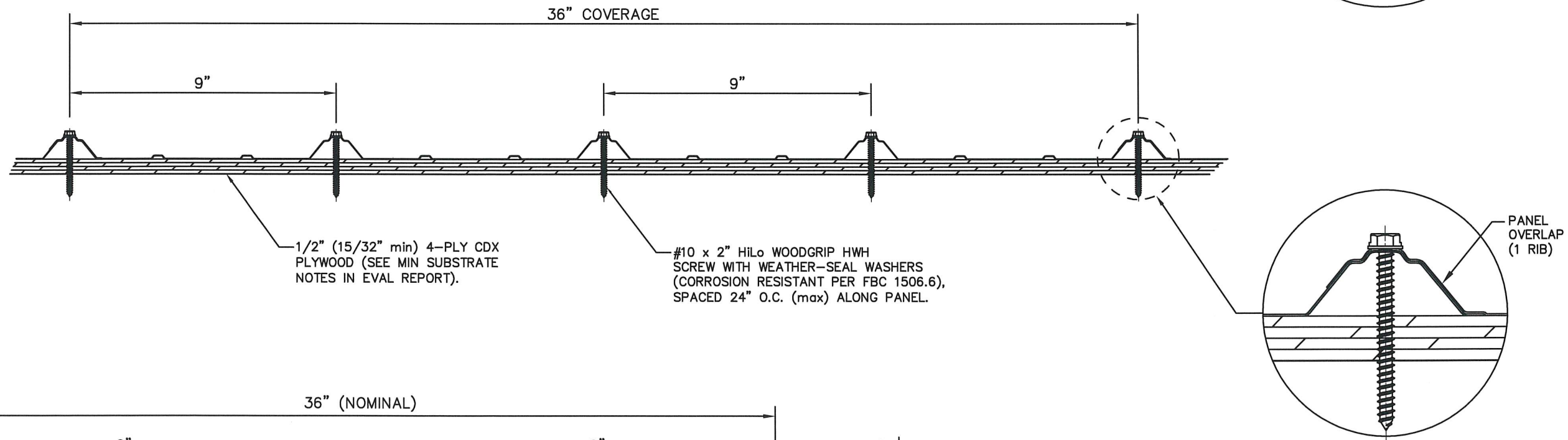
ANCHOR PATTERN #2: SPACED 24" O.C.
