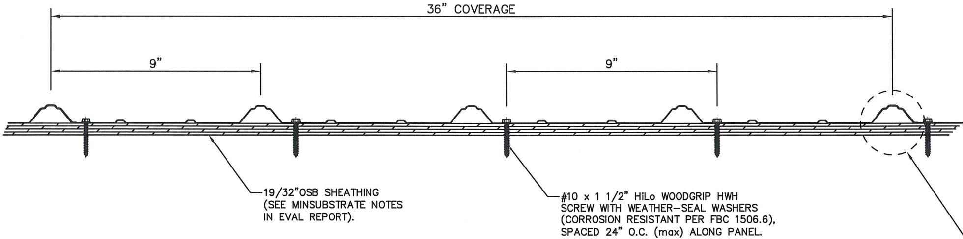
ANCHOR PATTERN #1: SPACED 24" O.C.
