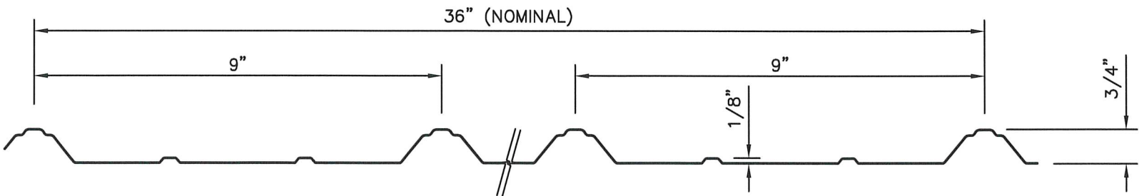
PANEL PROFILE
