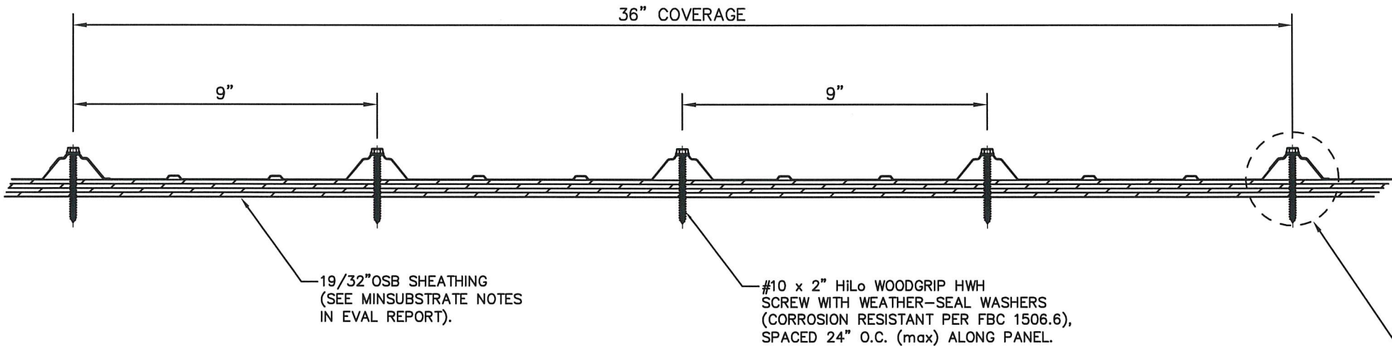
ANCHOR PATTERN #2: SPACED 24" O.C.
