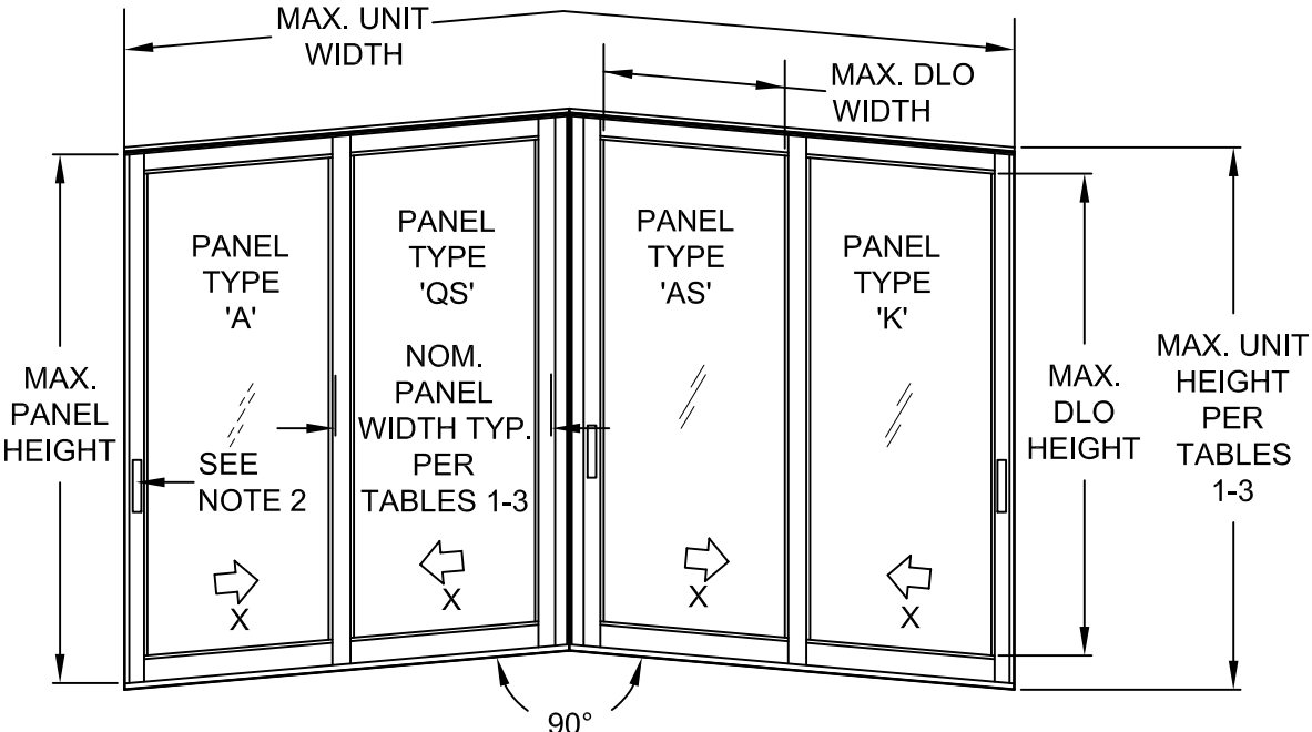
EXAMPLE: 90° INSIDE CORNER, 4 PANELS - XX/XX
