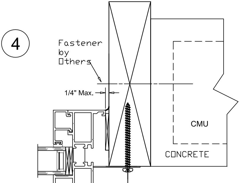
See sheet #2 for Nail Fin Install
