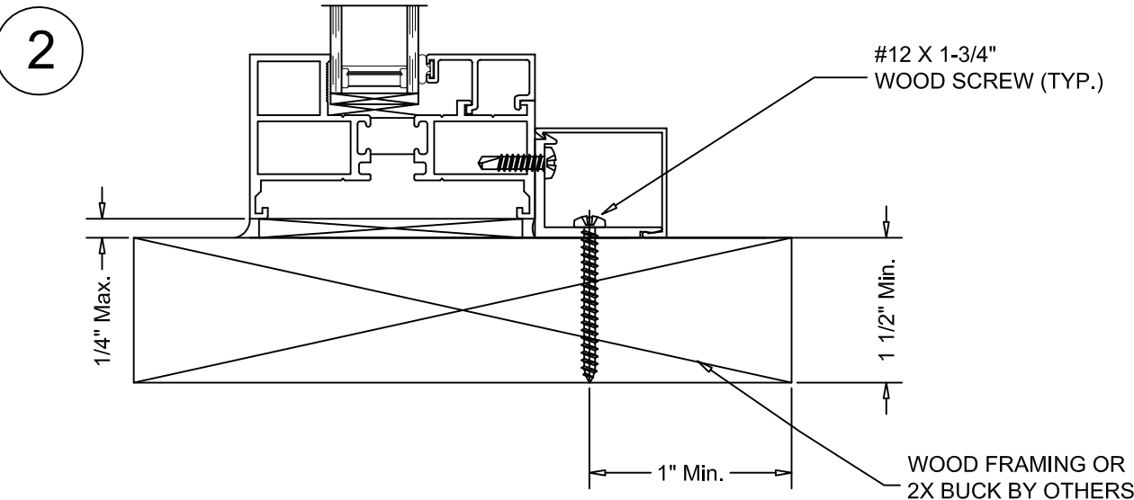
VERTICAL SECTION DETAIL
