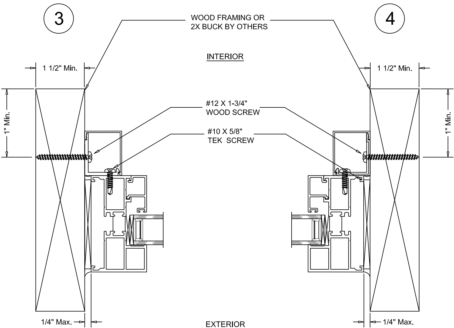
HORIZONTAL SECTION DETAIL
