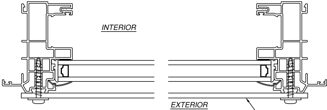
HORIZONTAL CROSS SECTION FRAME INSTALLATION WITH IMPACT PROTECTIVE SYSTEM (REFERENCE ONLY) HORIZONTAL INSTALLATION SHOWN, VERTICAL INSTALLATION SIMILAR
