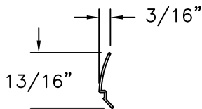
GLAZING BEAD
