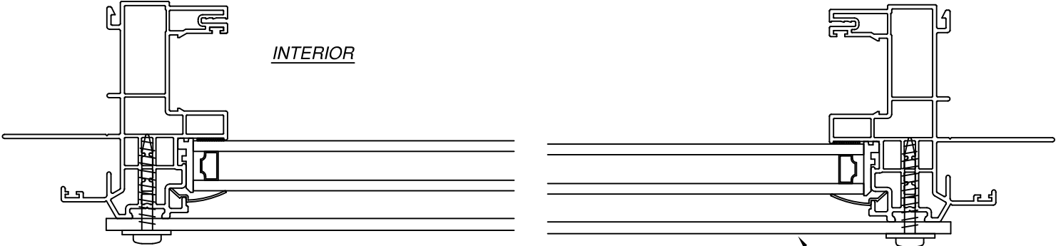
HORIZONTAL CROSS SECTION FIN INSTALLATION WITH J-CHANNEL WITH IMPACT PROTECTIVE SYSTEM (REFERENCE ONLY) HORIZONTAL INSTALLATION SHOWN, VERTICAL INSTALLATION SIMILAR
