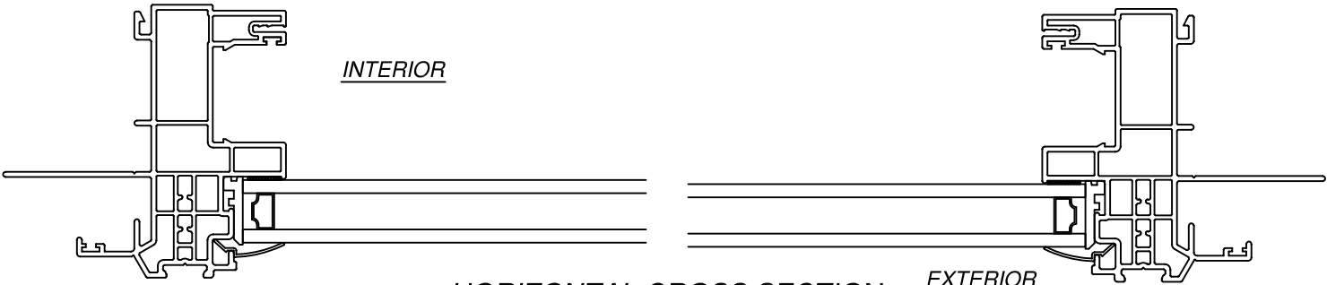
HORIZONTAL CROSS SECTION FIN INSTALLATION WITH J-CHANNEL
