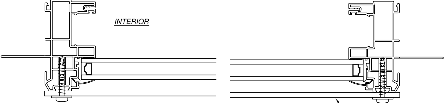
HORIZONTAL CROSS SECTION FIN INSTALLATION WITHOUT J-CHANNEL WITH IMPACT PROTECTIVE SYSTEM (REFERENCE ONLY) HORIZONTAL INSTALLATION SHOWN, VERTICAL INSTALLATION SIMILAR
