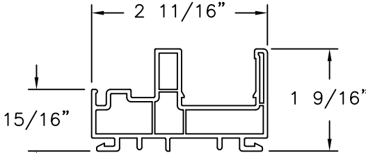
MAIN FRAME
