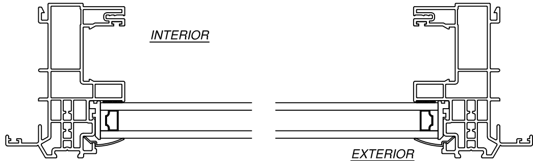
HORIZONTAL CROSS SECTION FRAME INSTALLATION
