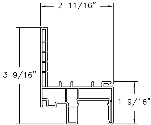
MAIN FRAME WITH FLANGE
