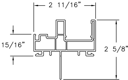
MAIN FRAME FIN INSTALLATION
