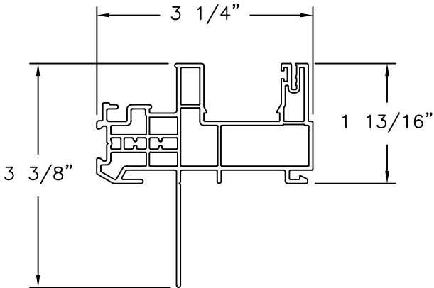
STORM JAMB WITHOUT J-CHANNEL FIN INSTALLATION
