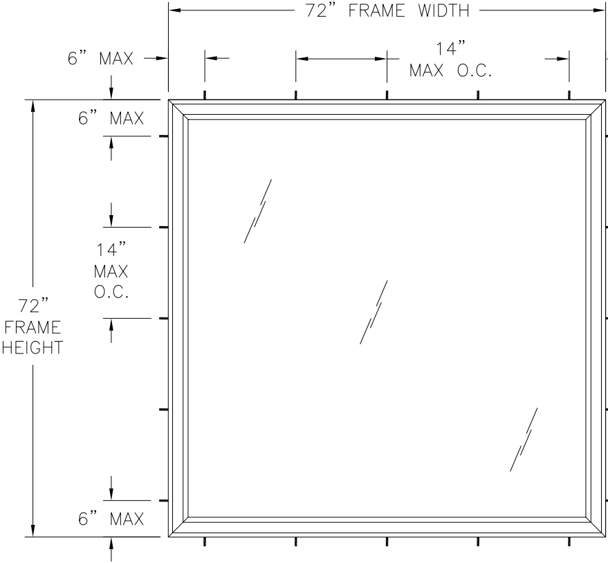
1970 FIXED WINDOW EXTERIOR VIEW FRAME INSTALLATION
