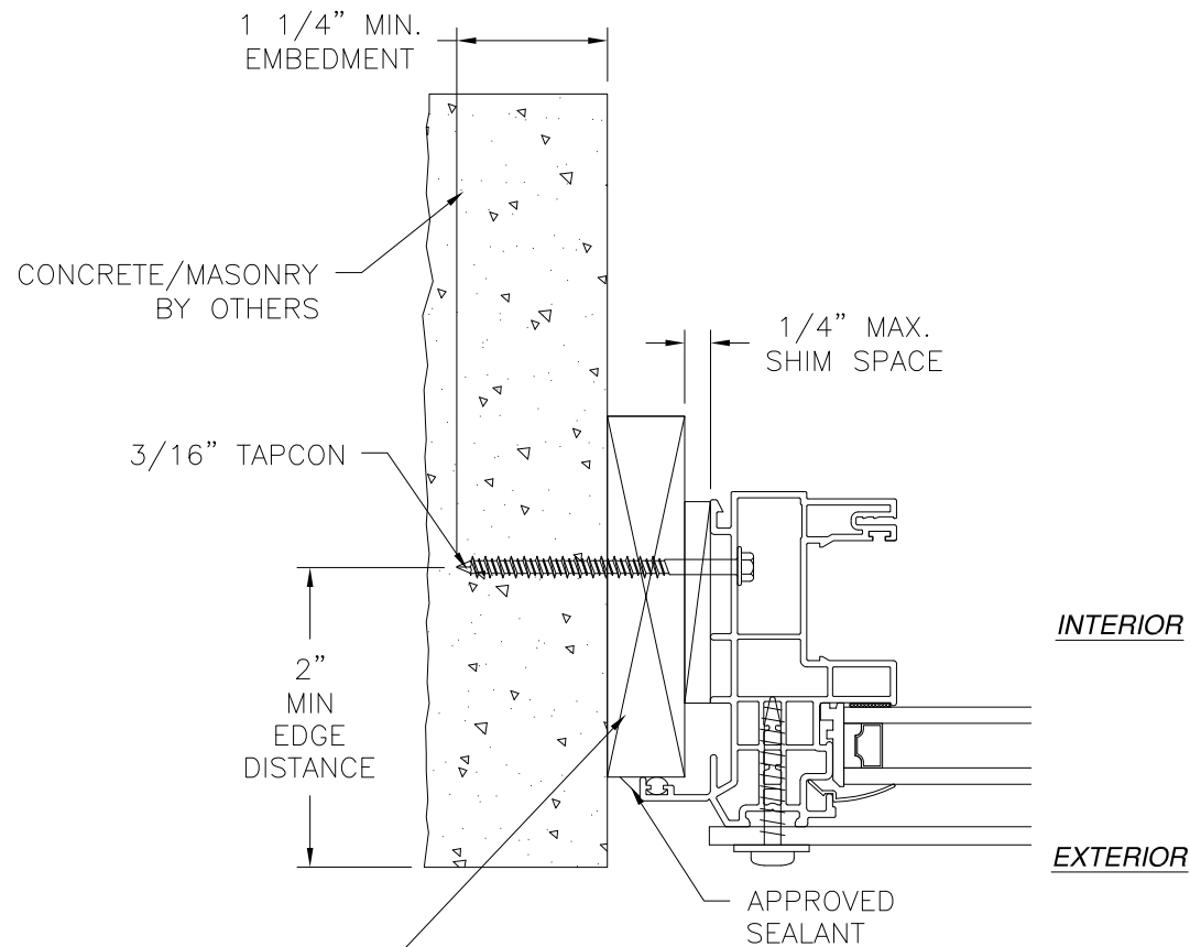
JAMB INSTALLATION DETAIL CONCRETE/MASONRY W/1X BUCK INSTALLATION
