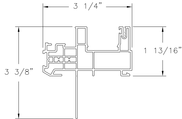
STORM JAMB WITHOUT J-CHANNEL FIN INSTALLATION PVC (CL-2930)
