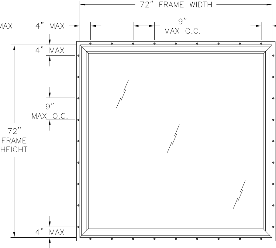
1970 FIXED WINDOW EXTERIOR VIEW FIN INSTALLATION WITH ROOFING NAILS
