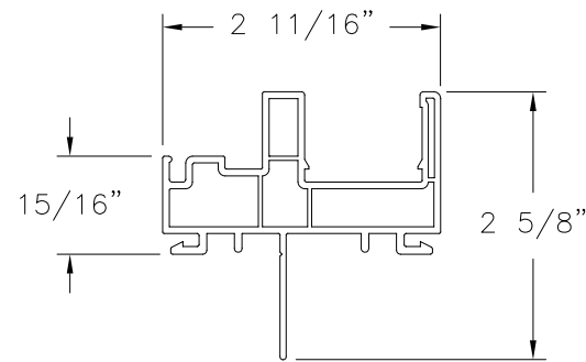
MAIN FRAME FIN INSTALLATION PVC (606004)
