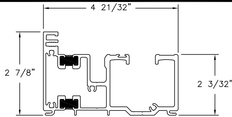
HEAD FRAME ALUMINUM 6063-T5
