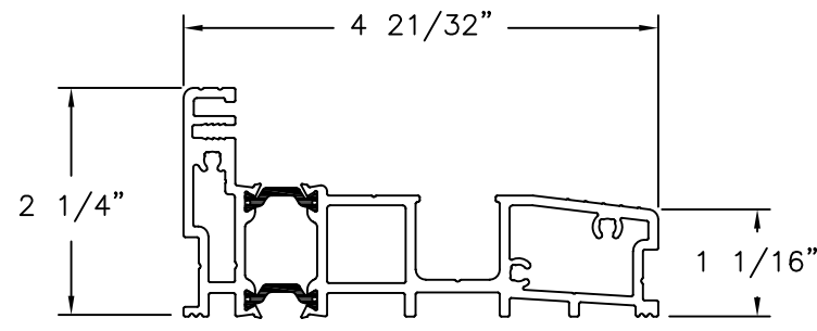
STANDARD THRESHOLD ALUMINUM 6063-T5
