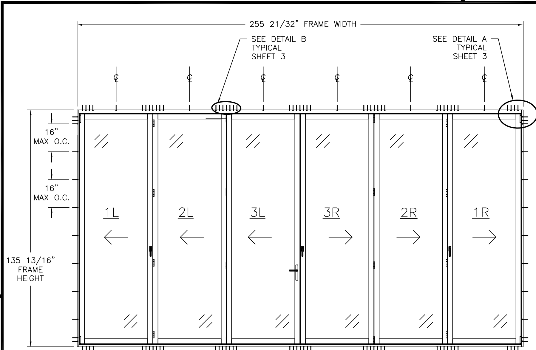
LANAI DOORS THERMALLY BROKEN ALUMINUM INSWING EXTERIOR VIEW
