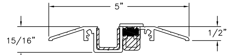
LOW RISE THRESHOLD ALUMINUM 6063-T5
