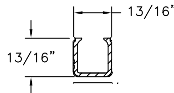
THRESHOLD INSERT RIGID PVC
