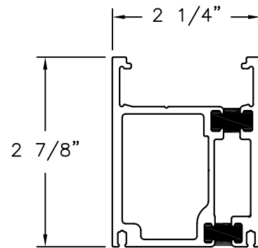
TOP/BOTTOM RAIL ALUMINUM 6063-T5
