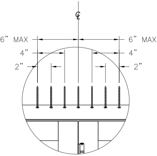
DETAIL B
