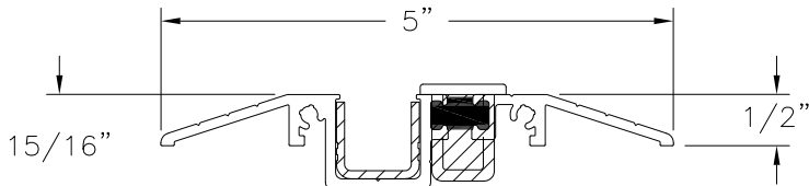
LOW RISE THRESHOLD ALUMINUM 6063-T5
