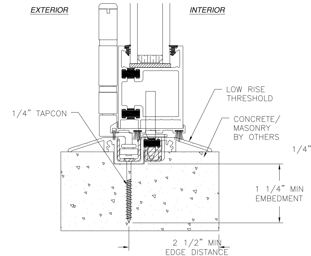
VERTICAL CROSS SECTION CONCRETE/MASONRY INSTALLATION LOW RISE THRESHOLD
