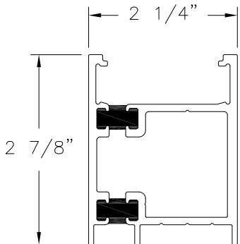
STILE ALUMINUM 6063-T5
