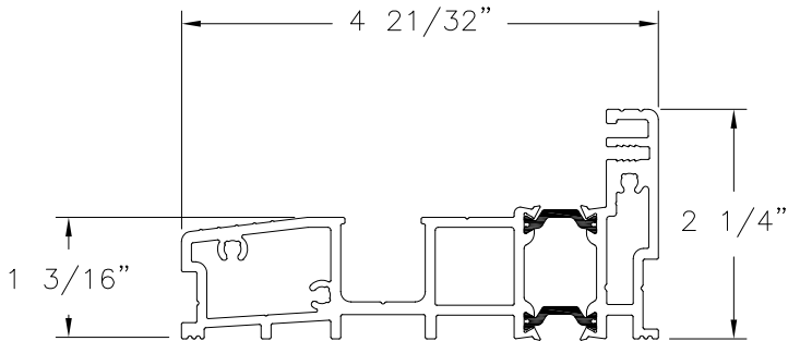
STANDARD THRESHOLD ALUMINUM 6063-T5
