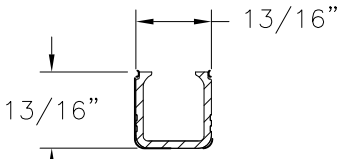
THRESHOLD INSERT RIGID PVC
