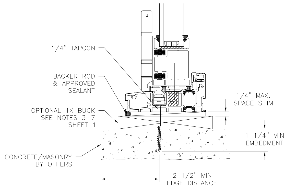
VERTICAL CROSS SECTION CONCRETE/MASONRY INSTALLATION STANDARD THRESHOLD SHOWN SEE SHEET 7 FOR OTHER THRESHOLDS INSTALLATION
