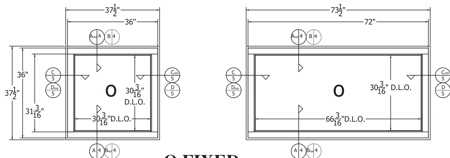
O FIXED TRANSOM WINDOWS ENVELOPED AND APPROVED UNITS
