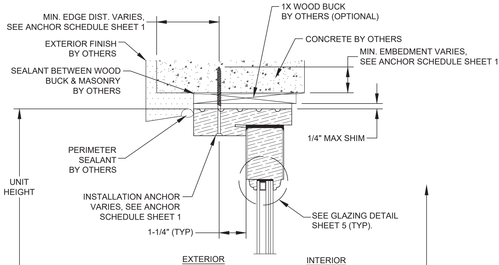
B VERTICAL SECTION CONCRETE SUBSTRATE INSTALLATION
