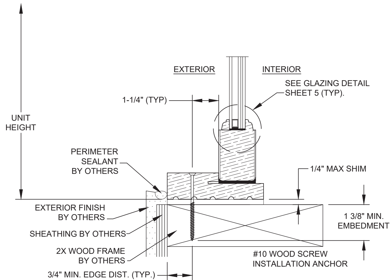
A VERTICAL SECTION 2X WOOD SUBSTRATE INSTALLATION
