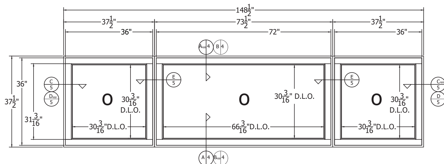
000 FIXED TRANSOM WINDOW TESTED AND APPROVED UNIT
