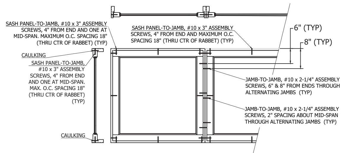
OO FIXED TRANSOM WINDOW ENVELOPED AND APPROVED UNIT
