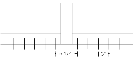
CONDITION 2 HEAD/SILL WITHOUT SUB BUCK (3/8" MAX SHIM)
