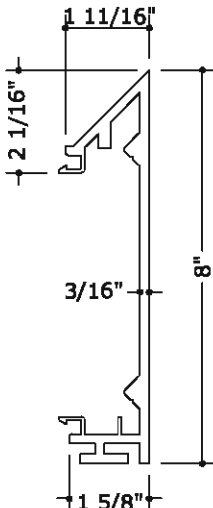
74 90° CORNER MULLION
