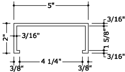
67 SUB-BUCK
