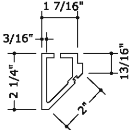
73 90° CORNER CAP ADAPTOR
