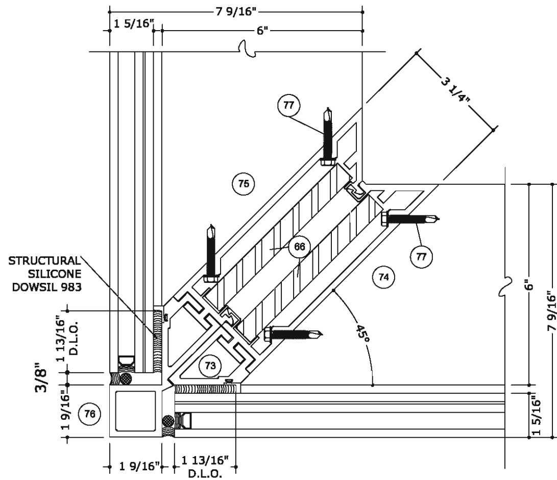
4 VERTICAL INTERMEDIATE DETAIL (REINFORCED) N.T.S
