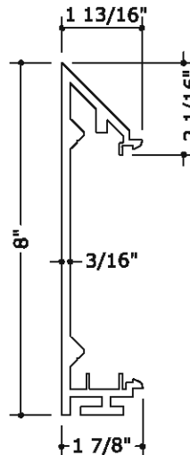
75 90° CORNER MULLION
