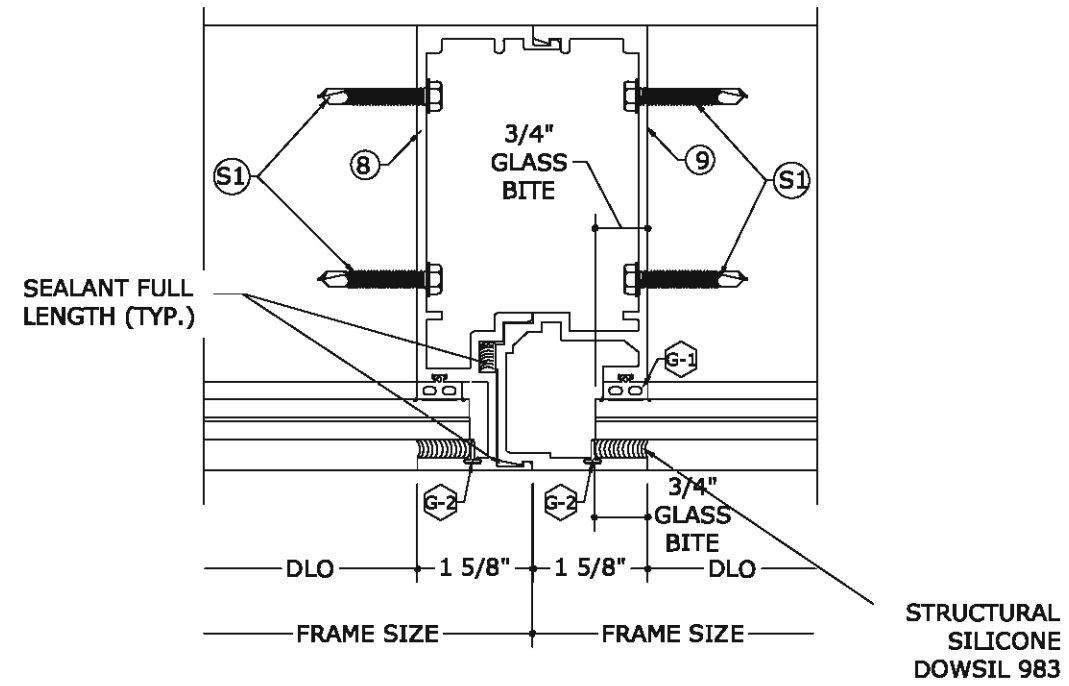
5 VERTICAL INTERMEDIATE DETAIL
