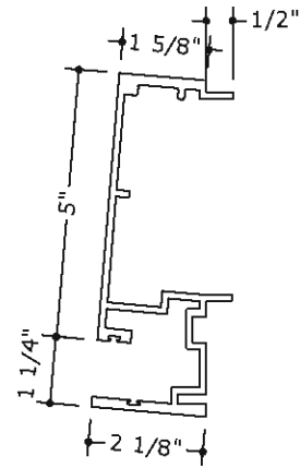
38 SEGMENTED MULLION
