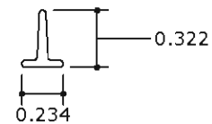
G-2 POLYETHYLENE GASKET
