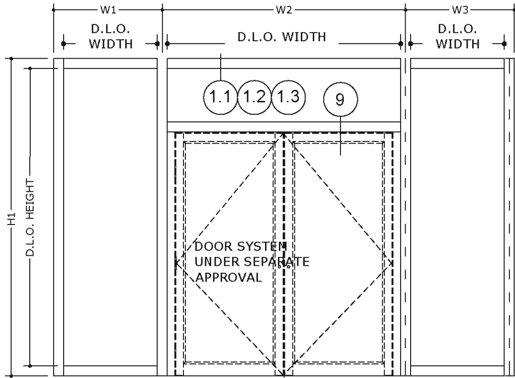
DOUBLE OR SINGLE DOOR
