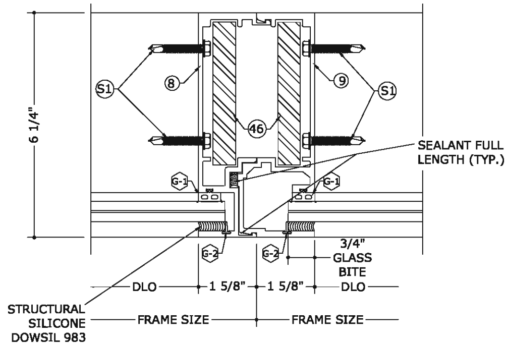
4 VERTICAL INTERMEDIATE DETAIL (REINFORCED)
