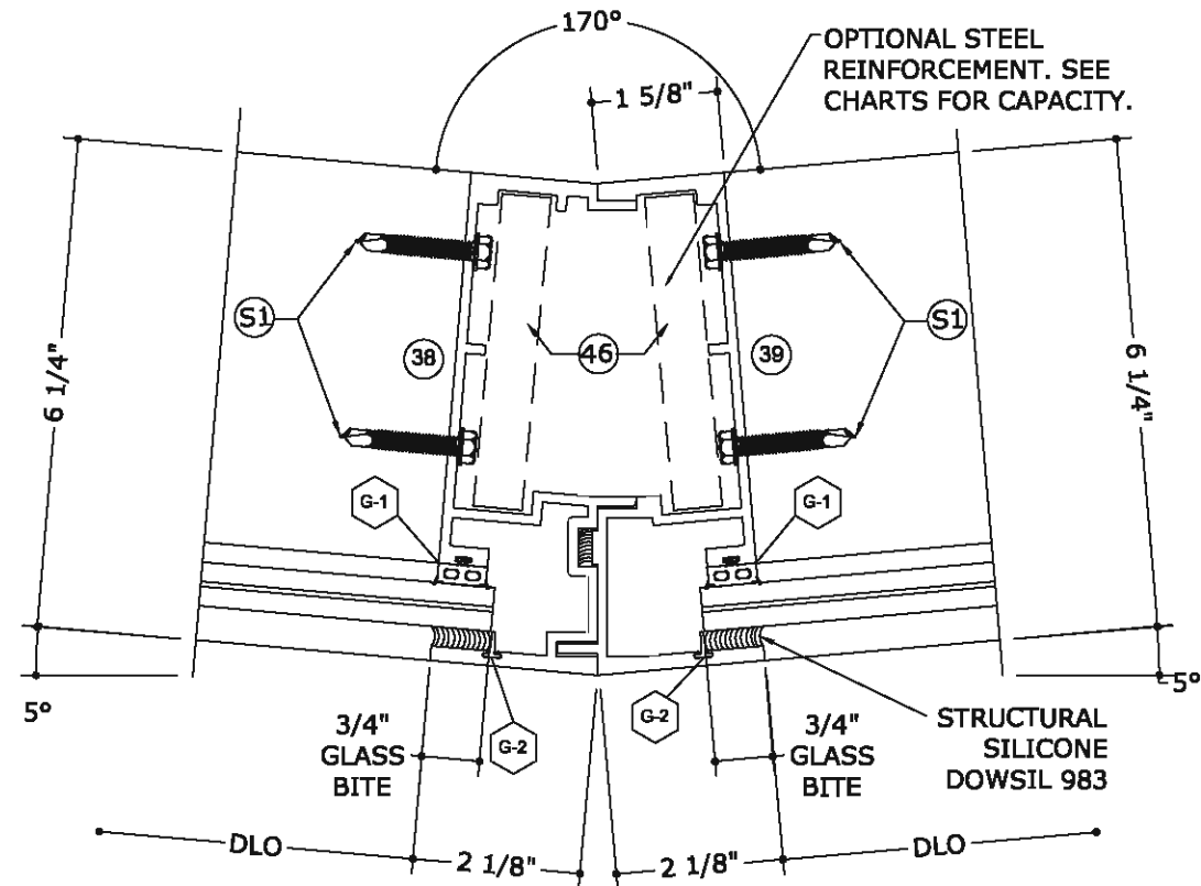
7 VERTICAL INTERMEDIATE DETAIL SEGMENTED 170 DEGREE MULLION
