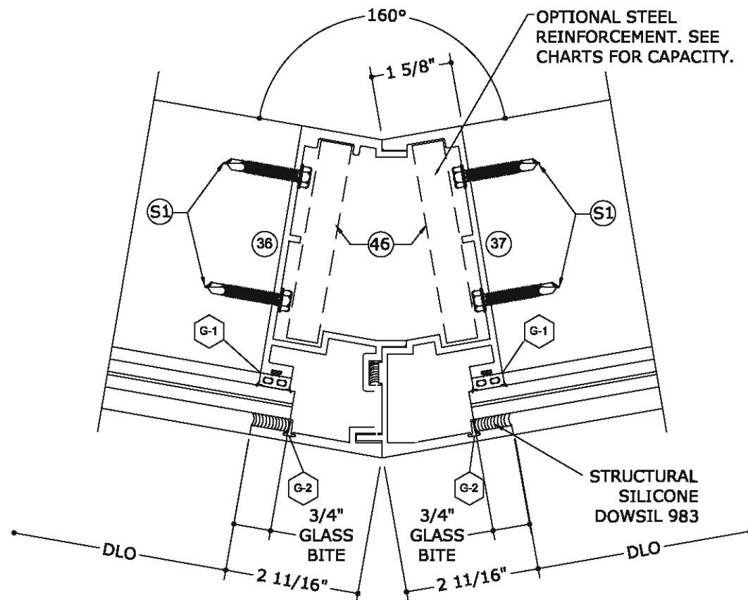
6 VERTICAL INTERMEDIATE DETAIL SEGMENTED 160 DEGREE MULLION
