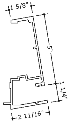
37 SEGMENTED MULLION
