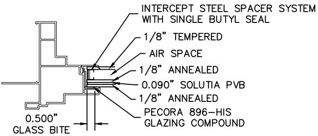
7/8" INSULATED TEMPERED/ANNEALED IMPACT GLASS WITH 0.090" PVB INTERLAYER
