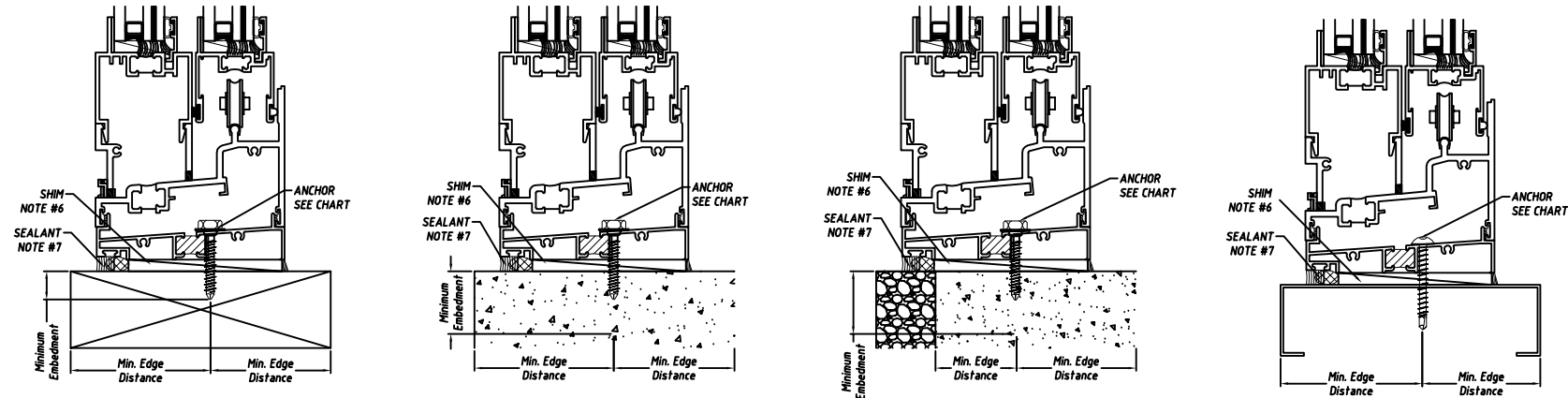
SILL
