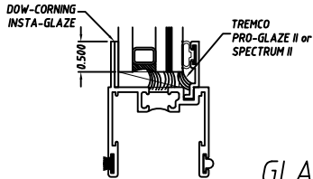
GLAZING
